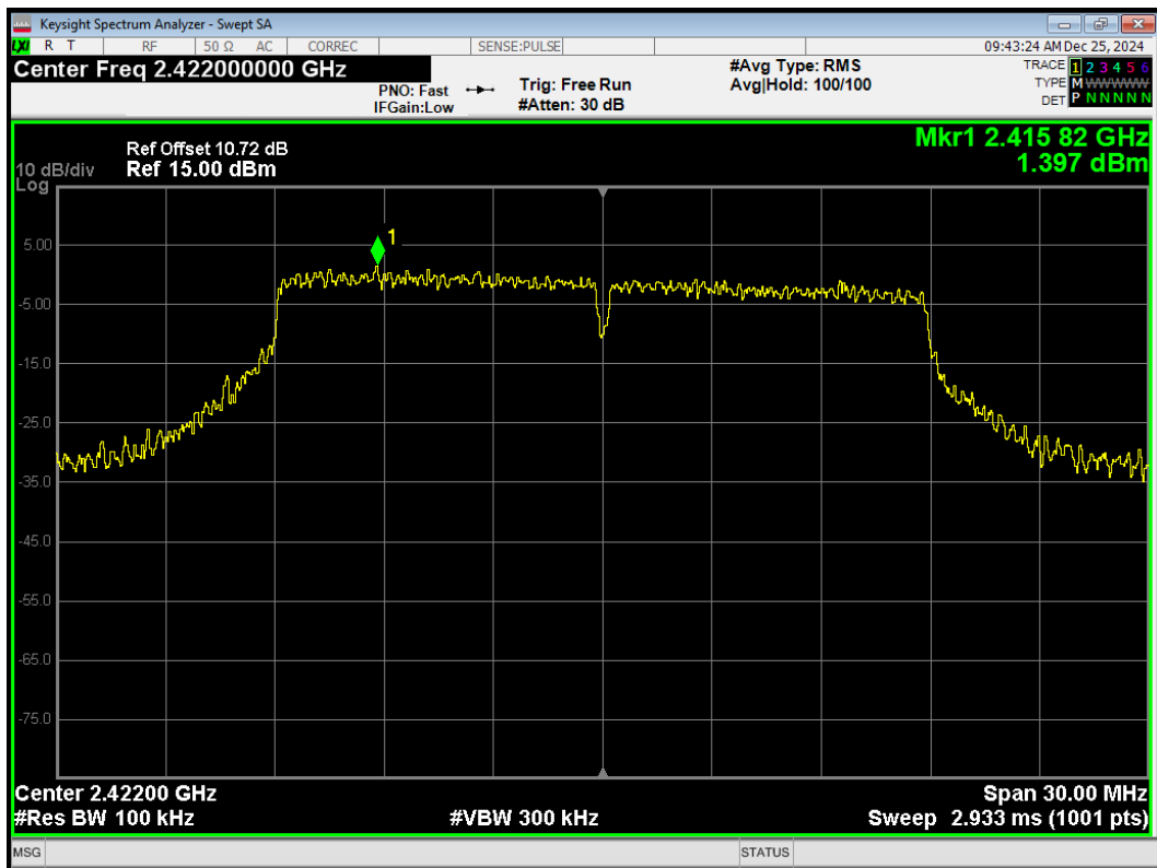
Tx. Spurious 802.11n(HT20) 2422MHz Emission
