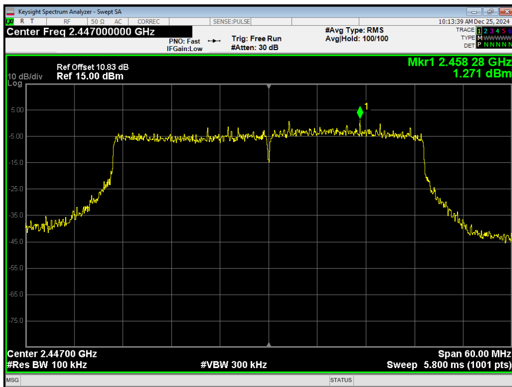
Tx. Spurious 802.11ax(HE40) 2447MHz Emission
