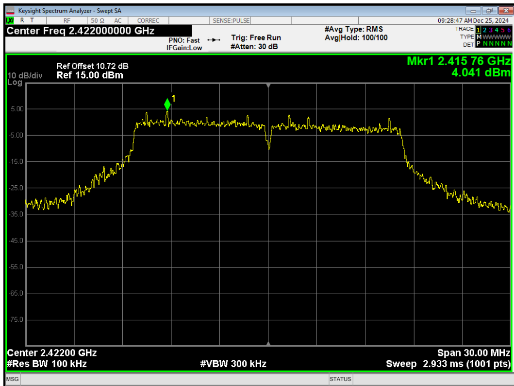
Tx. Spurious 802.11g 2422MHz Emission
