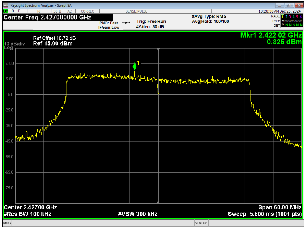
Tx. Spurious 802.11be(40) 2427MHz Emission
