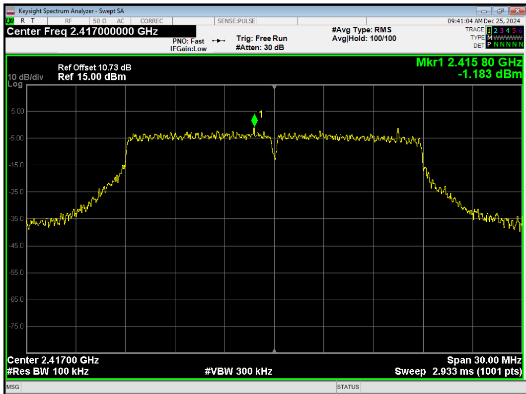
Tx. Spurious 802.11n(HT20) 2417MHz Emission
