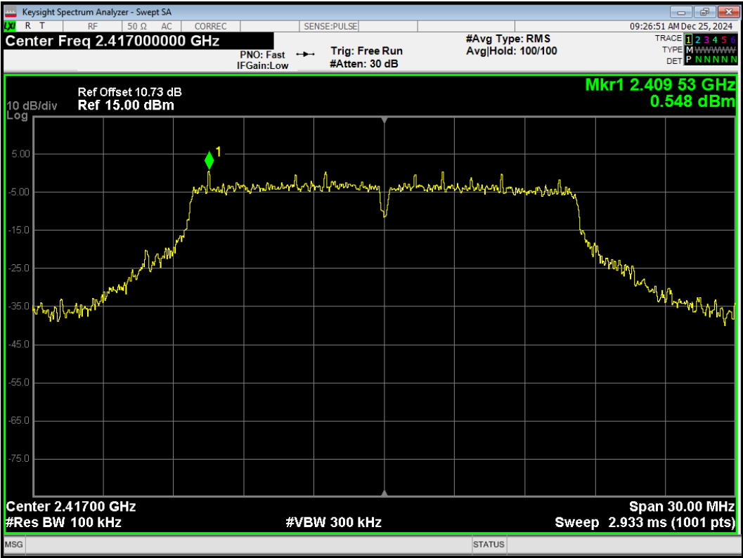
Tx. Spurious 802.11g 2417MHz Emission
