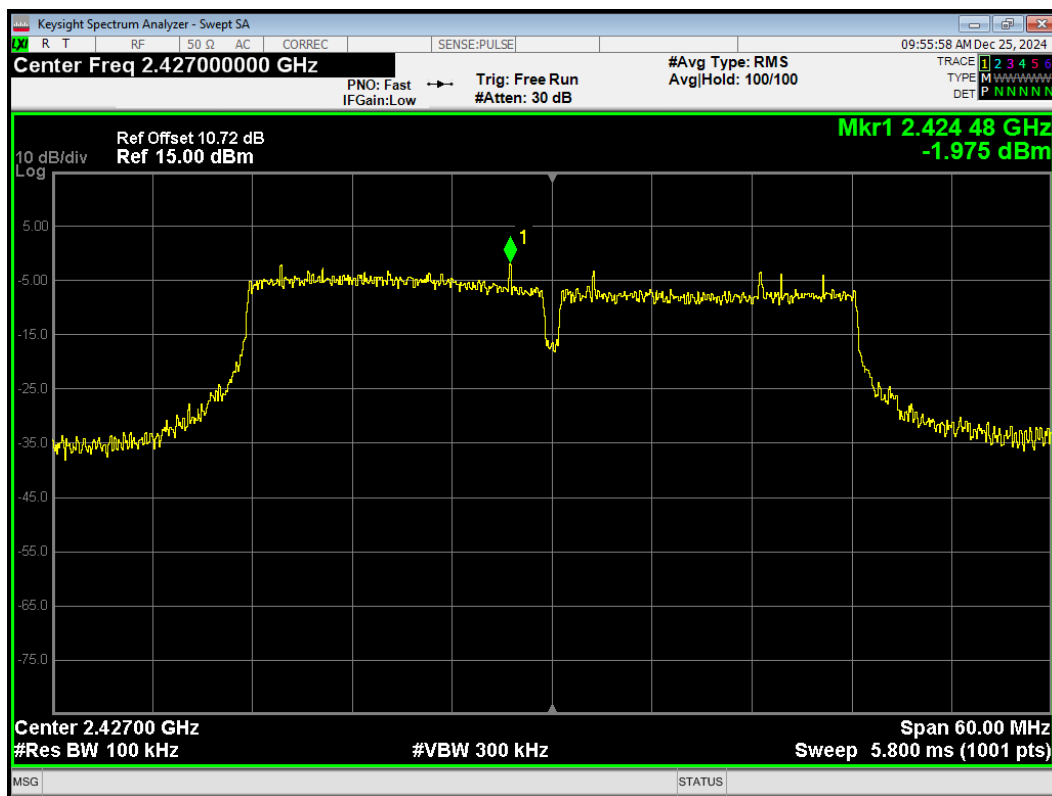
Tx. Spurious 802.11n(HT40) 2427MHz Emission
