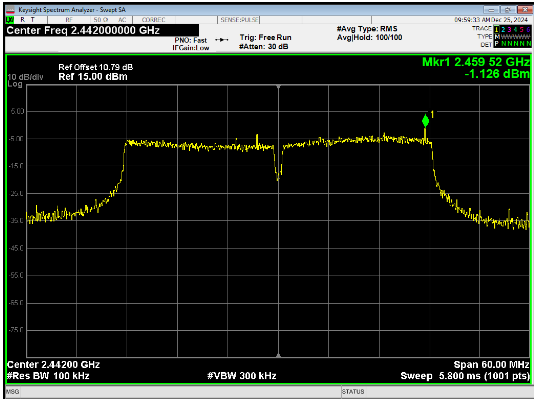
Tx. Spurious 802.11n(HT40) 2442MHz Emission
