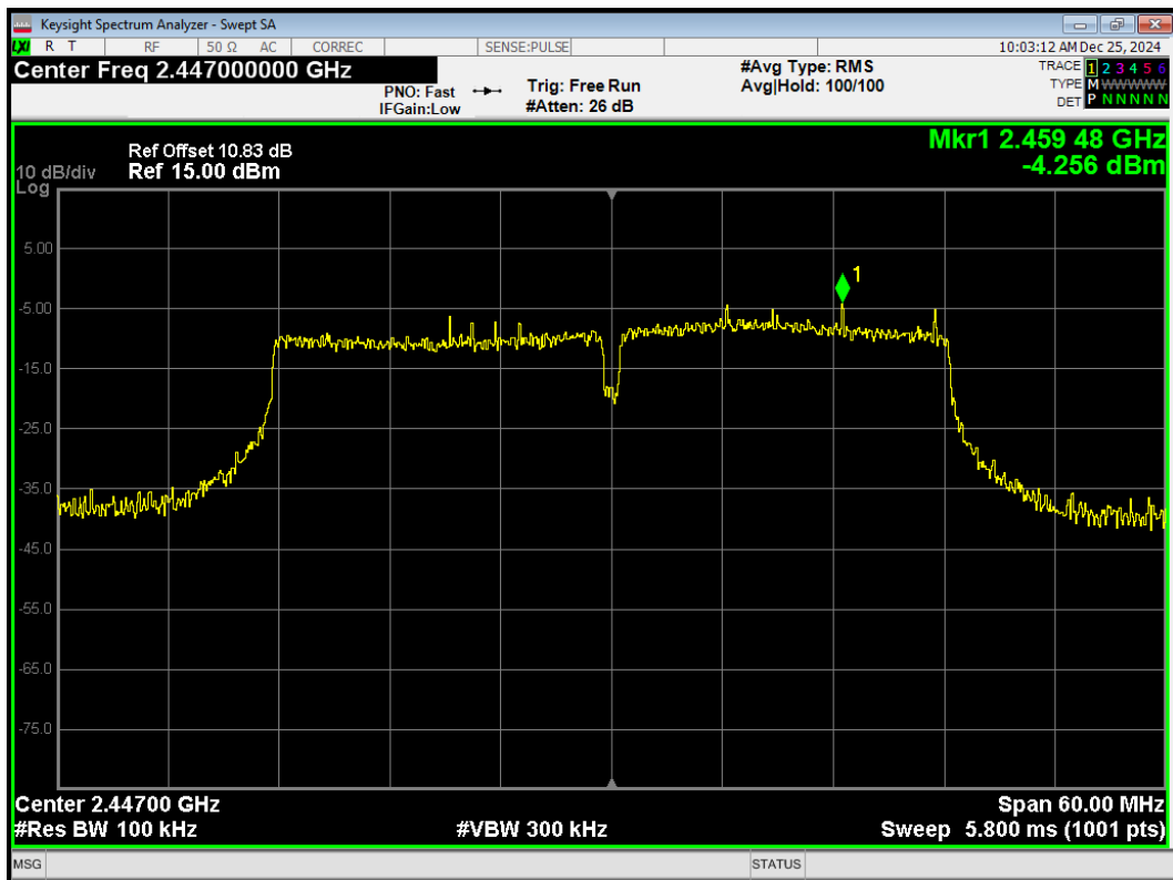
Tx. Spurious 802.11n(HT40) 2447MHz Emission
