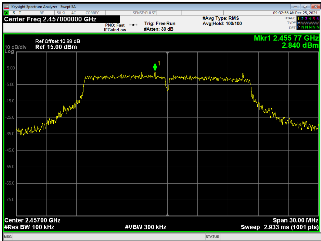
Tx. Spurious 802.11g 2457MHz Emission
