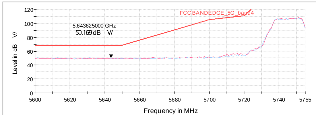
Wi-Fi 5GHz_a CH149
