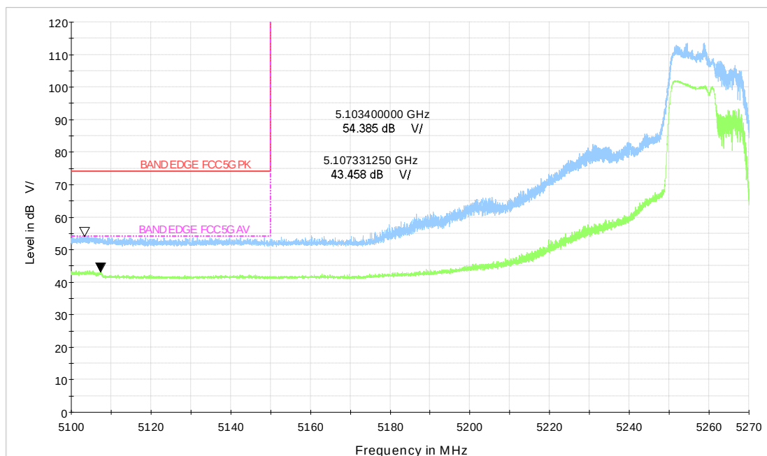
Wi-Fi 5GHz_BE20 106+26Tone LOW_CH52
