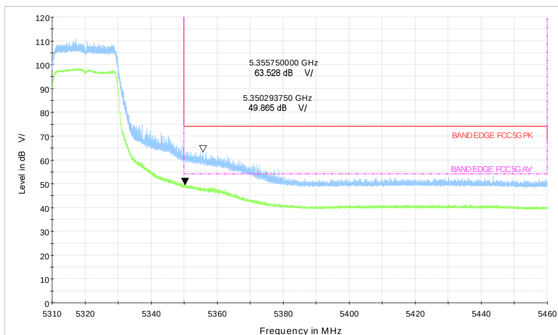
Wi-Fi 5GHz_ax20 CH64
