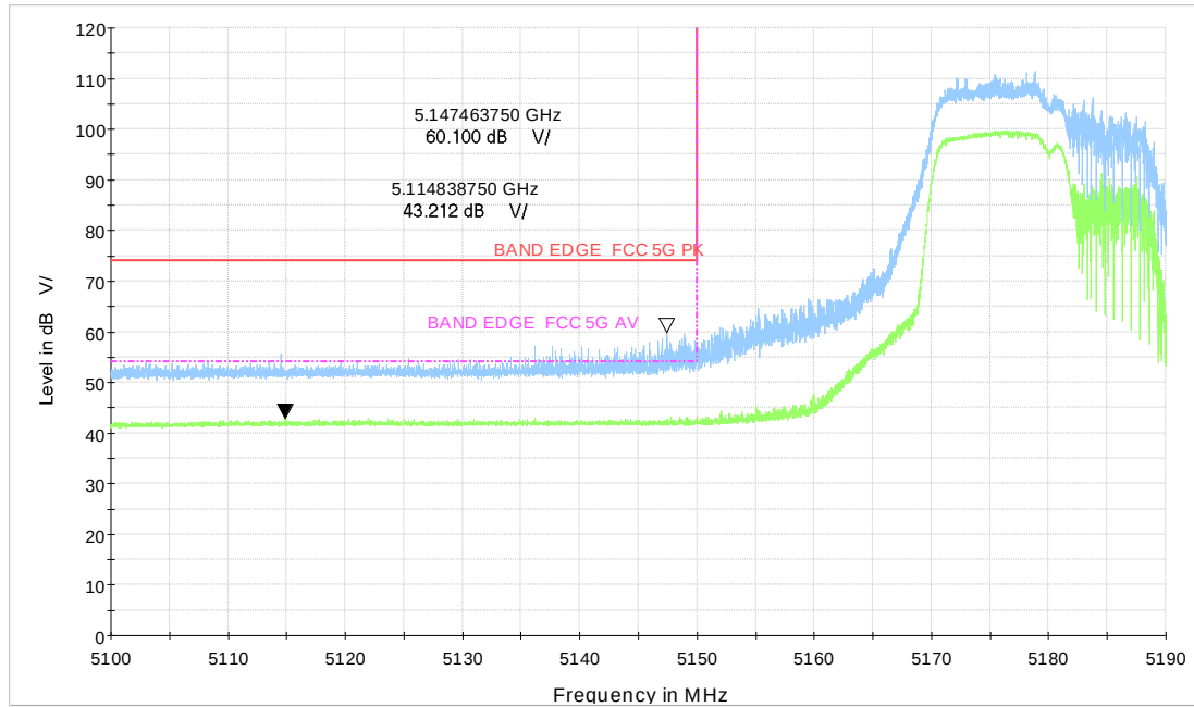
Wi-Fi 5GHz_BE20 106+26Tone LOW_CH36
