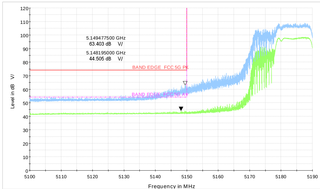
Wi-Fi 5GHz_BE20 106+26Tone HIGH_CH36
