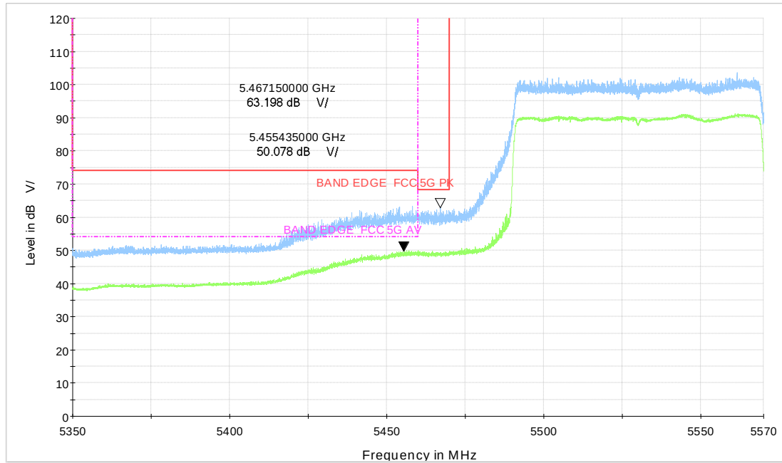
Wi-Fi 5GHz TB_BE80 CH106_996Tone
