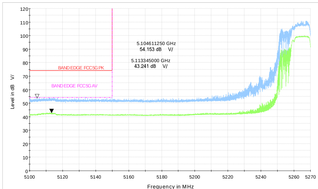
Wi-Fi 5GHz_BE20 106+26Tone HIGH_CH52
