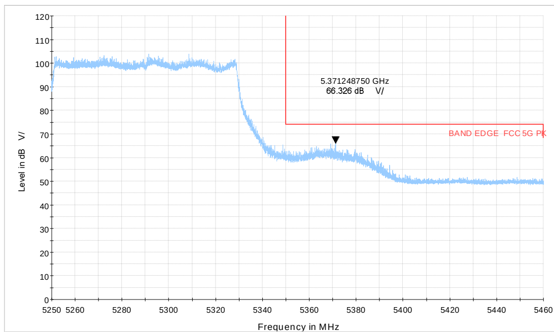
Wi-Fi 5GHz TB_BE80 CH58_996Tone
