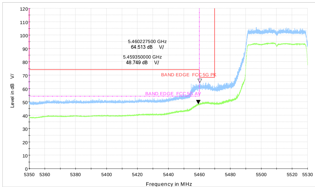
Wi-Fi 5GHz TB_ax40 CH102_484Tone
