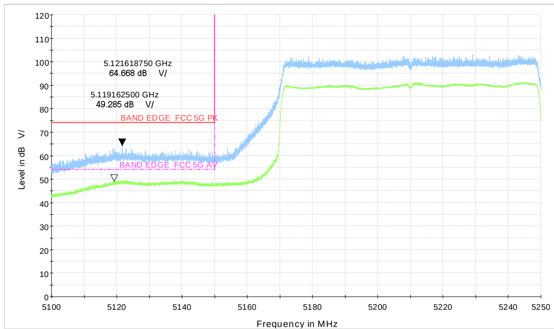
Wi-Fi 5GHz TB_ax80 CH42_996Tone
