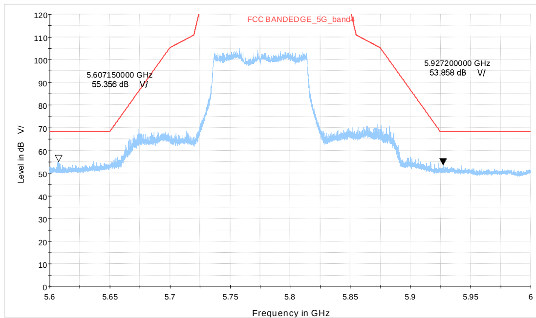
Wi-Fi 5GHz TB_BE80 CH155_996Tone
