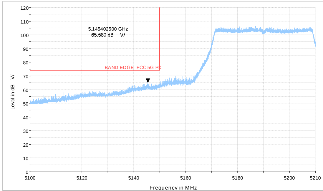
Wi-Fi 5GHz TB_BE40 CH38_484Tone
