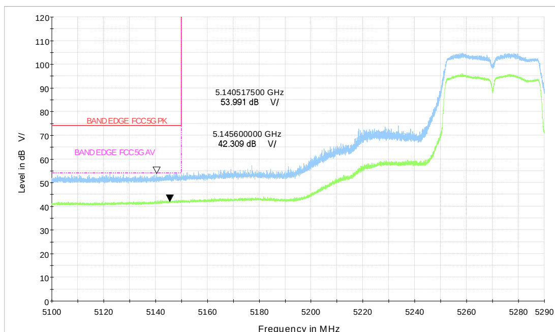
Wi-Fi 5GHz_n40 CH54
