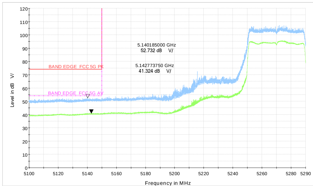
Wi-Fi 5GHz TB_BE40 CH54_484Tone
