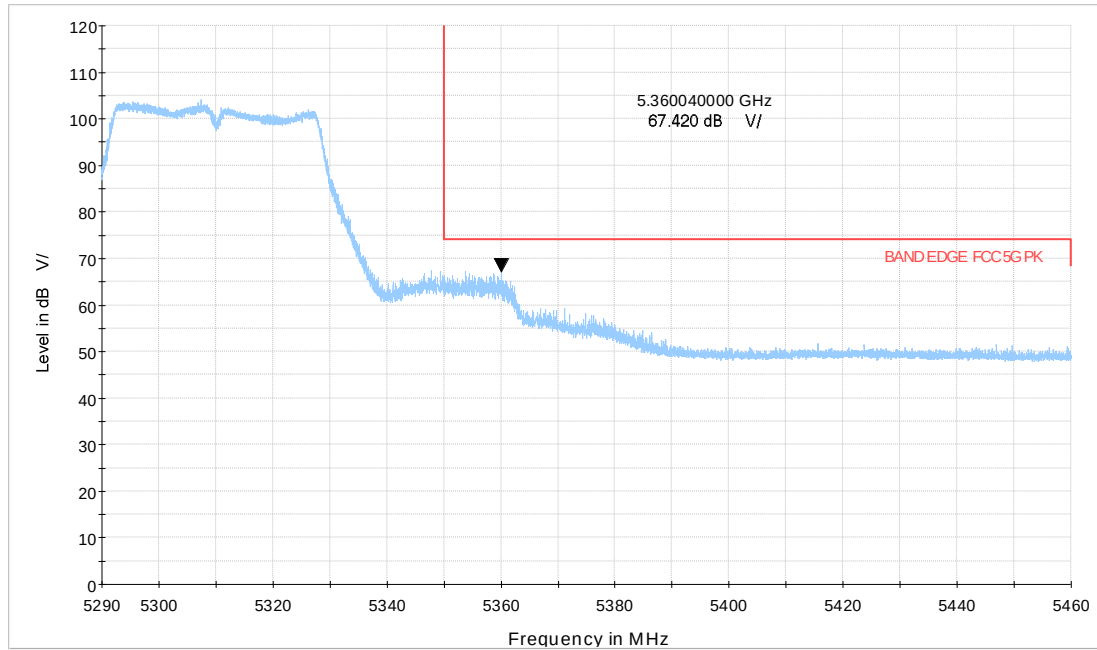
Wi-Fi 5GHz_n40 CH62
