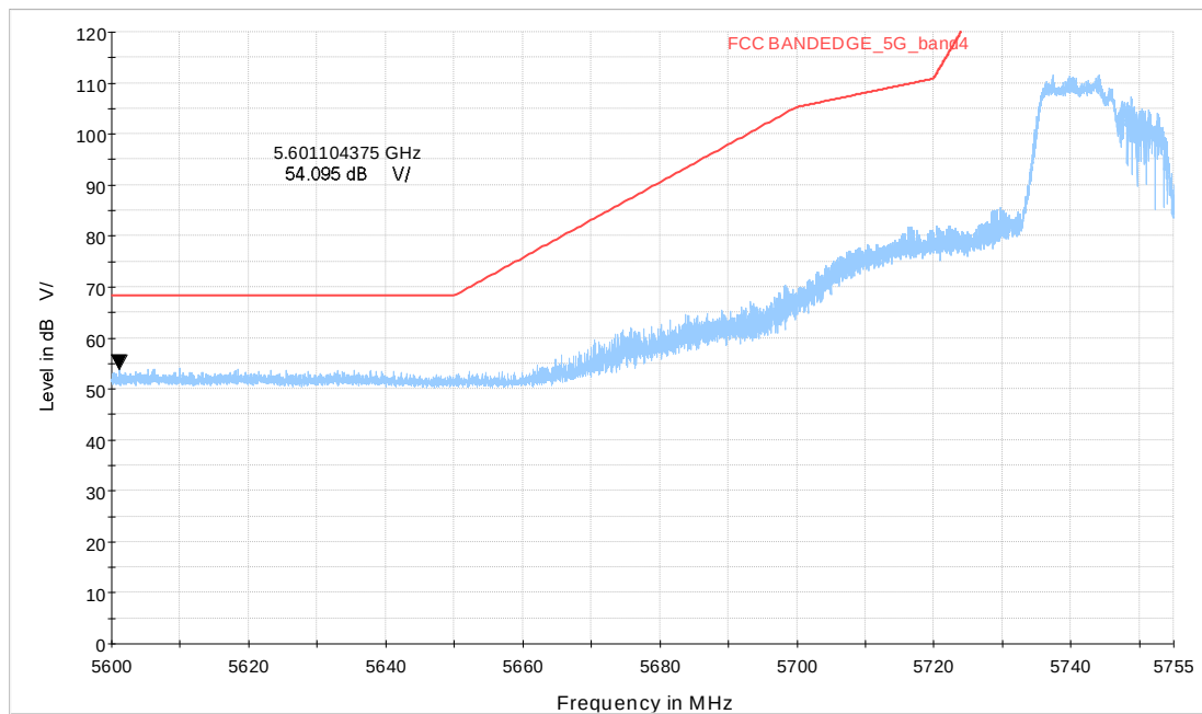
Wi-Fi 5GHz_BE20 106+26Tone LOW_CH149
