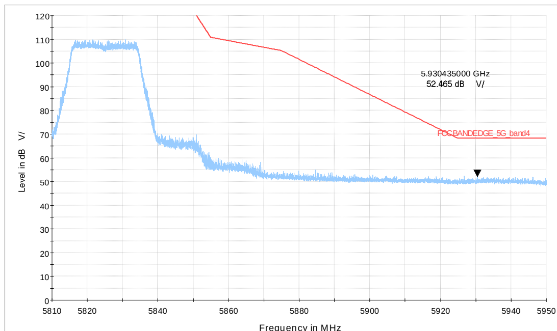
Wi-Fi 5GHz_BE20 CH165
