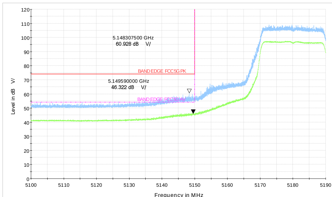
Wi-Fi 5GHz_BE20 CH36
