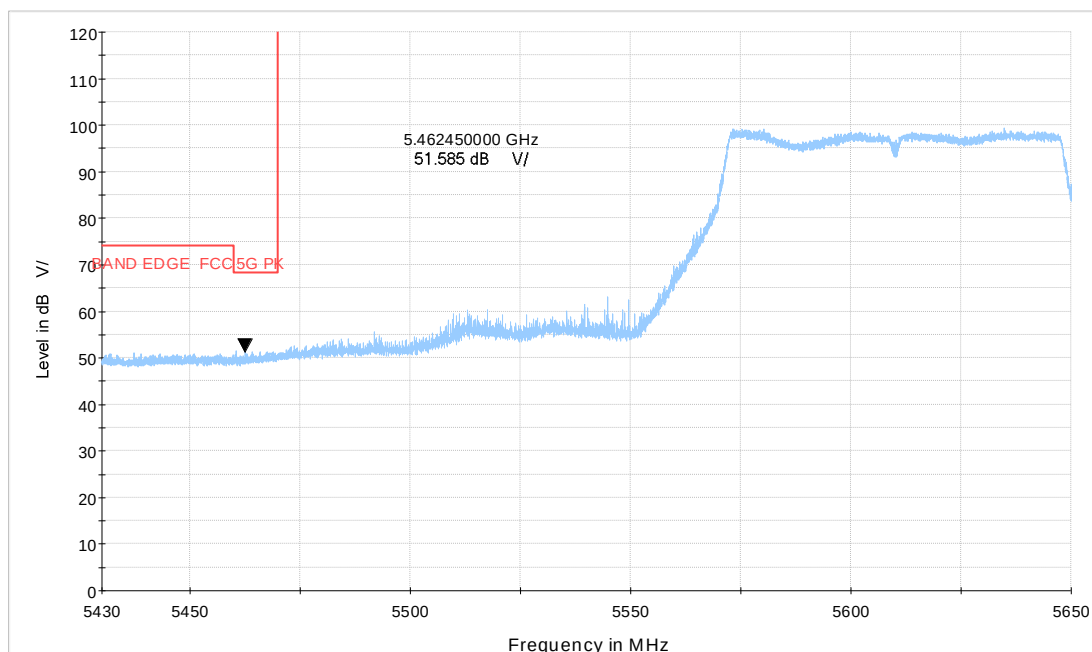
Wi-Fi 5GHz_ac80 CH122
