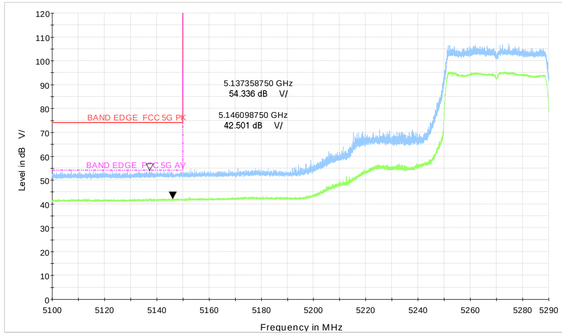
Wi-Fi 5GHz TB_ax40 CH54_484Tone
