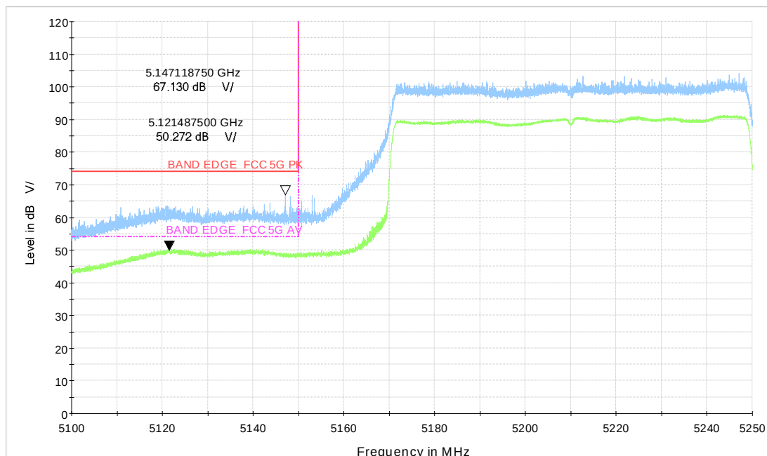
Wi-Fi 5GHz TB_BE80 CH42_996Tone
