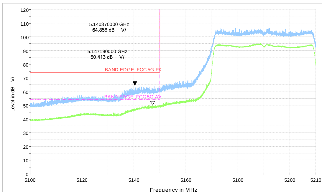
Wi-Fi 5GHz_BE40 CH38
