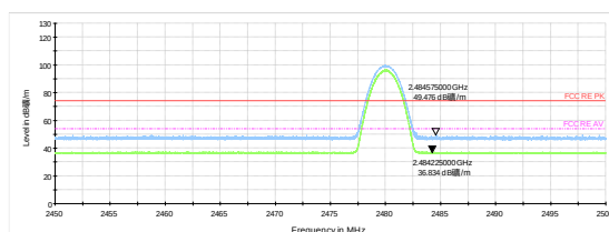
3DH5-Channel 78: Peak + Average
