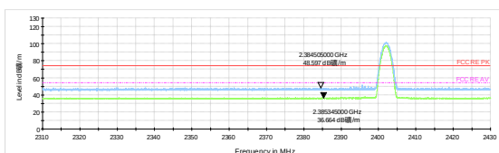
3DH5-Channel 0: Peak + Average
