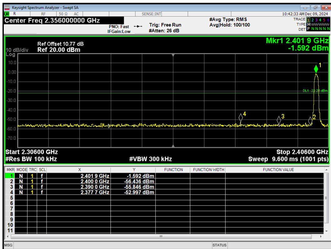
Band Edge 2-DH5 2402MHz No-Hopping Emission
