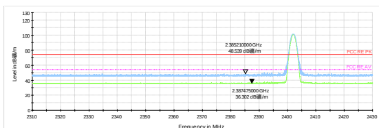
DH5-Channel 0: Peak + Average
