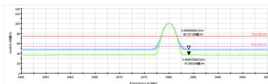
DH5-Channel 78: Peak + Average
