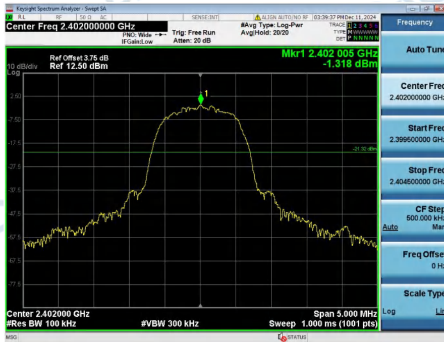
2_Spurious_Emissions_NVNT_ANT1_3-DH5_2402_00
