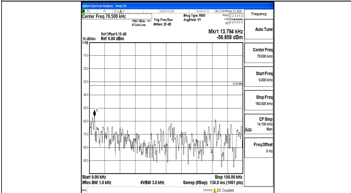
Band26_5MHz_QPSK_26765_1RB#0_0.009~0.15_0.009~0.15
