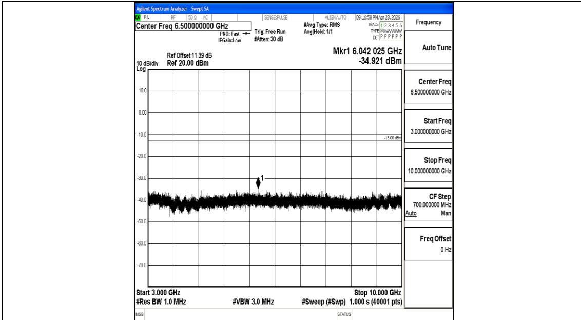
Band26_5MHz_16QAM_26740_1RB#0_3000~10000_3000~10000
