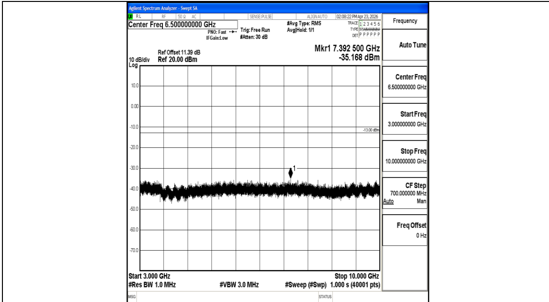
Band26_1.4MHz_16QAM_26783_1RB#0_3000~10000_3000~10000
