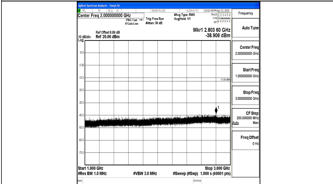
Band26_10MHz_16QAM_26740_1RB#0_1000~3000_1000~3000
