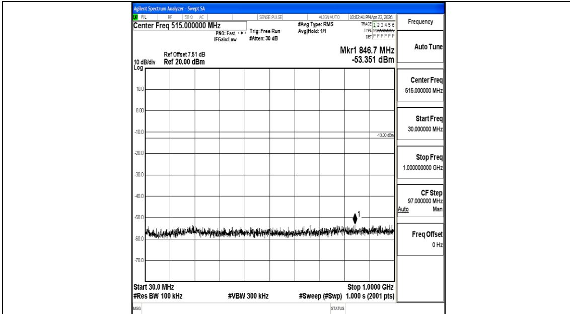
Band26_10MHz_16QAM_26740_1RB#0_30~1000_30~1000
