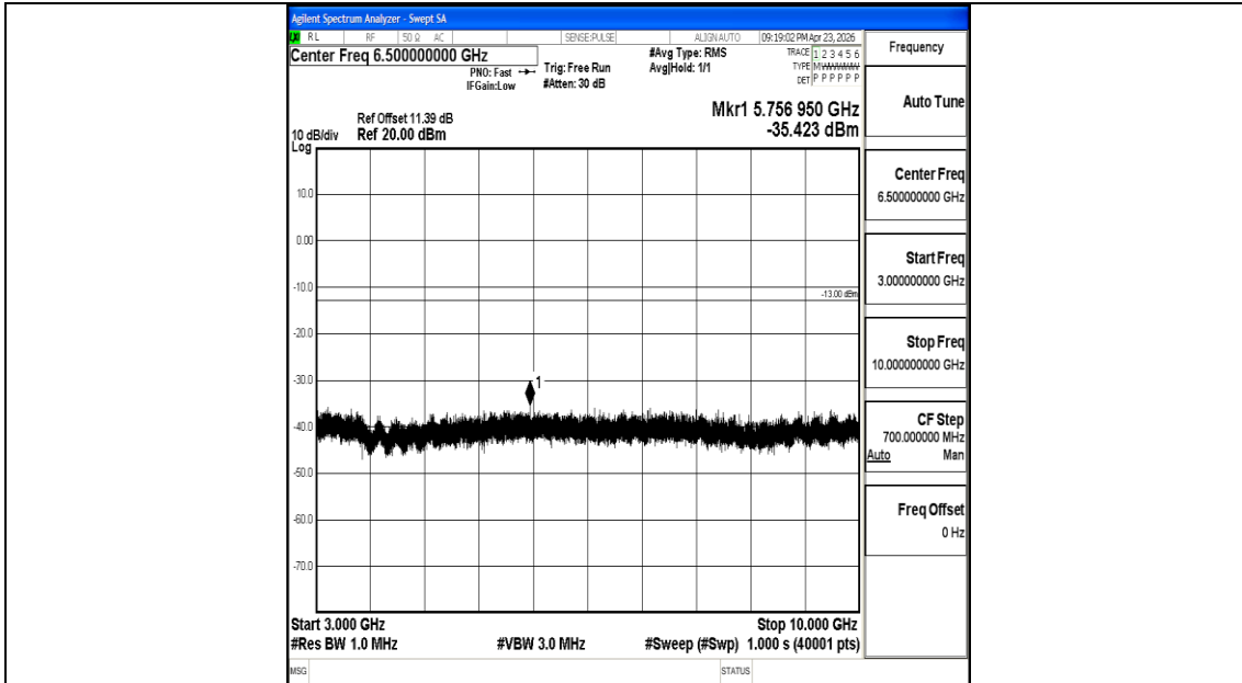
Band26_5MHz_16QAM_26765_1RB#0_3000~10000_3000~10000
