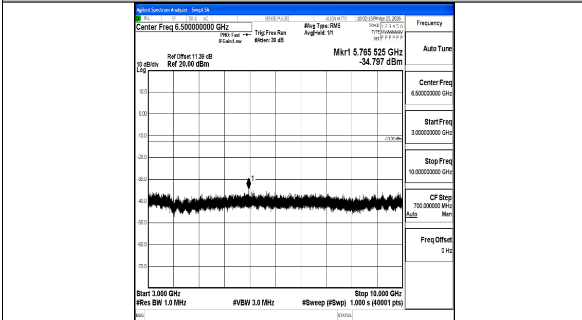
Band26_10MHz_QPSK_26740_1RB#0_3000~10000_3000~10000
