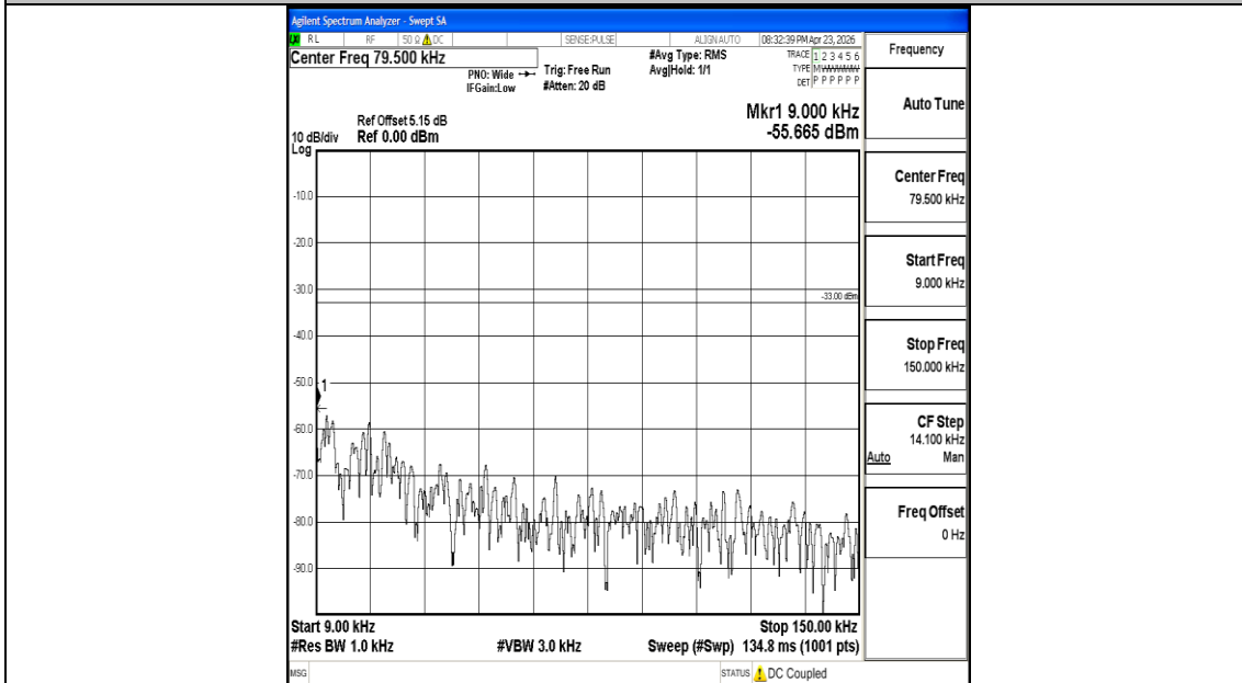
Band26_3MHz_QPSK_26705_1RB#0_0.009~0.15_0.009~0.15
