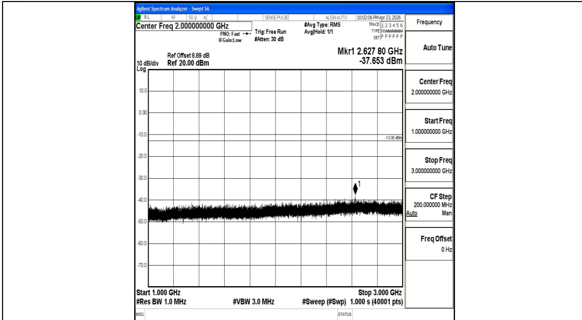
Band26_10MHz_QPSK_26740_1RB#0_1000~3000_1000~3000
