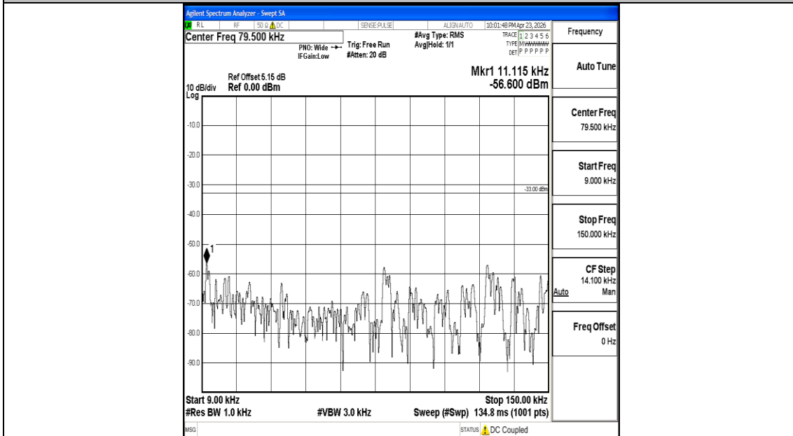
Band26_10MHz_QPSK_26740_1RB#0_0.009~0.15_0.009~0.15
