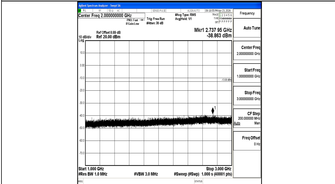
Band26_5MHz_16QAM_26765_1RB#0_1000~3000_1000~3000
