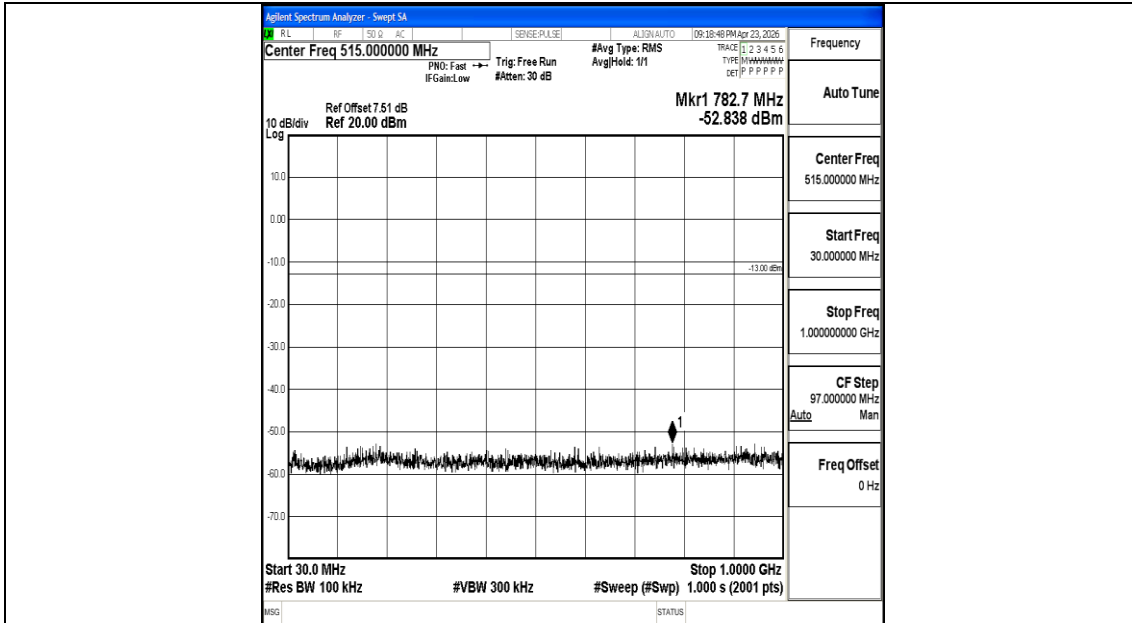
Band26_5MHz_16QAM_26765_1RB#0_30~1000_30~1000
