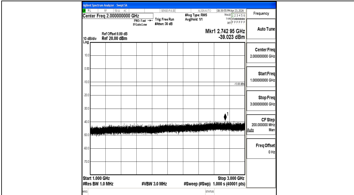
Band26_3MHz_QPSK_26775_1RB#0_1000~3000_1000~3000
