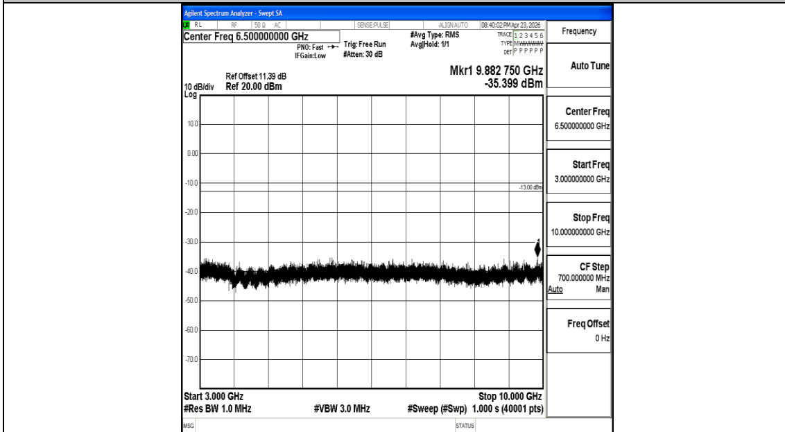
Band26_3MHz_QPSK_26775_1RB#0_3000~10000_3000~10000
