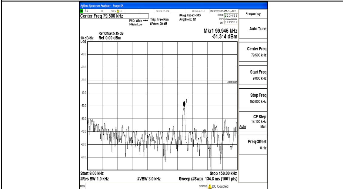
Band26_5MHz_QPSK_26740_1RB#0_0.009~0.15_0.009~0.15
