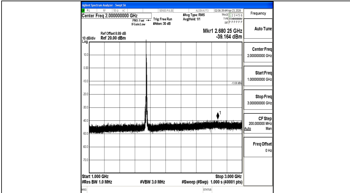
Band4_10MHz_QPSK_20350_1RB#0_1000~3000_1000~3000
