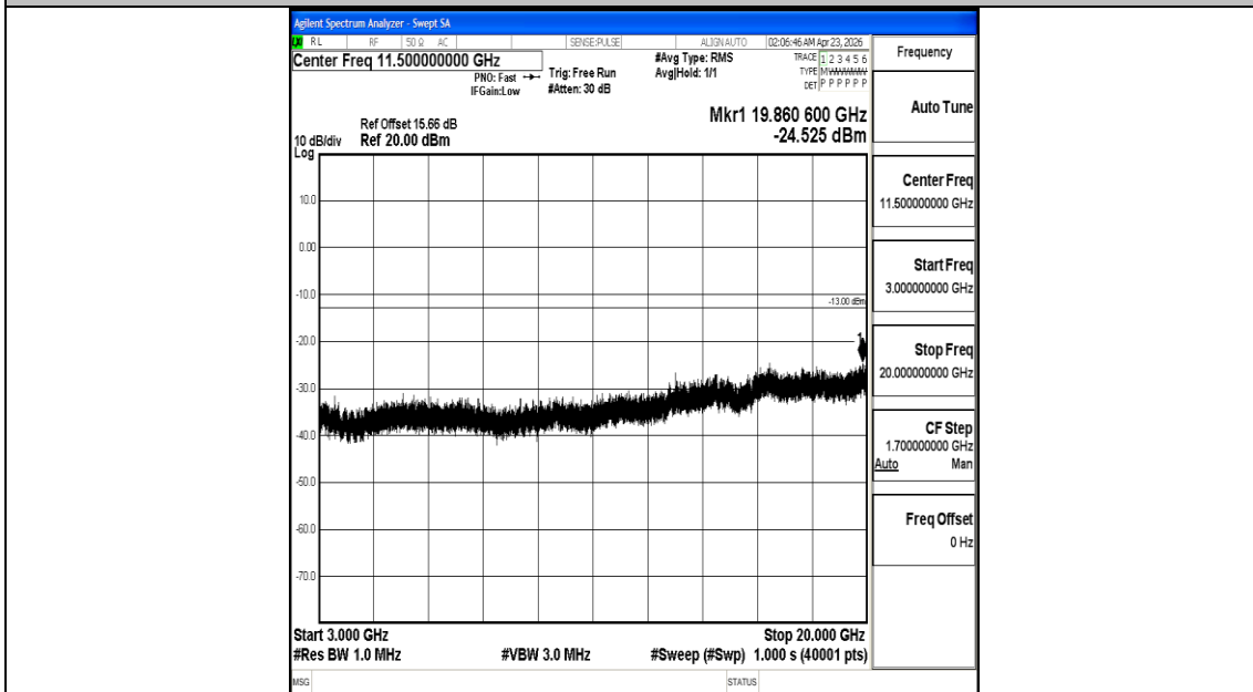
Band4_10MHz_QPSK_20350_1RB#0_3000~20000_3000~20000
