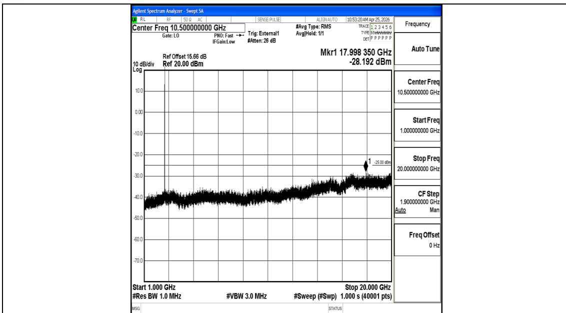
Band41_10MHz_16QAM_40620_1RB#0_1000~20000_1000~20000
