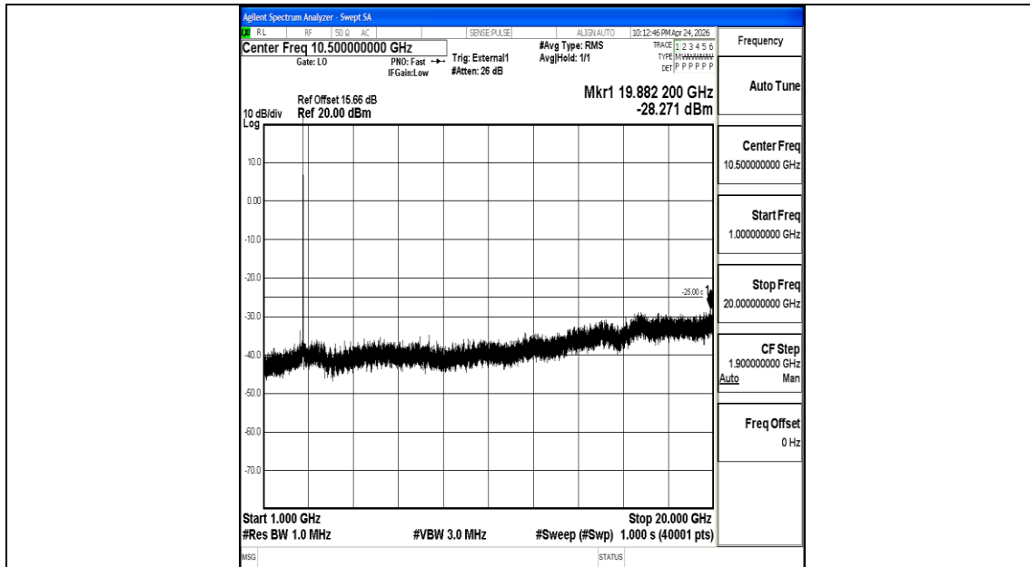
Band41_15MHz_16QAM_41515_1RB#0_1000~20000_1000~20000
