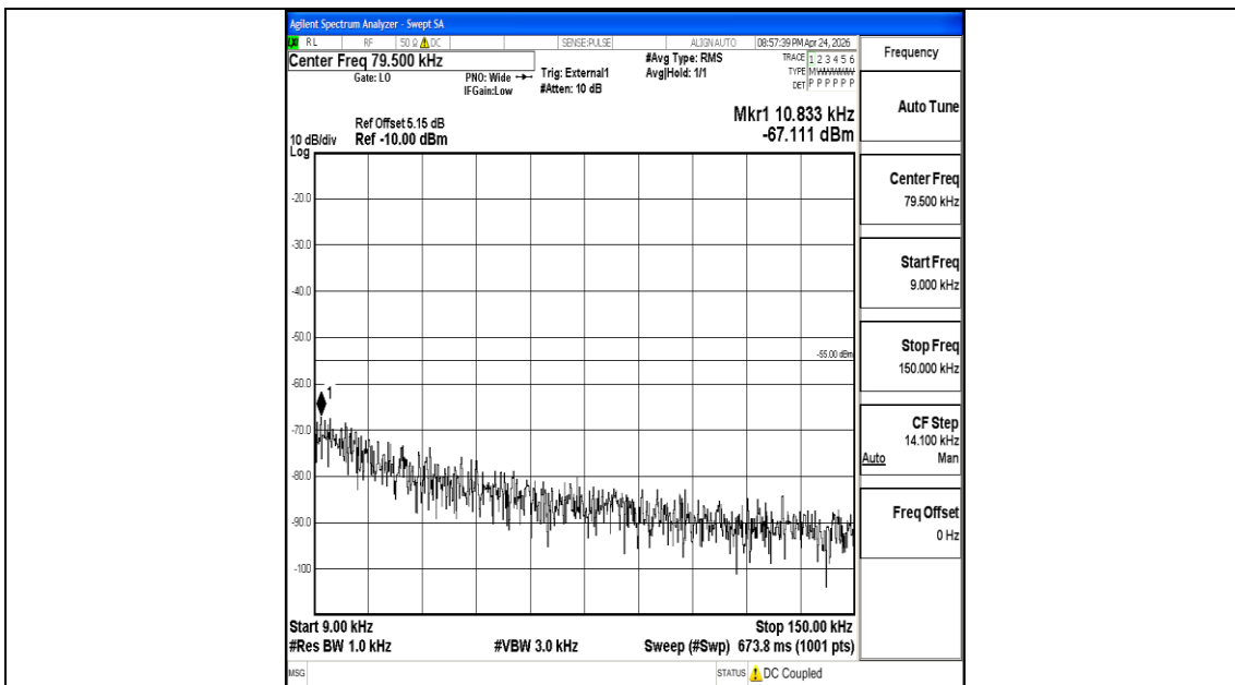
Band41_5MHz_QPSK_41565_1RB#0_0.009~0.15_0.009~0.15
