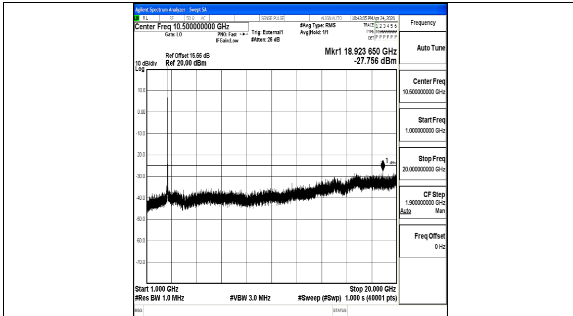
Band41_20MHz_16QAM_40620_1RB#0_1000~20000_1000~20000
