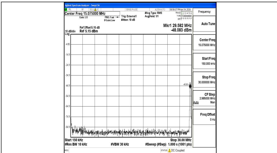
Band41_5MHz_16QAM_40620_1RB#0_0.15~30_0.15~30
