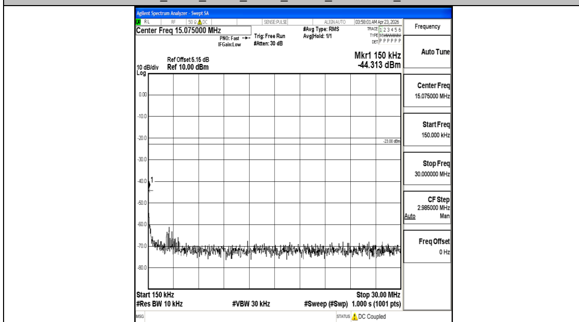
Band5_3MHz_QPSK_20635_1RB#0_0.15~30_0.15~30
