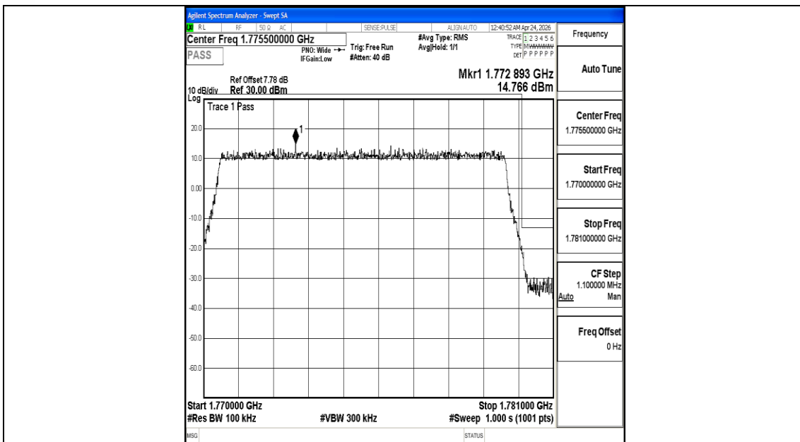
Band66_10MHz_QPSK_132622_50RB#0
