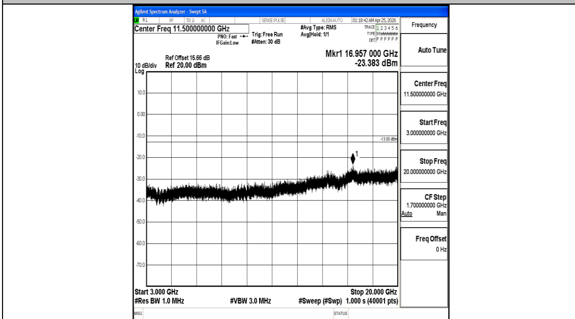
Band66_3MHz_QPSK_132322_1RB#0_3000~20000_3000~20000
