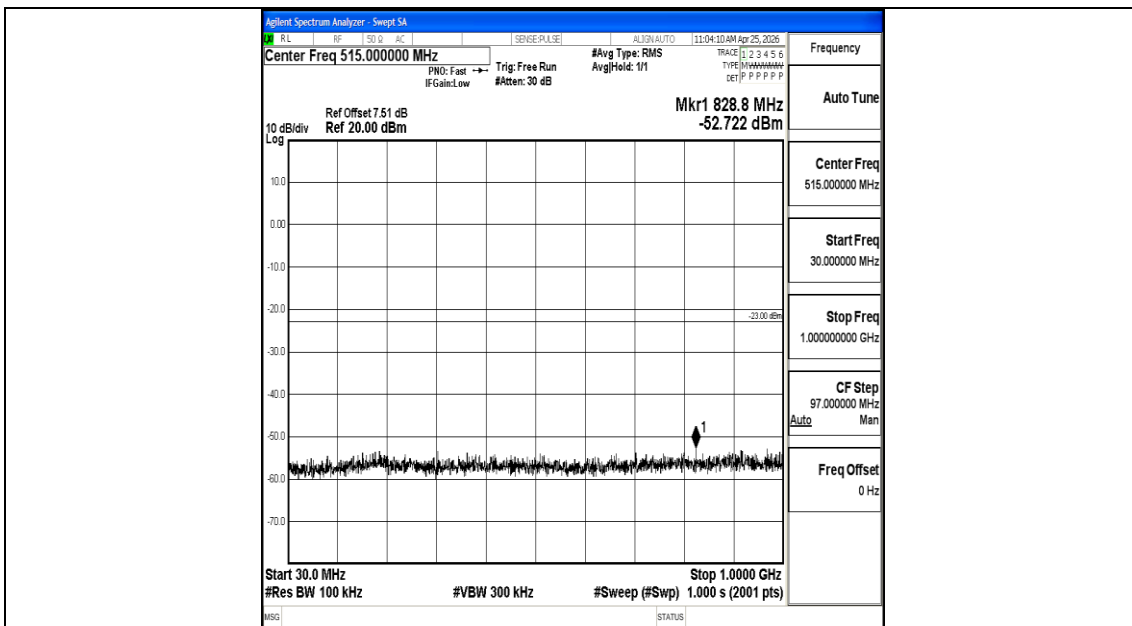
Band66_1.4MHz_16QAM_131979_1RB#0_30~1000_30~1000
