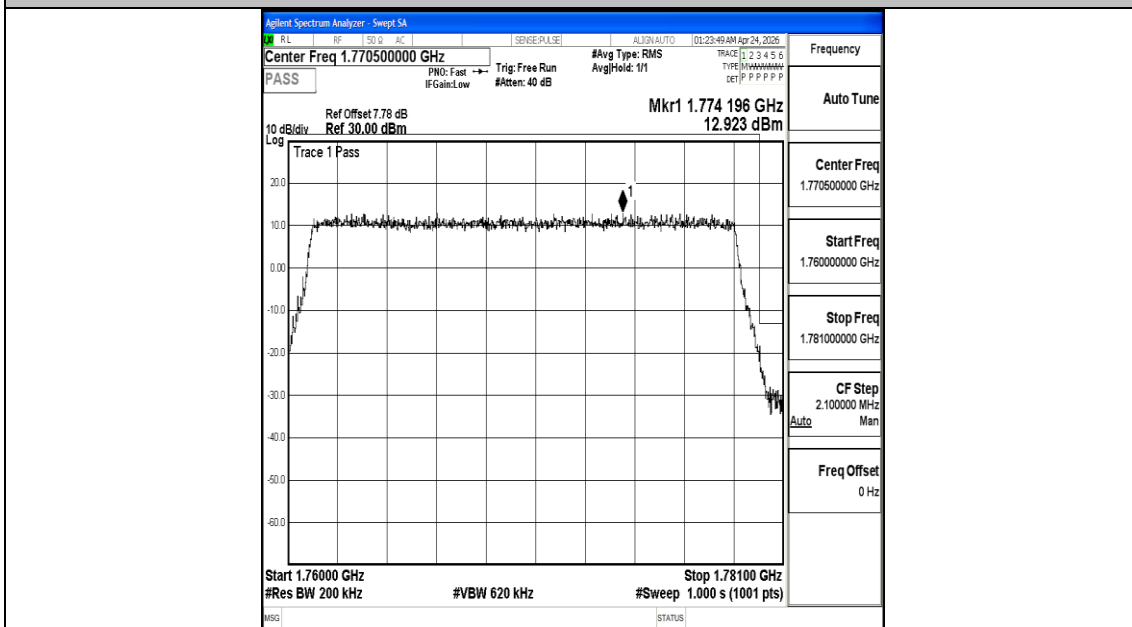
Band66_20MHz_16QAM_132572_100RB#0
