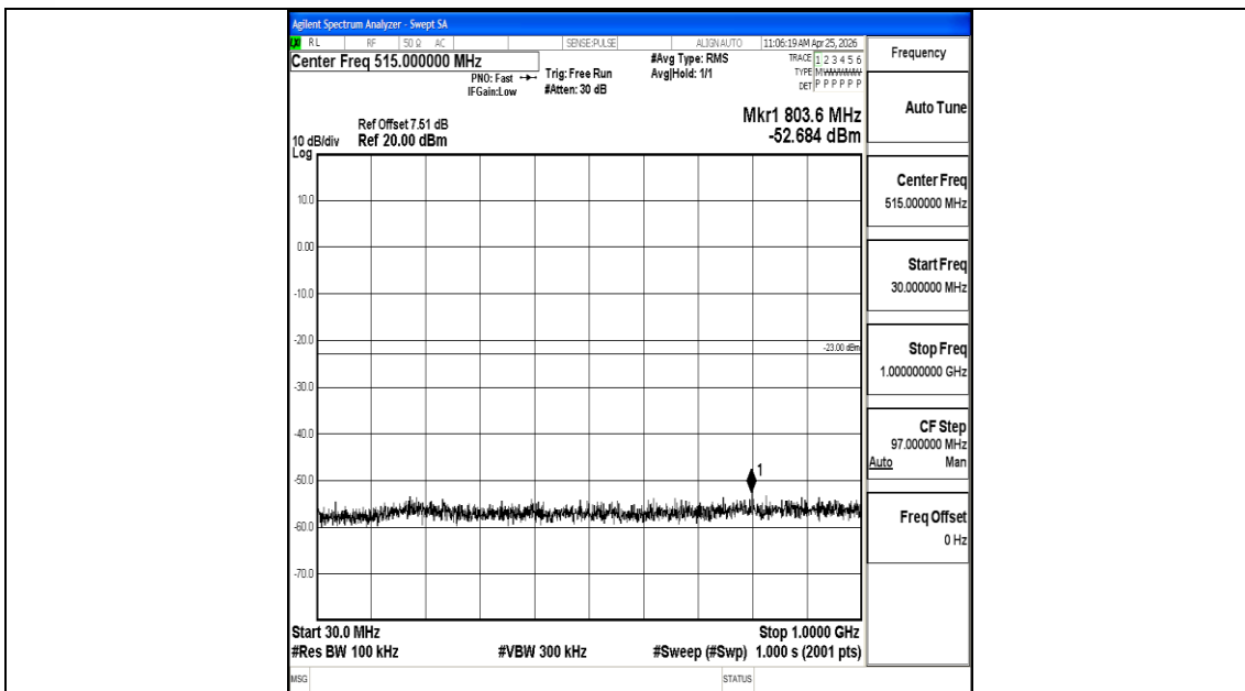
Band66_1.4MHz_16QAM_132665_1RB#0_30~1000_30~1000
