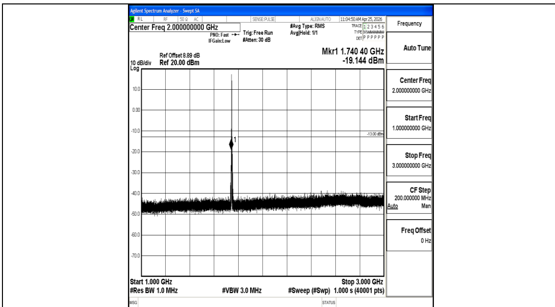
Band66_1.4MHz_QPSK_132322_1RB#0_1000~3000_1000~3000
