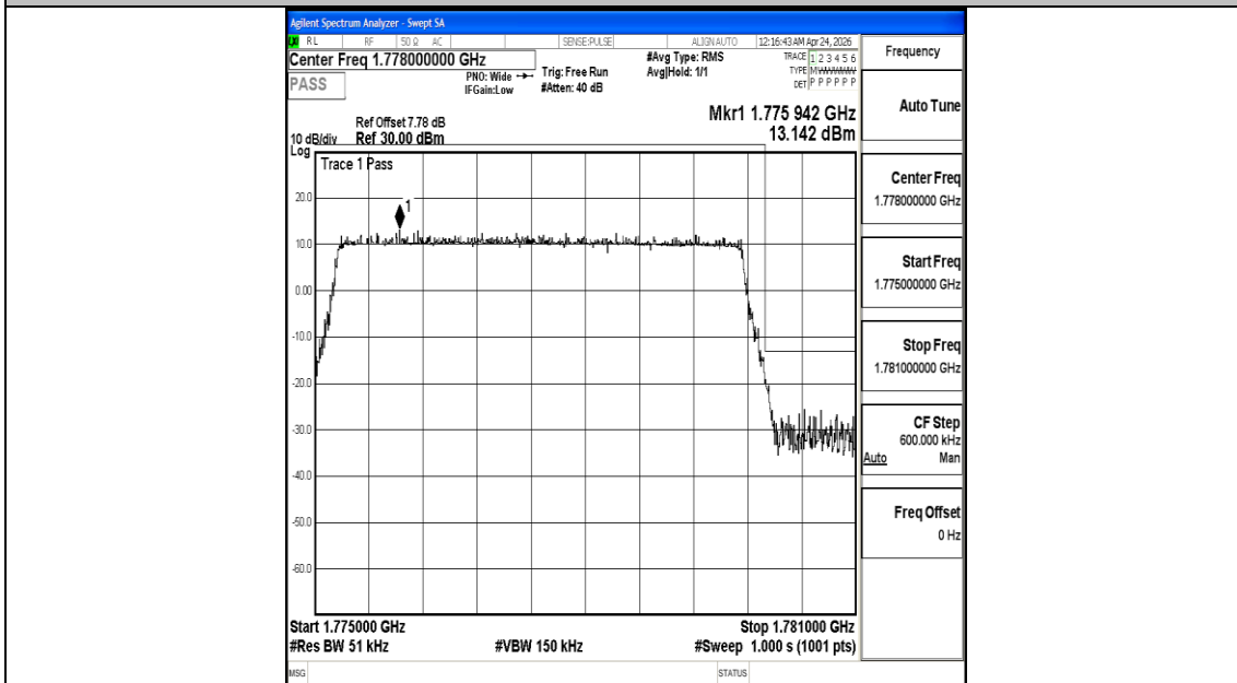
Band66_5MHz_16QAM_132647_25RB#0
