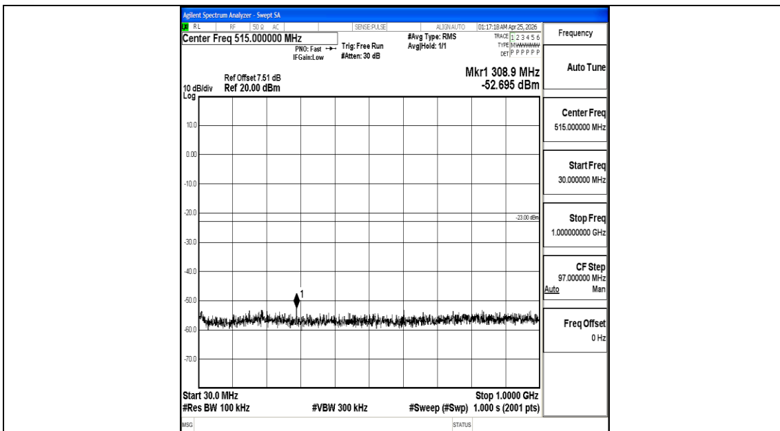
Band66_3MHz_QPSK_131987_1RB#0_30~1000_30~1000
