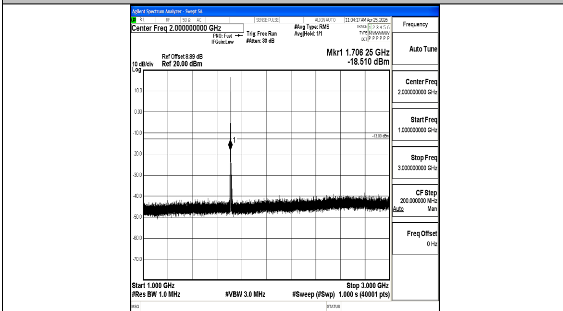
Band66_1.4MHz_16QAM_131979_1RB#0_1000~3000_1000~3000
