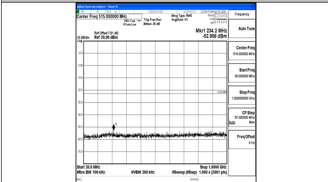
Band66_1.4MHz_QPSK_132665_1RB#0_30~1000_30~1000
