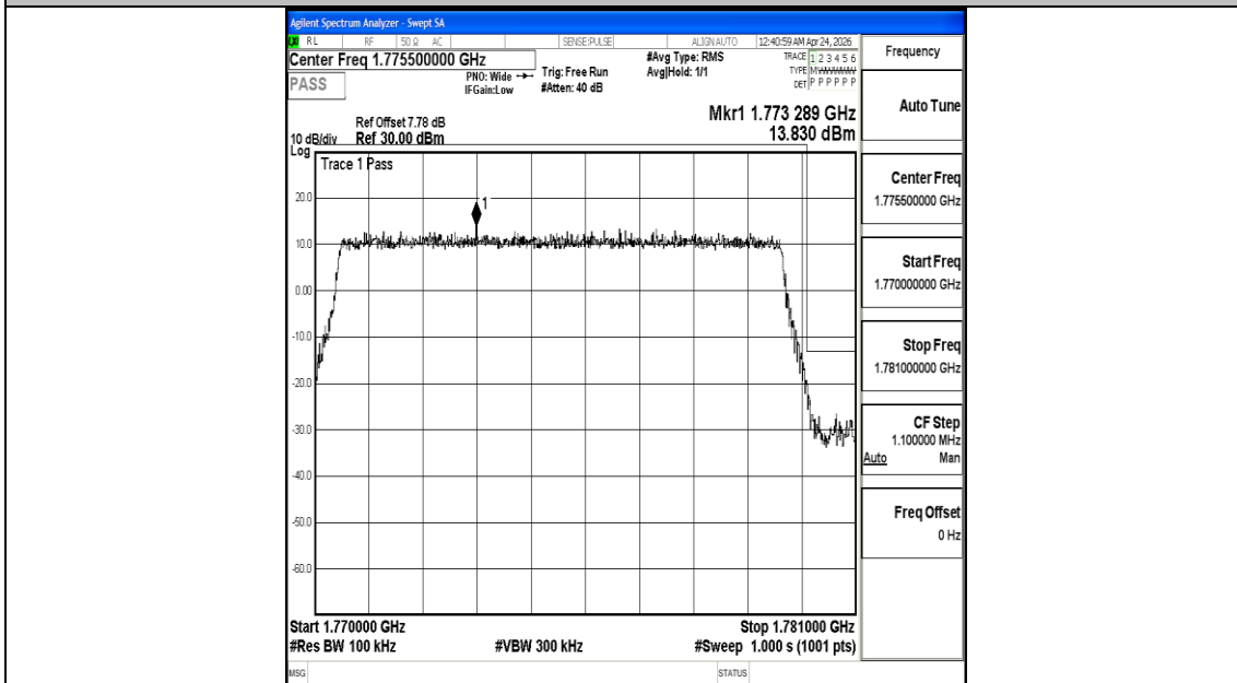
Band66_10MHz_16QAM_132622_50RB#0
