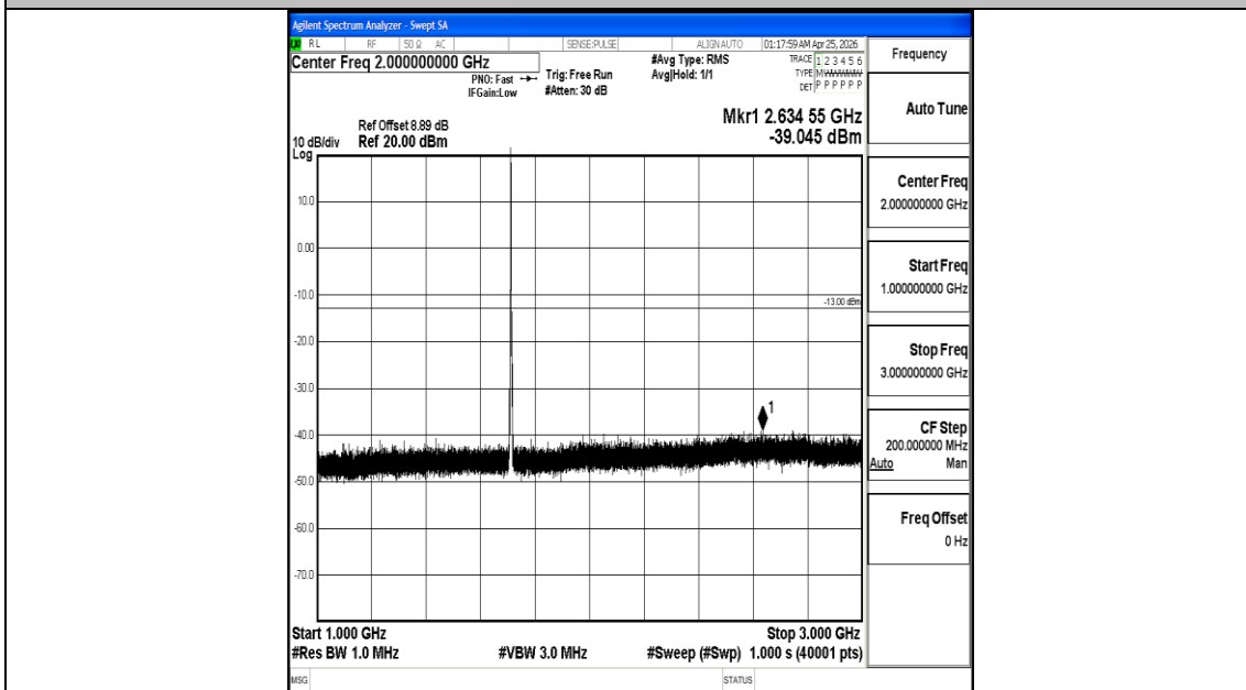
Band66_3MHz_16QAM_131987_1RB#0_1000~3000_1000~3000
