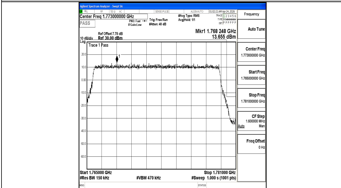
Band66_15MHz_16QAM_132597_75RB#0
