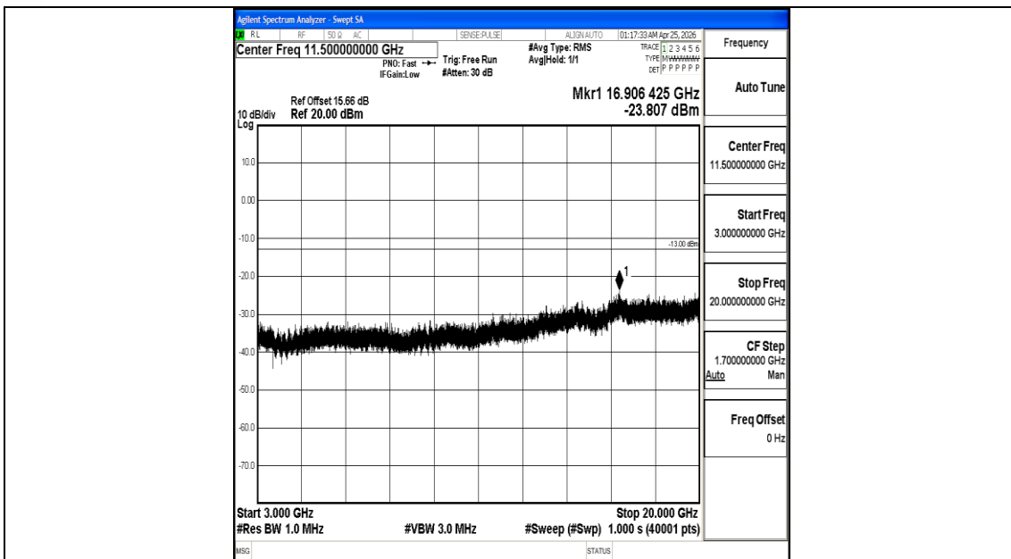
Band66_3MHz_QPSK_131987_1RB#0_3000~20000_3000~20000
