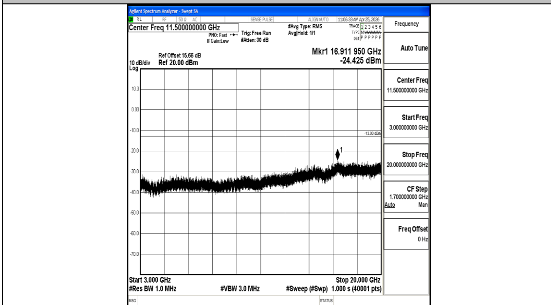
Band66_1.4MHz_16QAM_132665_1RB#0_3000~20000_3000~20000
