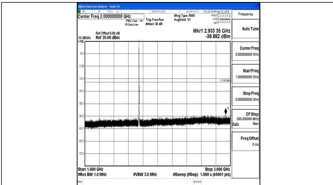
Band66_3MHz_QPSK_132322_1RB#0_1000~3000_1000~3000
