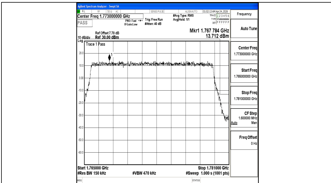
Band66_15MHz_QPSK_132597_75RB#0
