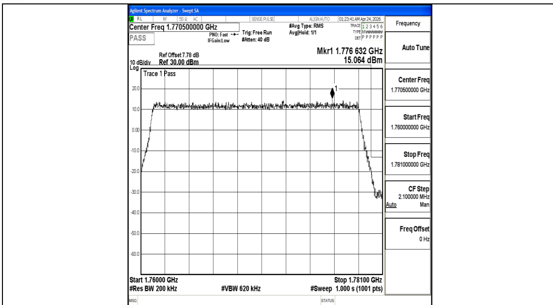
Band66_20MHz_QPSK_132572_100RB#0
