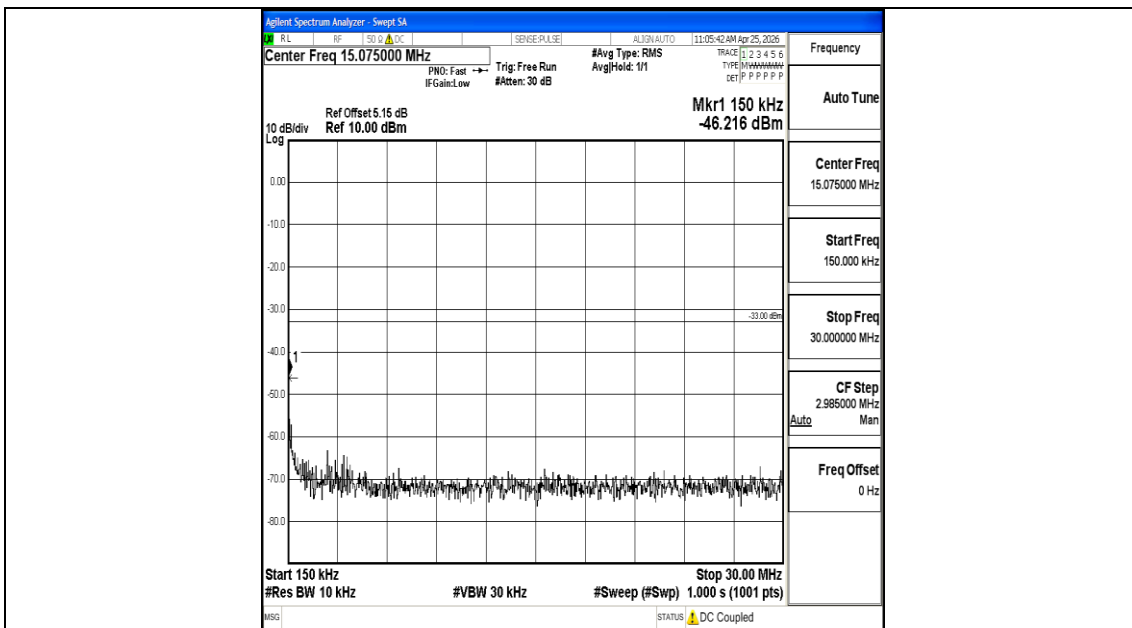
Band66_1.4MHz_QPSK_132665_1RB#0_0.15~30_0.15~30
