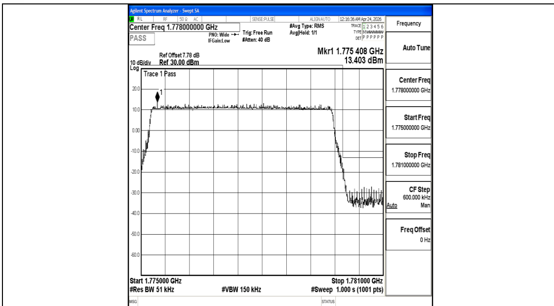
Band66_5MHz_QPSK_132647_25RB#0
