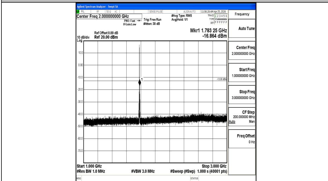
Band66_1.4MHz_16QAM_132665_1RB#0_1000~3000_1000~3000
