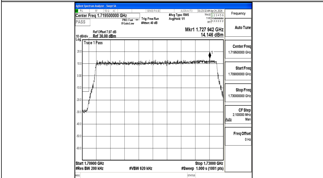
Band66_20MHz_16QAM_132072_100RB#0
