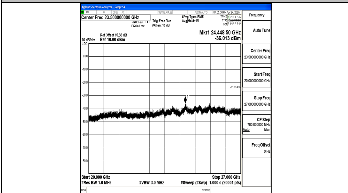
Band7_15MHz_QPSK_21375_1RB#0_20000~27000_20000~27000
