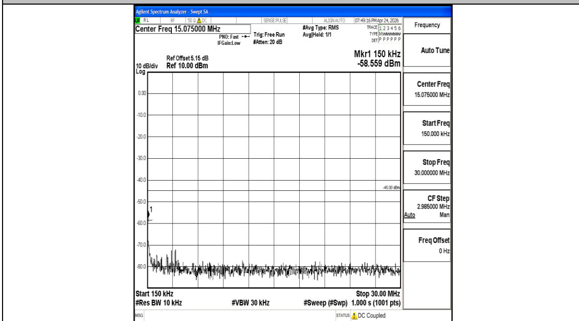
Band7_15MHz_QPSK_20825_1RB#0_0.15~30_0.15~30
