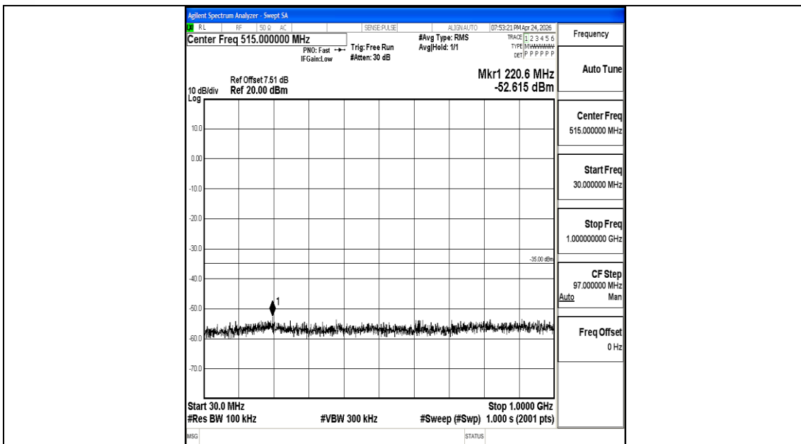
Band7_20MHz_16QAM_20850_1RB#0_30~1000_30~1000
