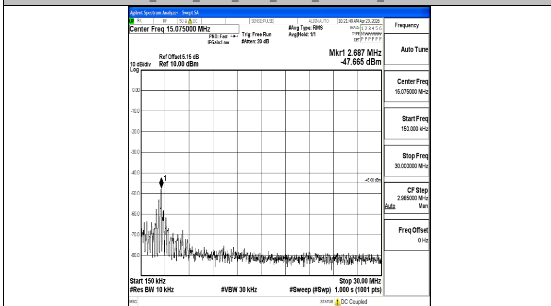
Band7_10MHz_QPSK_21100_1RB#0_0.15~30_0.15~30
