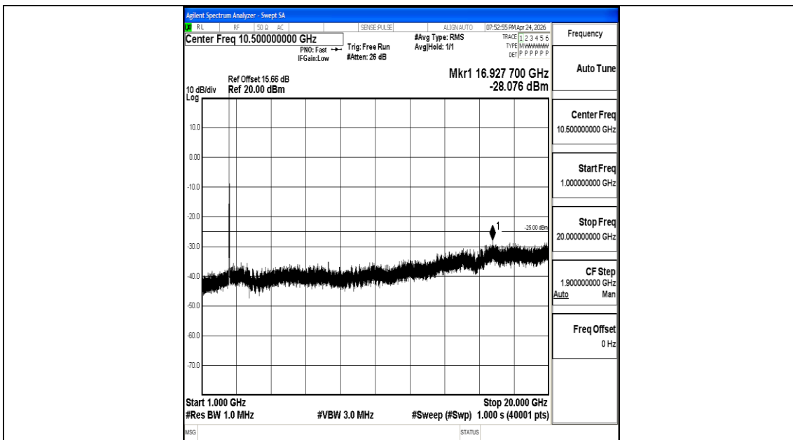
Band7_20MHz_QPSK_20850_1RB#0_1000~20000_1000~20000
