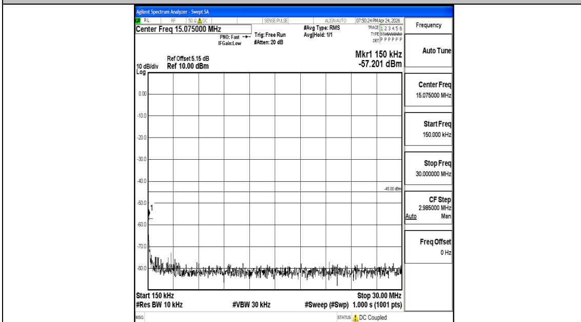
Band7_15MHz_QPSK_21100_1RB#0_0.15~30_0.15~30
