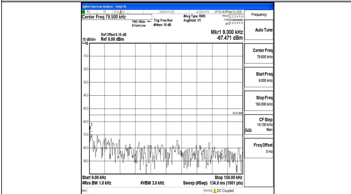
Band7_15MHz_QPSK_21375_1RB#0_0.009~0.15_0.009~0.15
