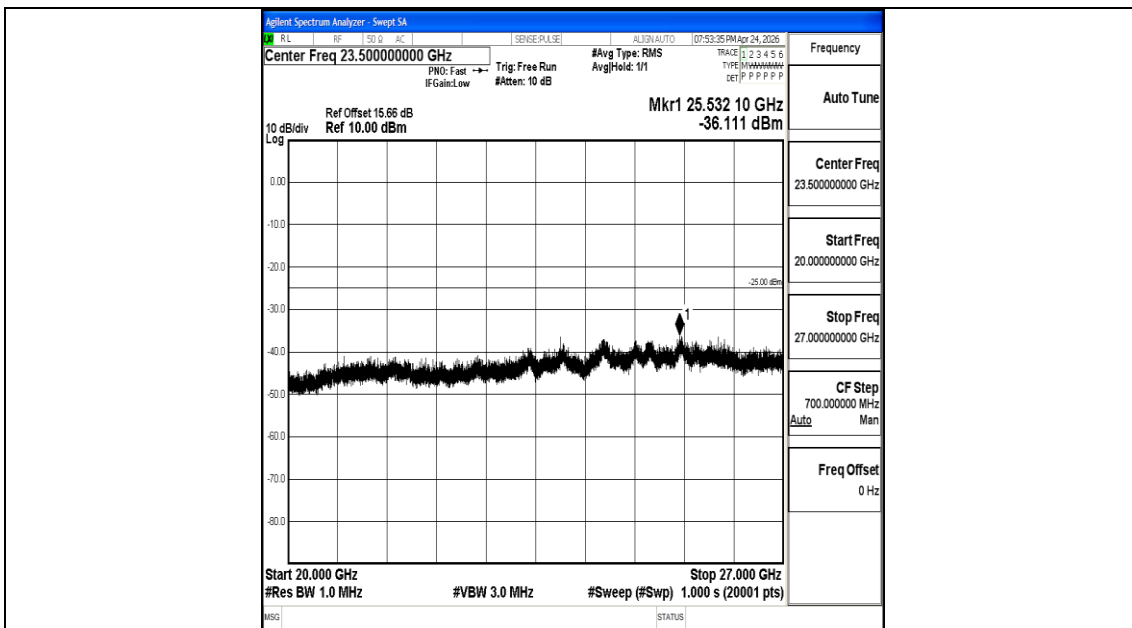
Band7_20MHz_16QAM_20850_1RB#0_20000~27000_20000~27000
