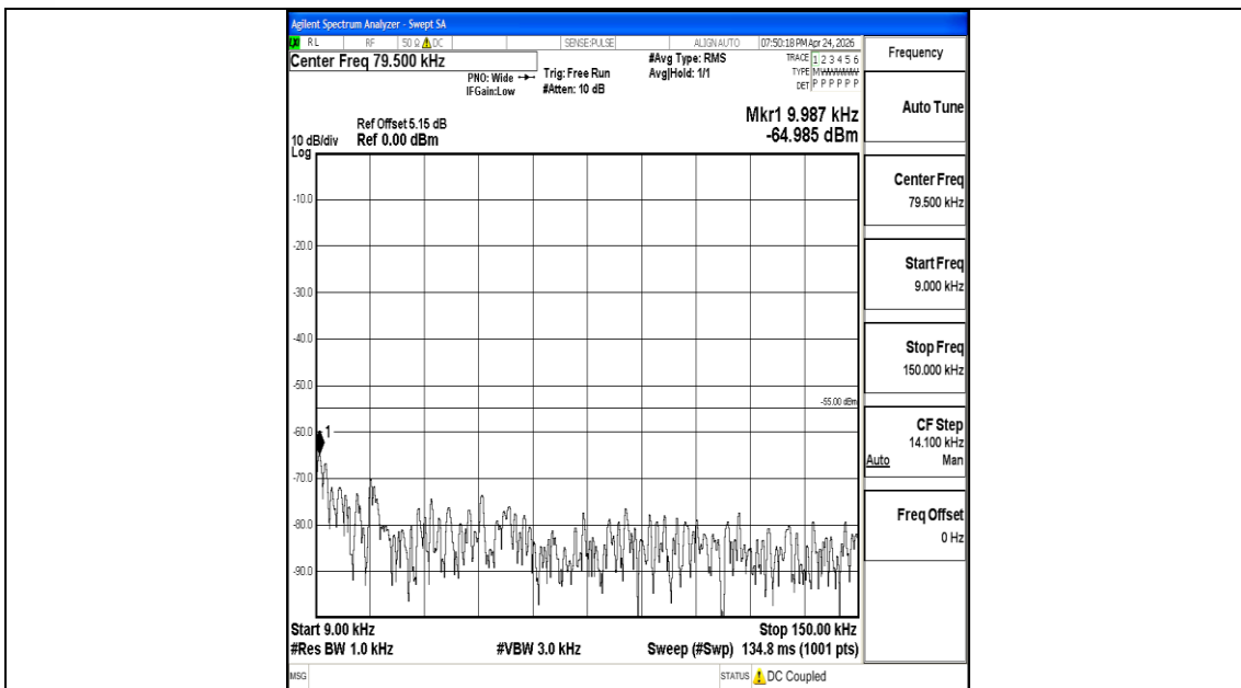
Band7_15MHz_QPSK_21100_1RB#0_0.009~0.15_0.009~0.15
