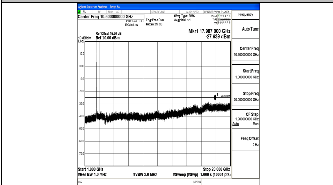
Band7_20MHz_16QAM_20850_1RB#0_1000~20000_1000~20000
