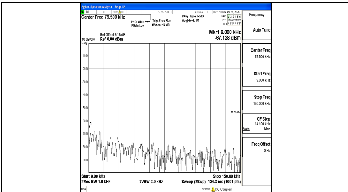
Band7_20MHz_16QAM_20850_1RB#0_0.009~0.15_0.009~0.15
