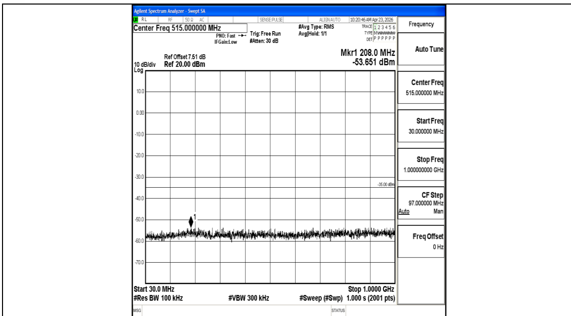
Band7_10MHz_QPSK_20800_1RB#0_30~1000_30~1000
