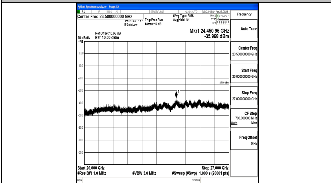
Band7_10MHz_16QAM_21400_1RB#0_20000~27000_20000~27000
