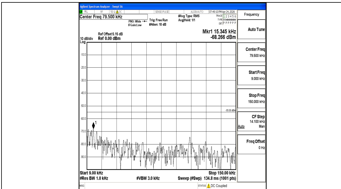
Band7_15MHz_QPSK_20825_1RB#0_0.009~0.15_0.009~0.15
