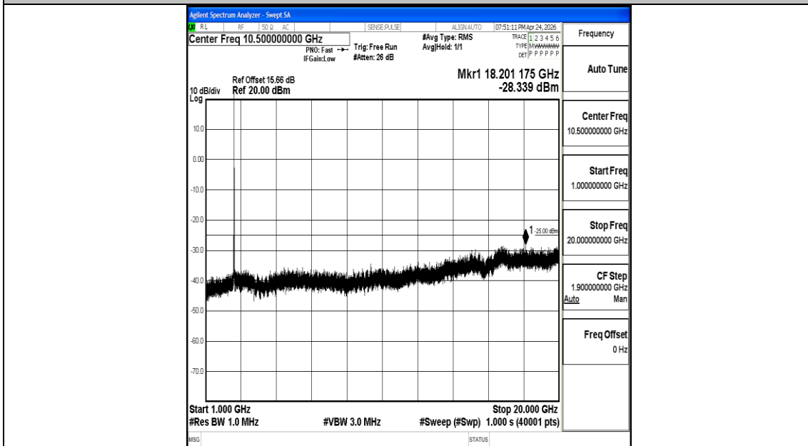
Band7_15MHz_16QAM_21100_1RB#0_1000~20000_1000~20000
