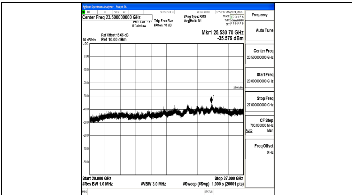
Band7_15MHz_16QAM_21100_1RB#0_20000~27000_20000~27000
