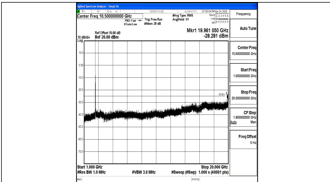
Band7_15MHz_16QAM_20825_1RB#0_1000~20000_1000~20000
