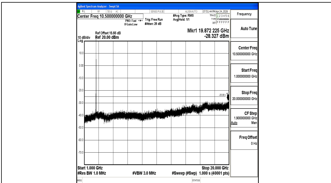
Band7_15MHz_QPSK_21375_1RB#0_1000~20000_1000~20000
