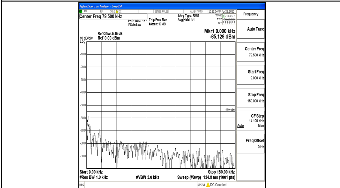
Band7_10MHz_16QAM_21100_1RB#0_0.009~0.15_0.009~0.15
