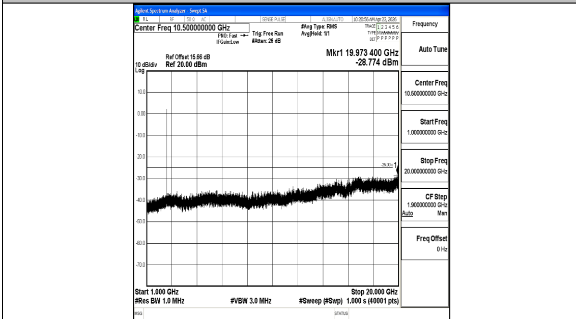
Band7_10MHz_QPSK_20800_1RB#0_1000~20000_1000~20000
