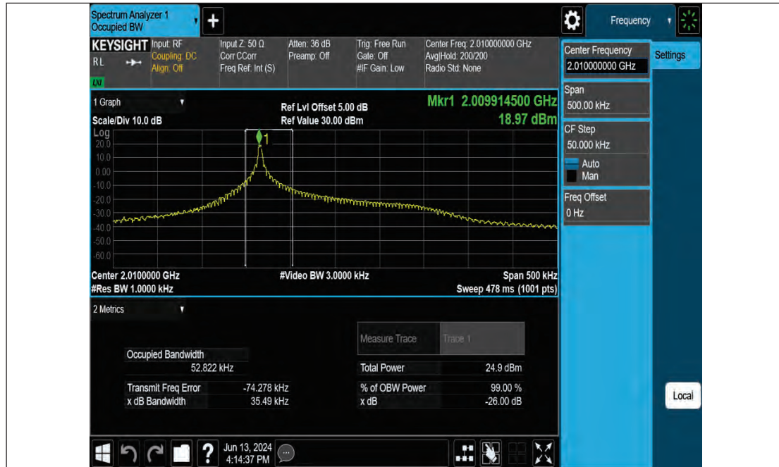
Band23-3.75kHz-OBW-M-BPSK-1@46
