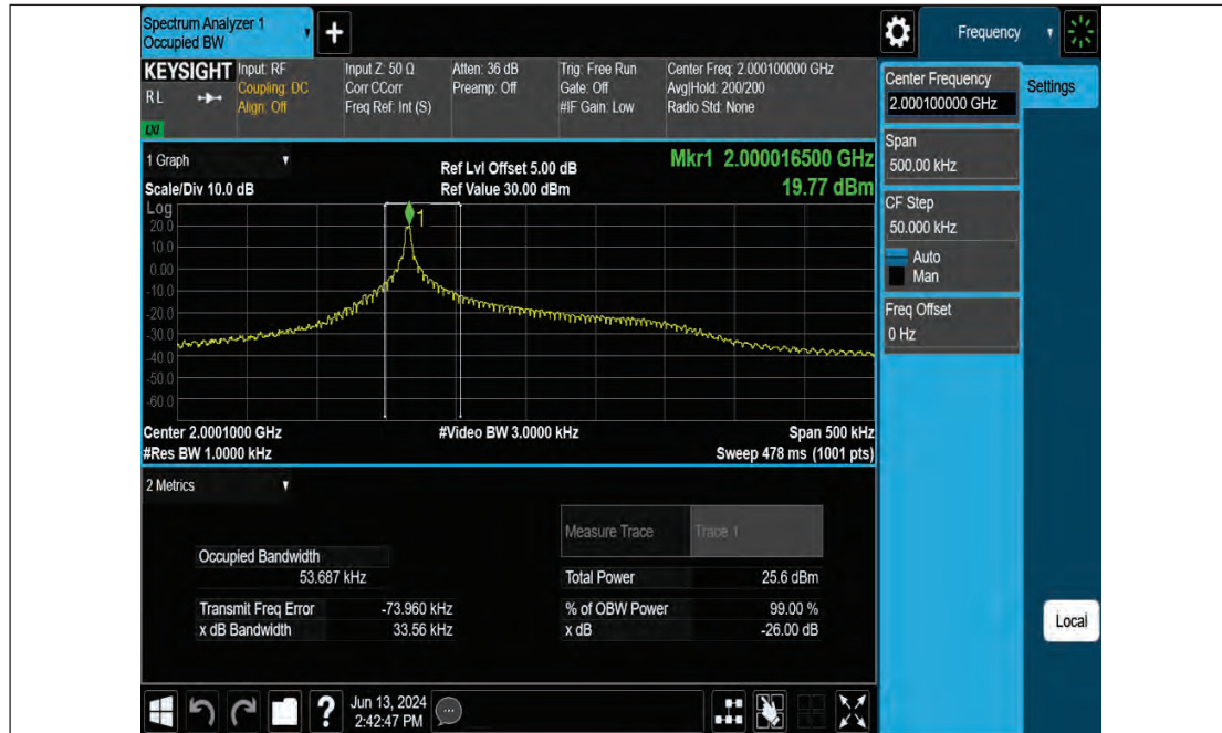
Band23-3.75kHz-OBW-L-QPSK-1@46
