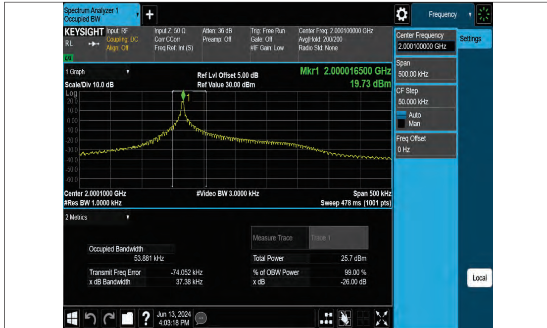
Band23-3.75kHz-OBW-L-BPSK-1@46
