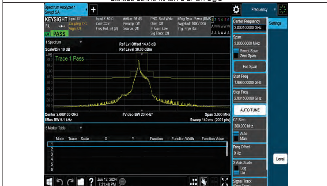
Band23-15kHz-MASK-L-BPSK-1@1
