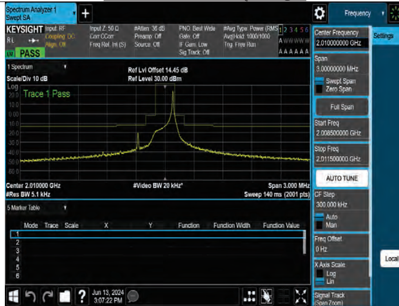
Band23-3.75kHz-MASK-M-BPSK-1@1
