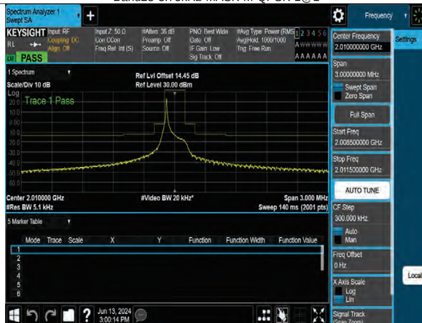
Band23-3.75kHz-MASK-M-QPSK-1@1
