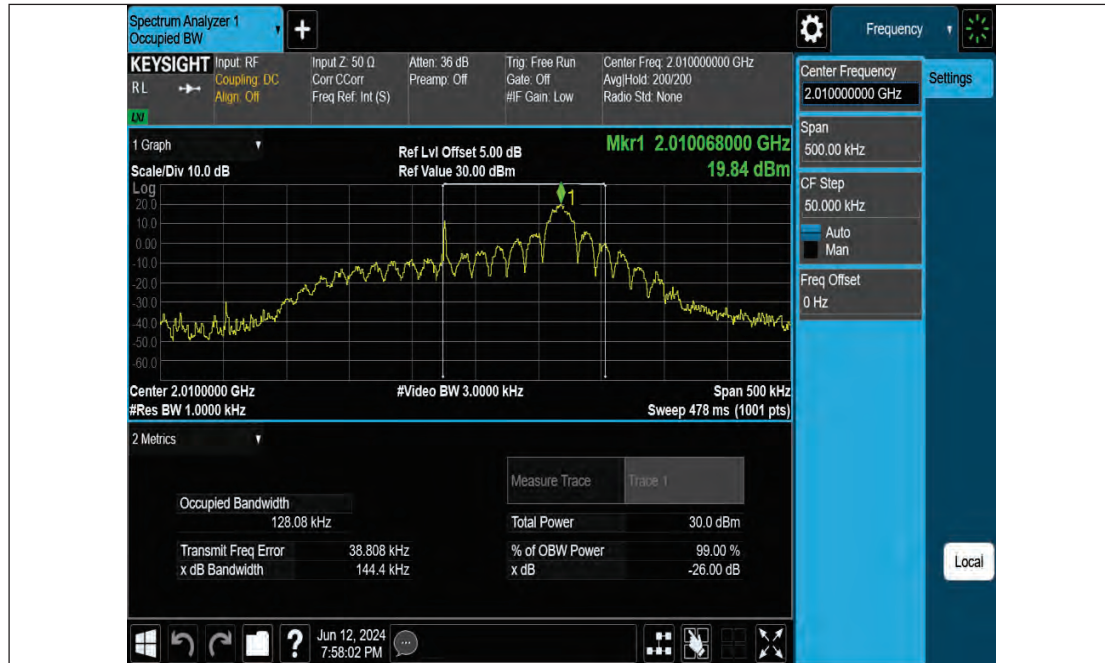
Band23-15kHz-OBW-H-QPSK-12@0
