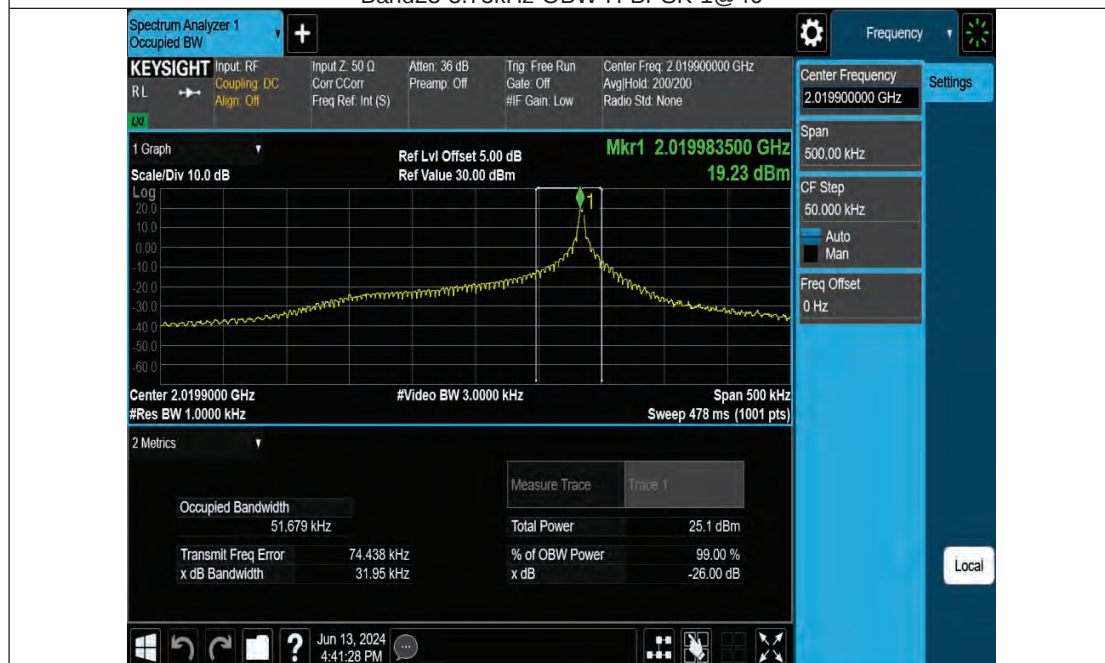
Band23-3.75kHz-OBW-H-BPSK-1@46
