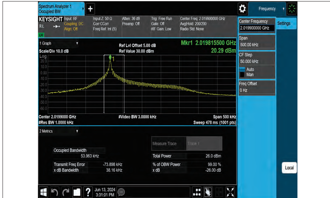
Band23-3.75kHz-OBW-H-QPSK-1@46
