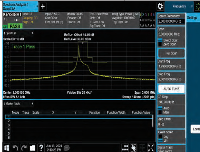
Band23-3.75kHz-MASK-L-QPSK-1@1
