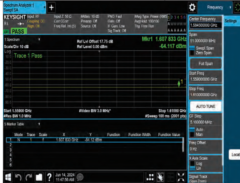
Band23-15kHz-Discrete emission-M-BPSK-1@1
