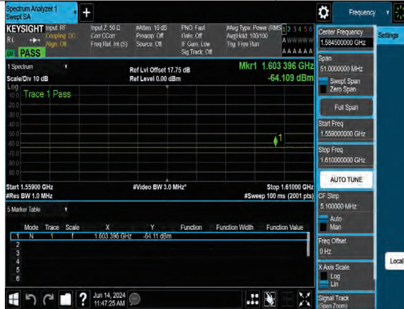
Band23-15kHz-Discrete emission-L-BPSK-1@1
