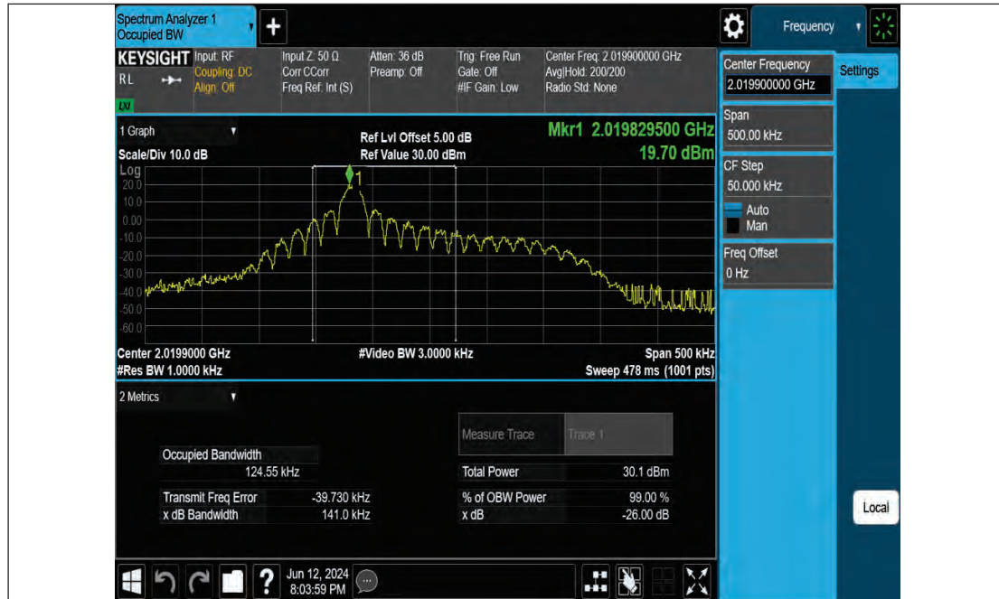
Band23-15kHz-OBW-H-BPSK-1@10
