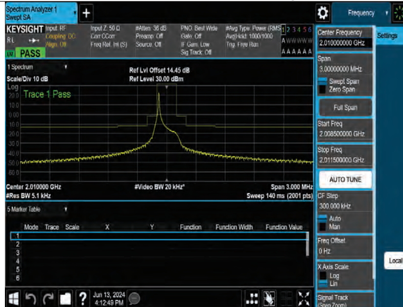
Band23-3.75kHz-MASK-M-BPSK-1@1
