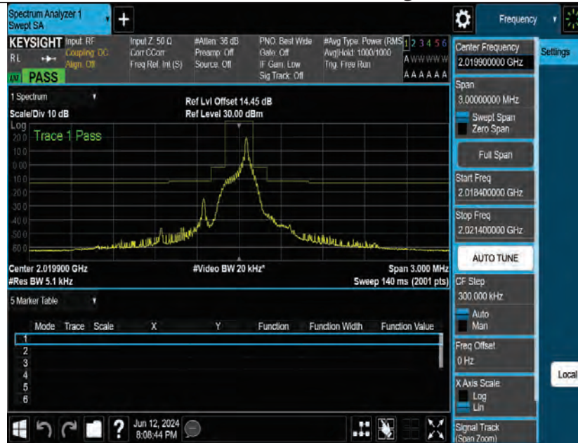
Band23-3.75kHz-MASK-L-QPSK-1@1
