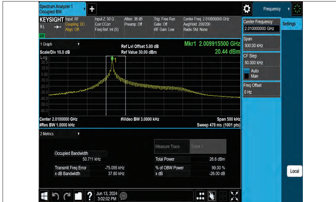
Band23-3.75kHz-OBW-M-QPSK-1@46
