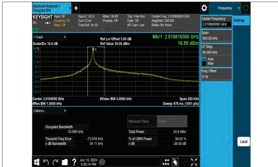
Band23-3.75kHz-OBW-H-BPSK-1@46
