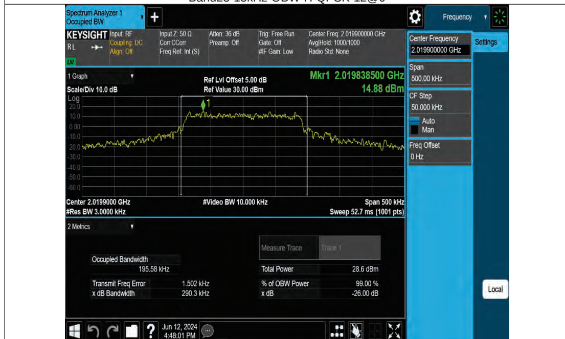
Band23-15kHz-OBW-H-QPSK-1@1
