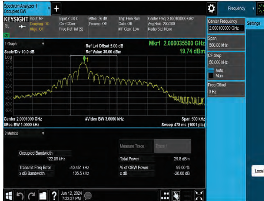
Band23-15kHz-OBW-L-BPSK-1@1
