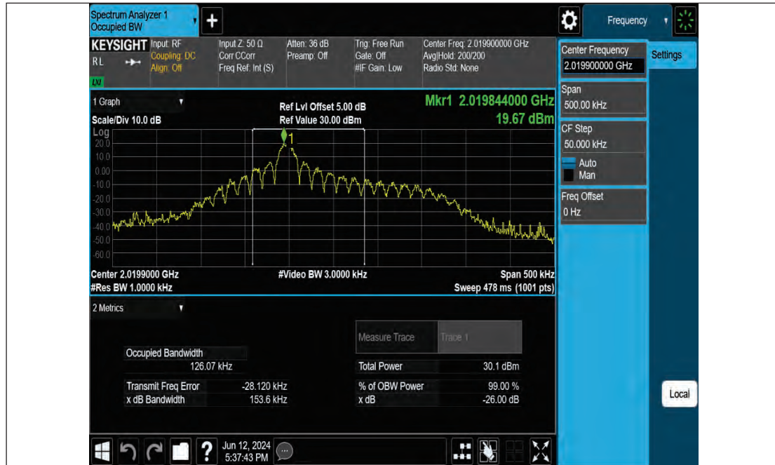
Band23-15kHz-OBW-H-QPSK-1@10
