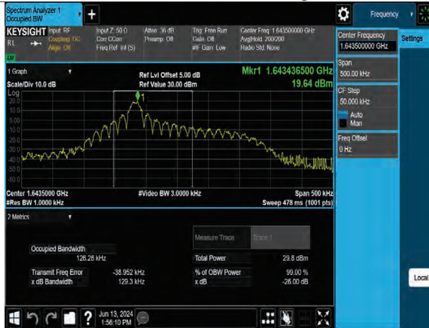
Band255-15kHz-OBW-M-BPSK-1@10
