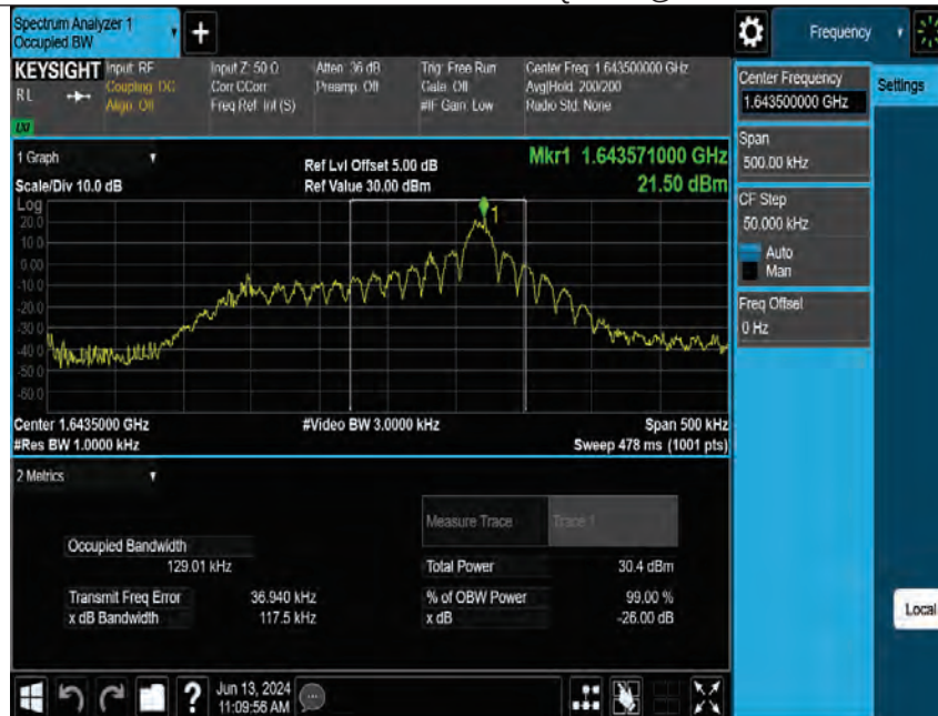
Band255-15kHz-OBW-M-QPSK-1@10
