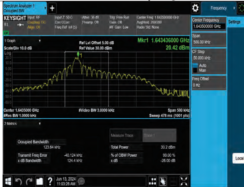
Band255-15kHz-OBW-M-QPSK-1@10
