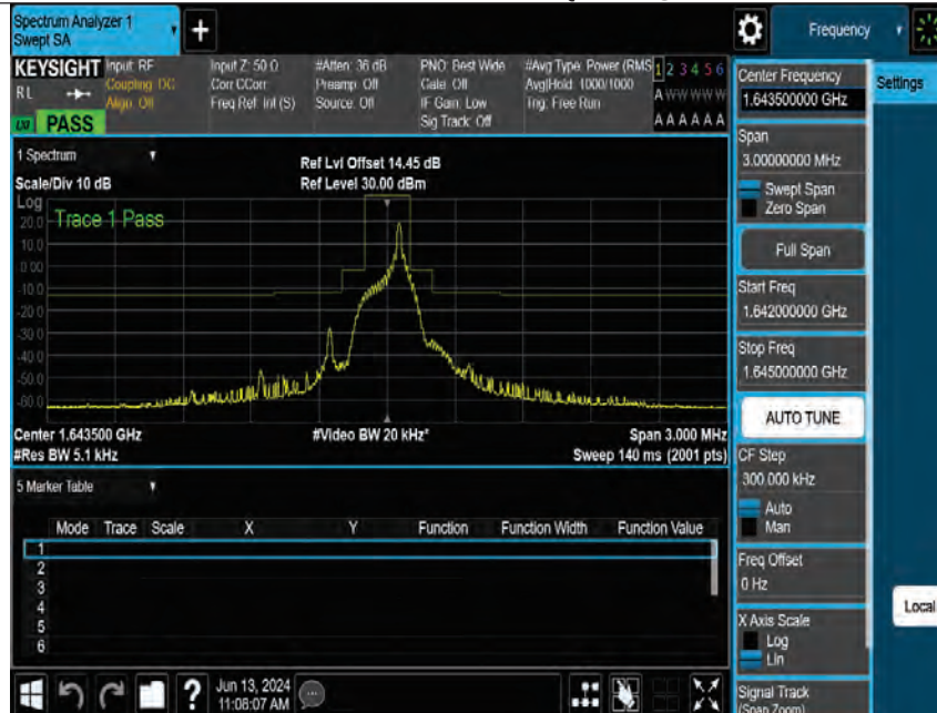
Band255-15kHz-MASK-M-QPSK-1@10
