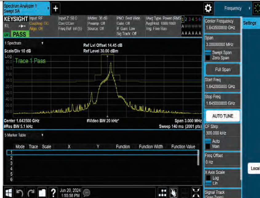
Band255-15kHz-MASK-M-BPSK-1@10
