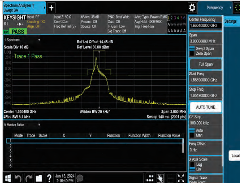
Band255-15kHz-MASK-H-BPSK-1@1
