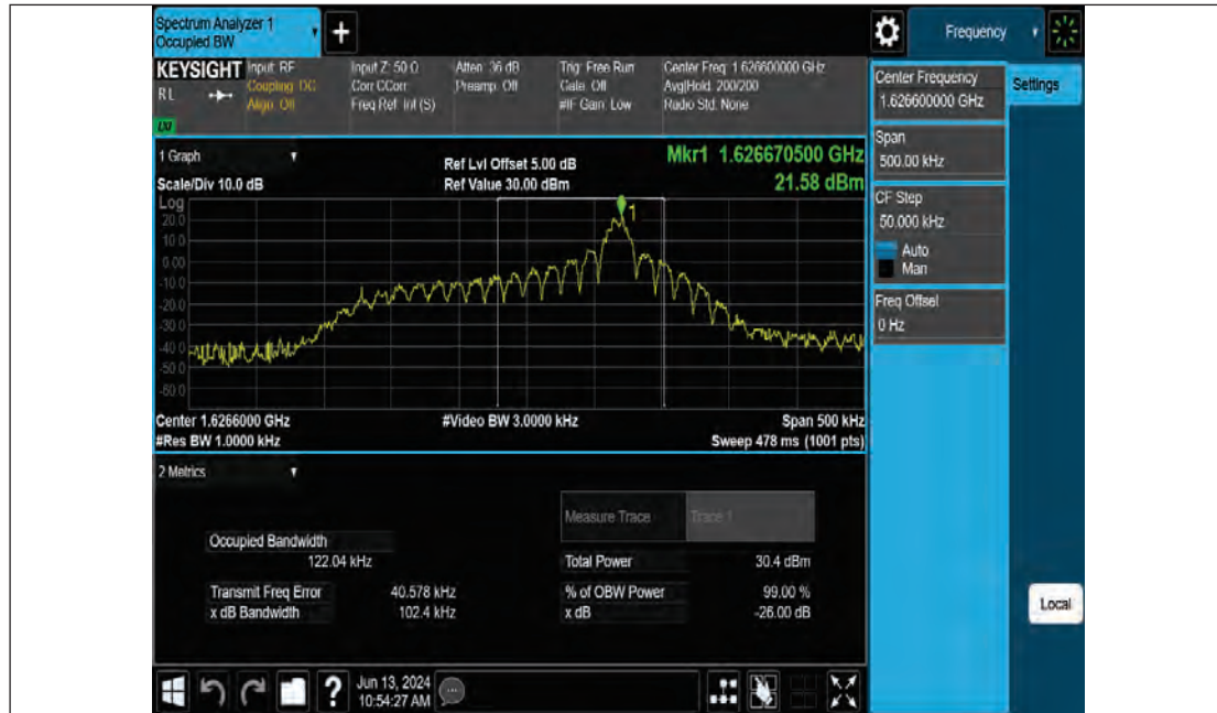
Band255-15kHz-OBW-L-BPSK-1@1
