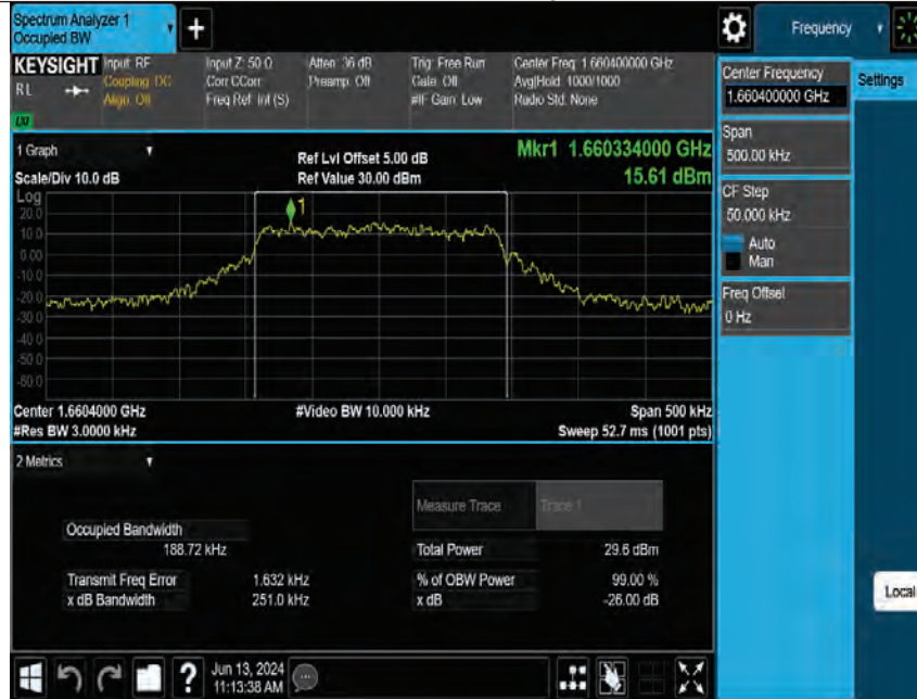
Band255-15kHz-OBW-H-QPSK-1@1
