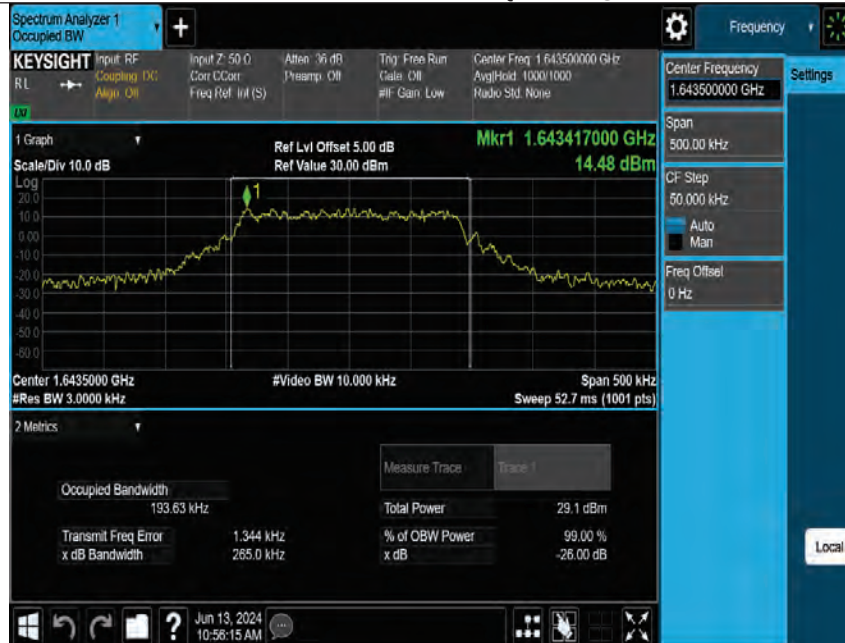
Band255-15kHz-OBW-M-QPSK-12@0
