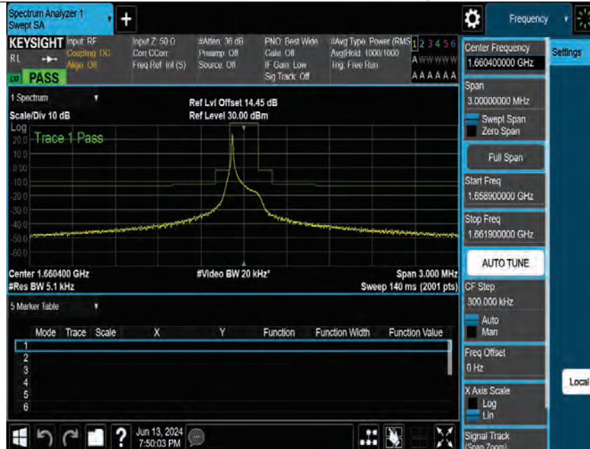
Band255-3.75kHz-MASK-H-BPSK-1@1
