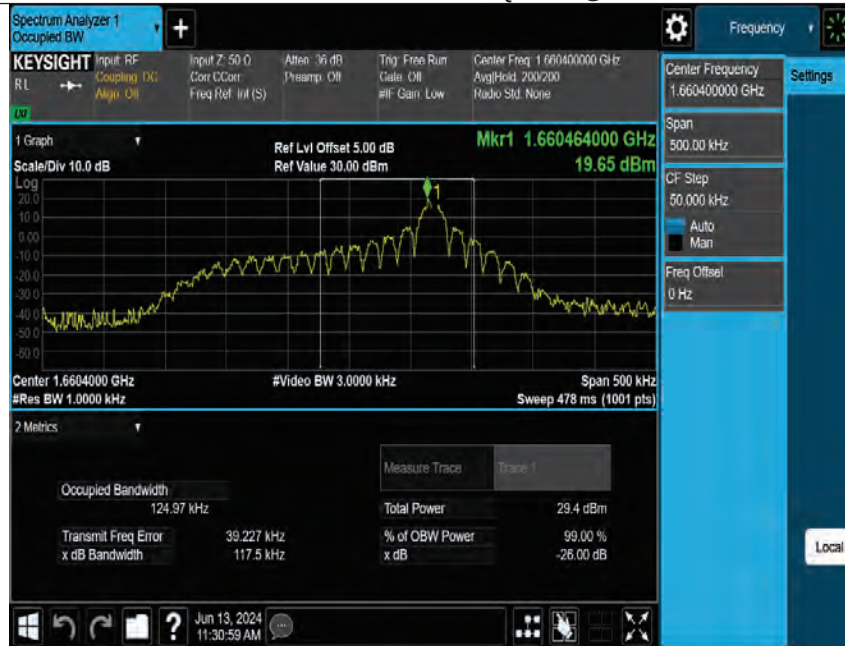
Band255-15kHz-OBW-H-BPSK-1@1
