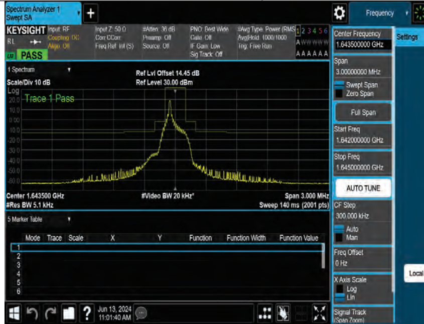
Band255-15kHz-MASK-M-QPSK-1@10
