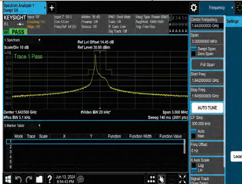
Band255-3.75kHz-MASK-M-QPSK-1@1
