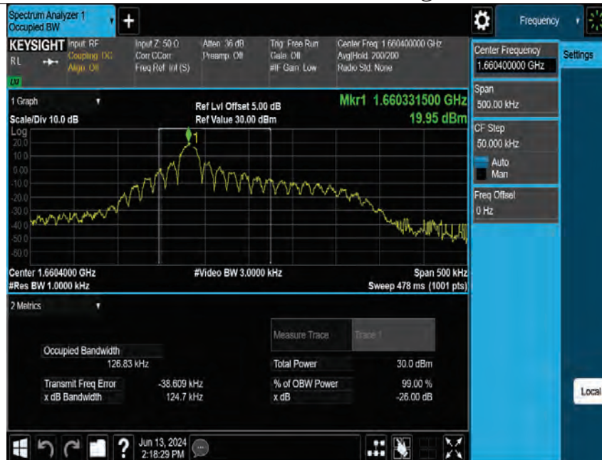
Band255-15kHz-OBW-H-BPSK-1@1
