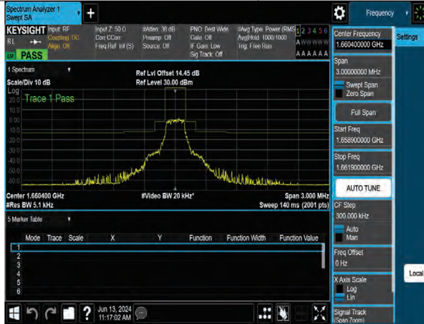
Band255-15kHz-MASK-H-QPSK-1@1
