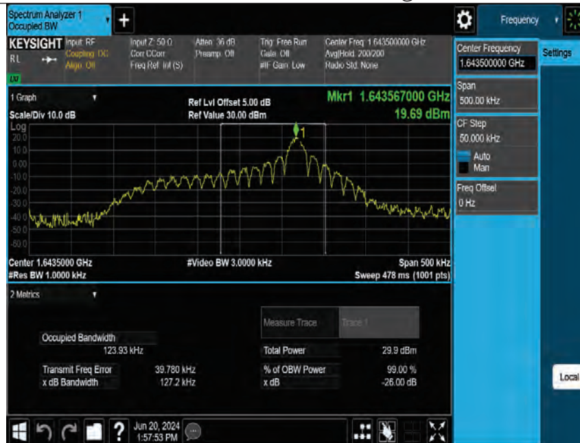
Band255-15kHz-OBW-M-BPSK-1@10
