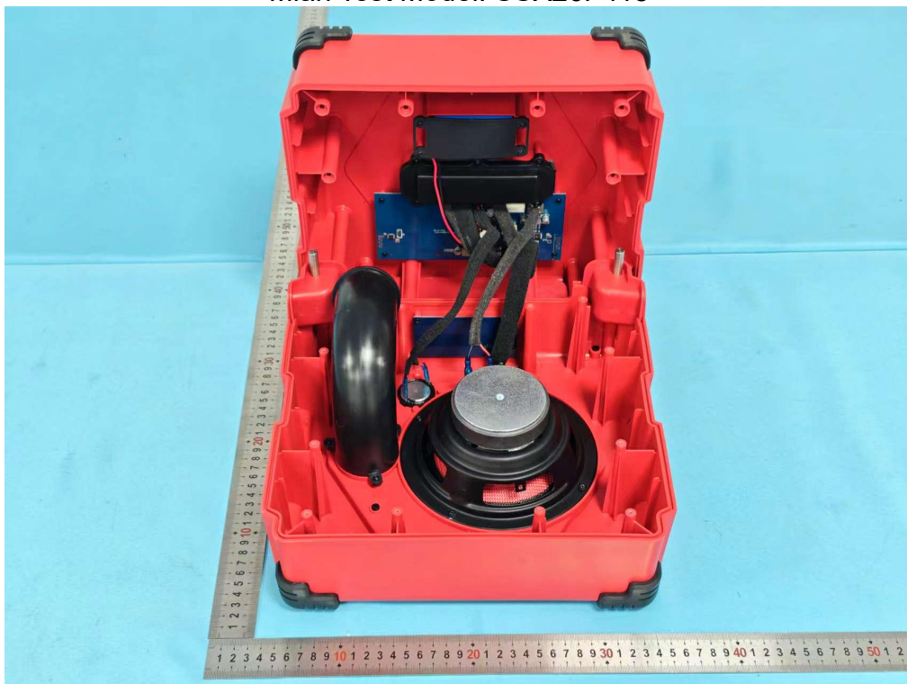
Photo 1 Internal photos of EUT Mian Test Model: SSX26P118
