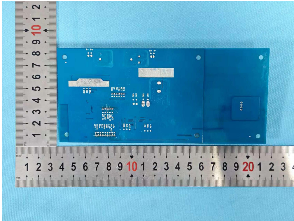
Photo 11 Internal photos of EUT Mian Test Model: SSX26P118
