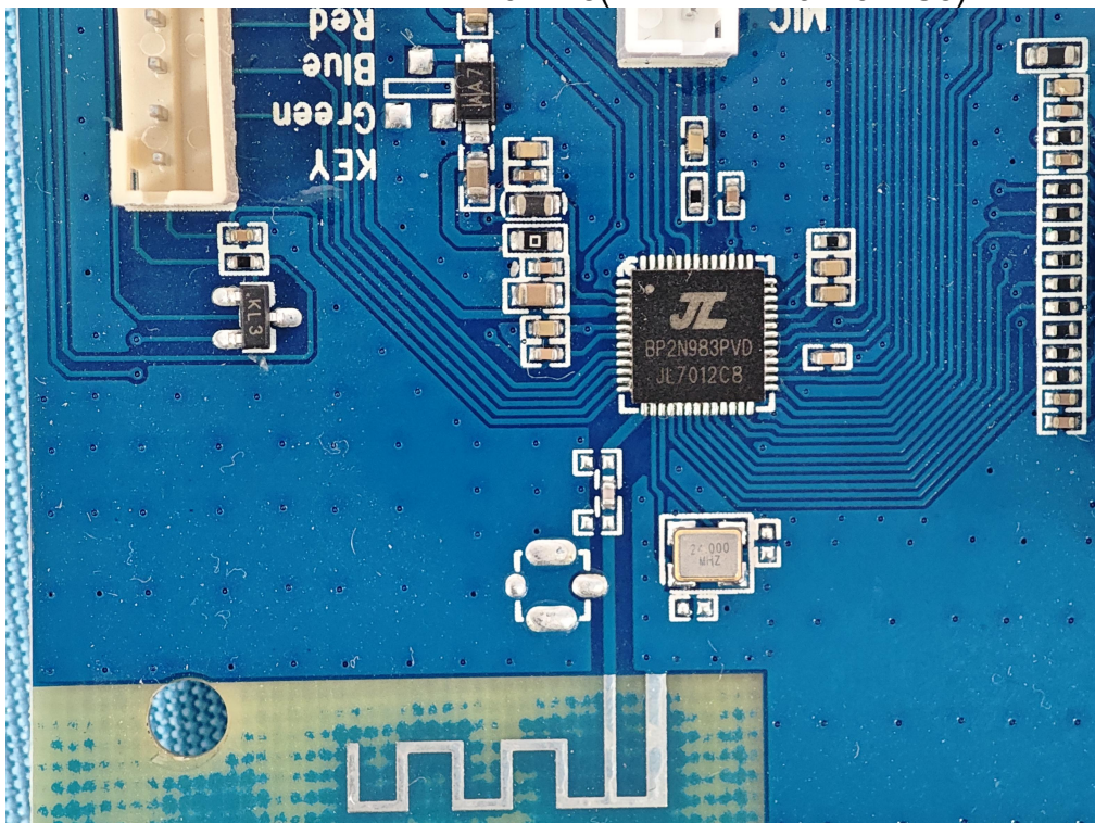
Photo 12 Internal photos of EUT Mian Test Model: SSX26P118(BT Module: JL7012C8)
