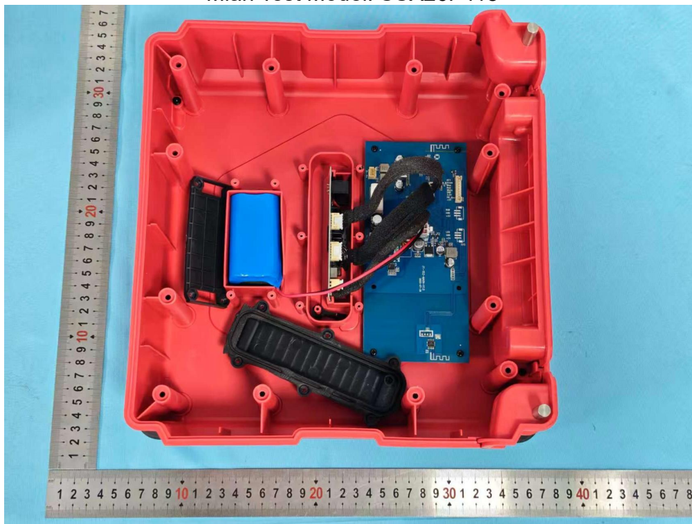
Photo 7 Internal photos of EUT Mian Test Model: SSX26P118
