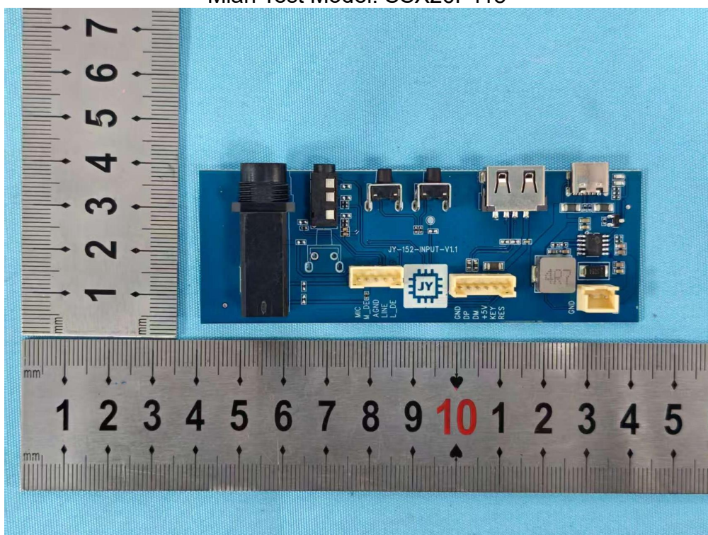
Photo 8 Internal photos of EUT Mian Test Model: SSX26P118-
