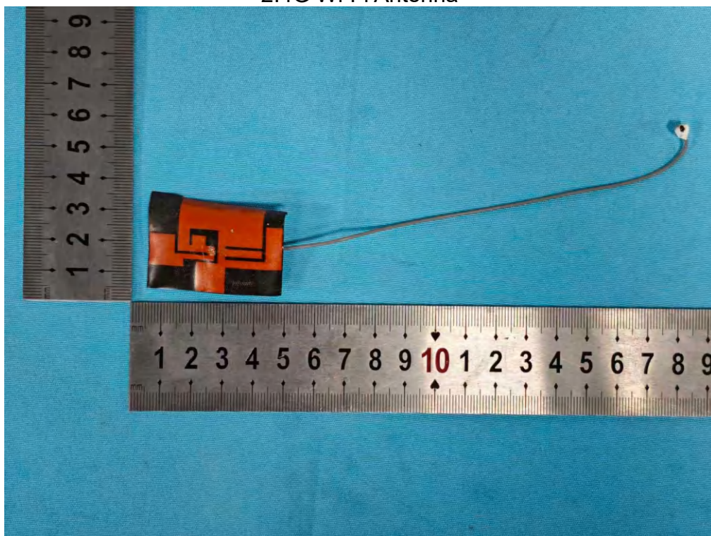
Photo 8 Internal photos of EUT 2.4G Wi-Fi Antenna
