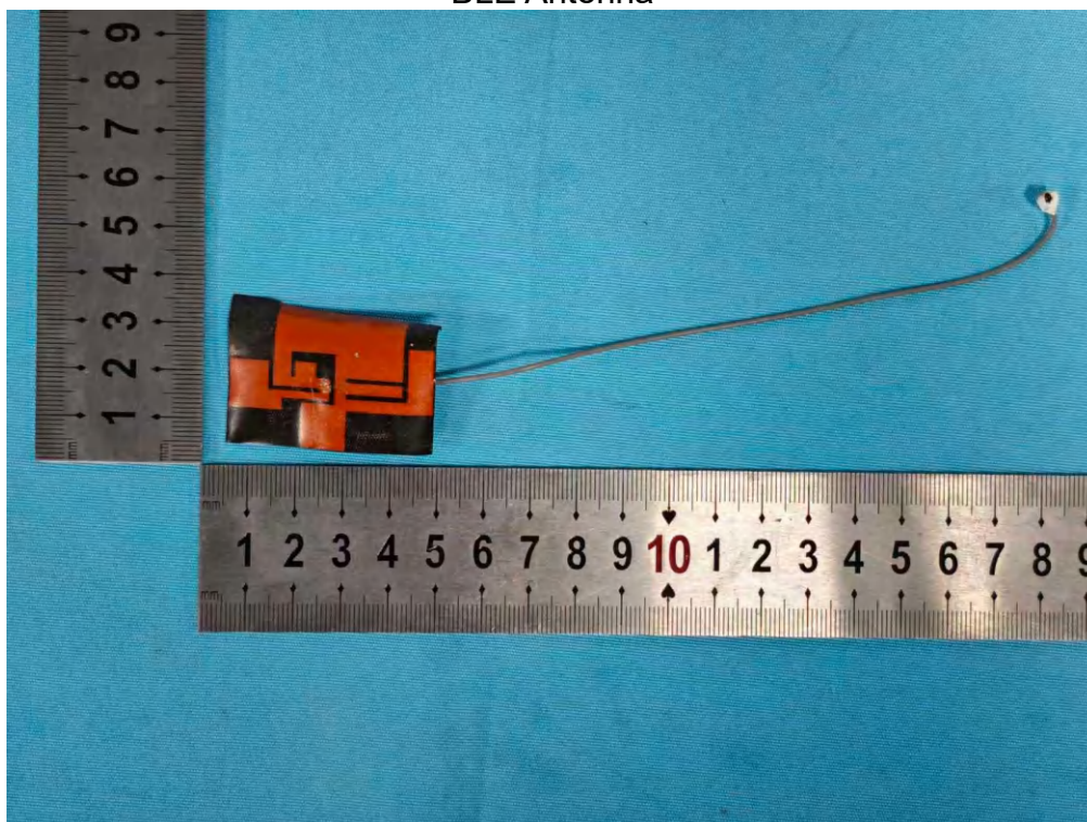
Photo 10 Internal photos of EUT BLE Antenna
