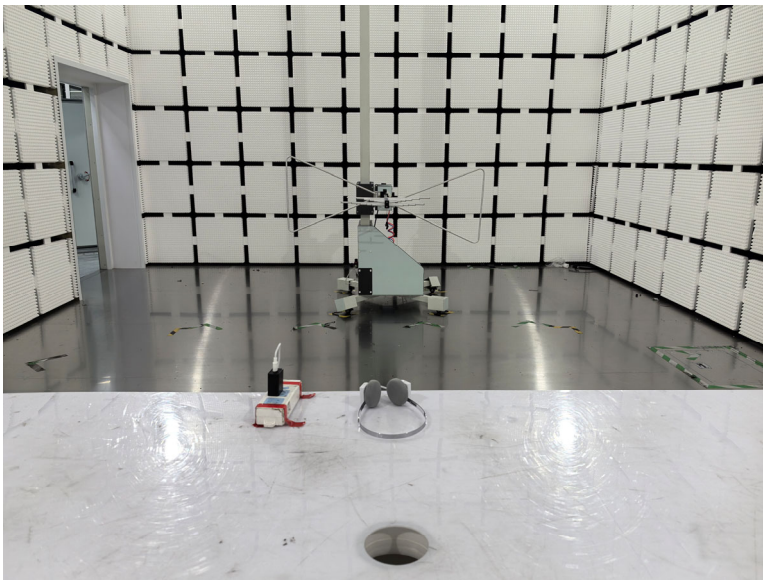
Radiated Emission
