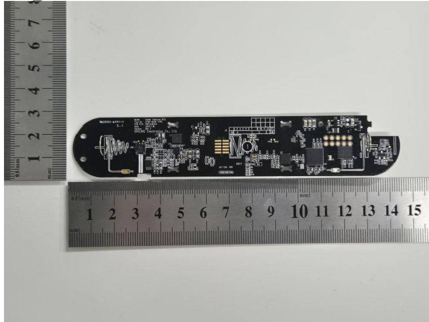
PCB FRONT
