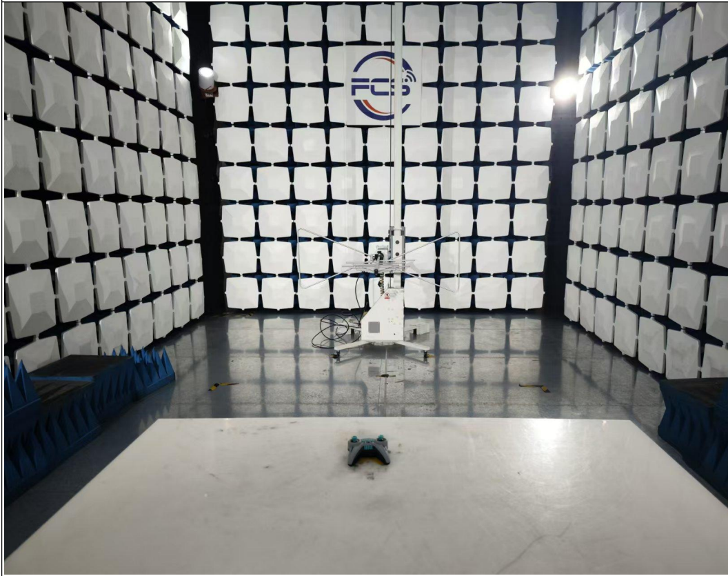
Above 1GHz for radiated emission test setup
