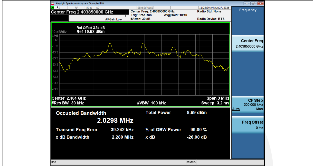
99% Occupied Bandwidth NVNT_ANT1_User_2403
