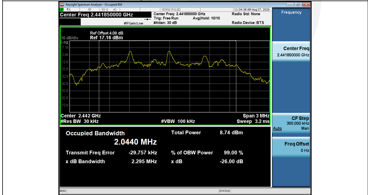
99% Occupied Bandwidth NVNT_ANT1_User_2441
