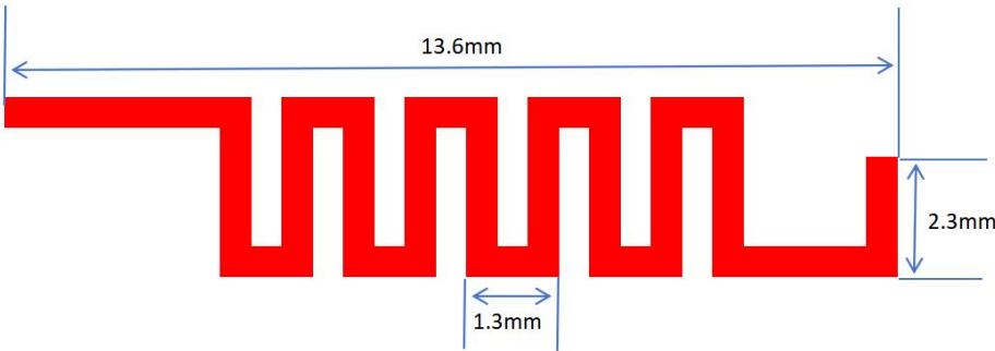
Antenna Photo & Length (mm)
