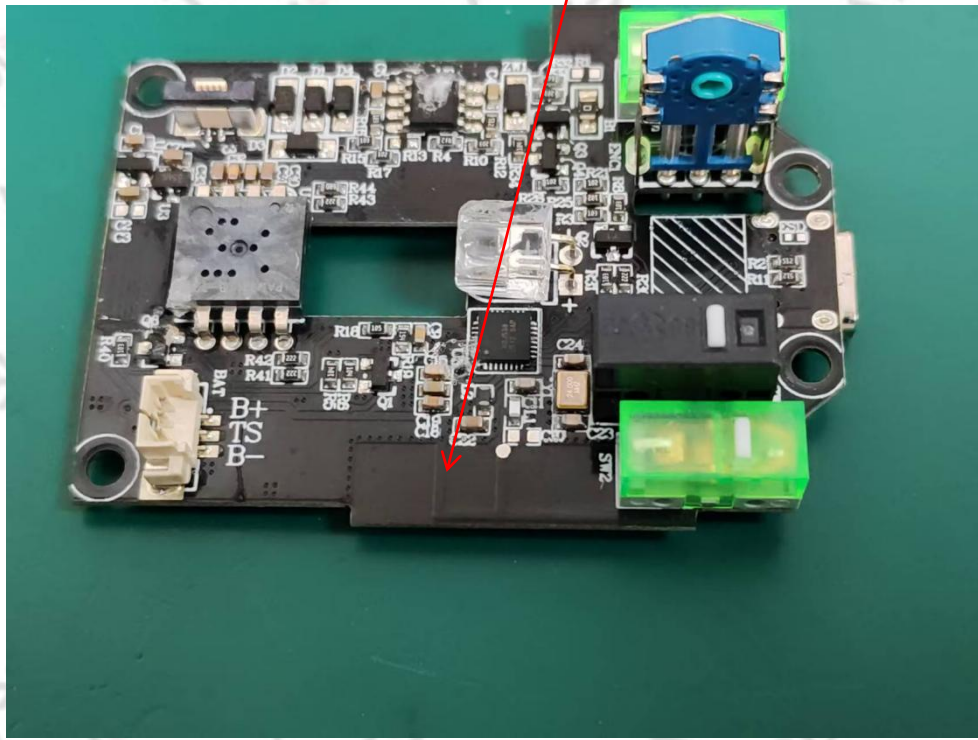
BT&2.4GHz_ANT
