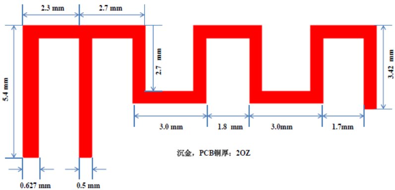
Antenna Dimension
