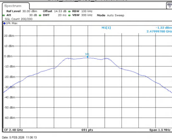
DH5_Ant1_2480_0~Reference
