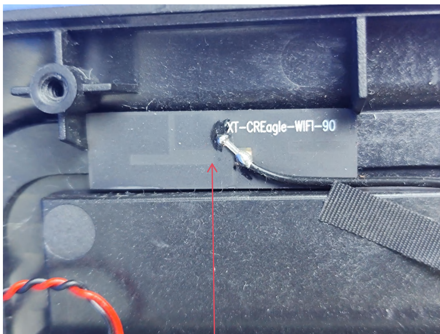
ANT 1(2.4GWIFI)
