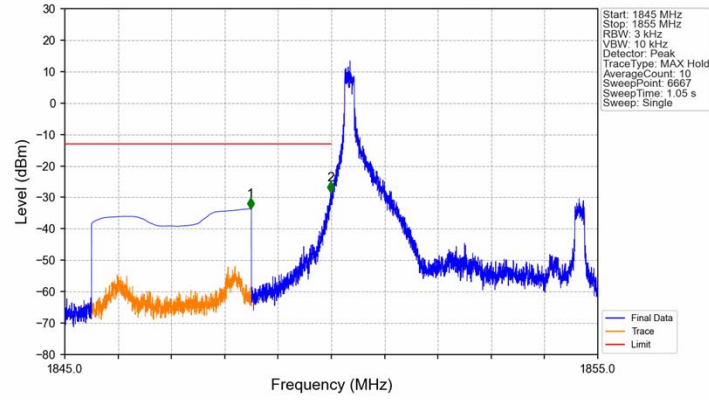
Band2_5MHz_QPSK_LCH_1852.5MHz_RB_1_0_NTNV
