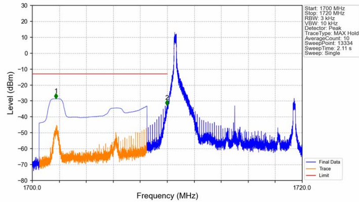
Band4_10MHz_QPSK_LCH_1715MHz_RB_1_0_NTNV
