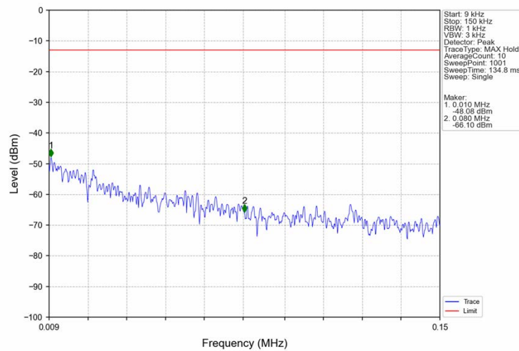
Band4_10MHz_QPSK_LCH_1715MHz_RB_1_0_NTNV
