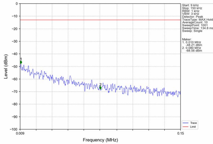
Band4_5MHz_16QAM_LCH_1712.5MHz_RB_1_0_NTNV
