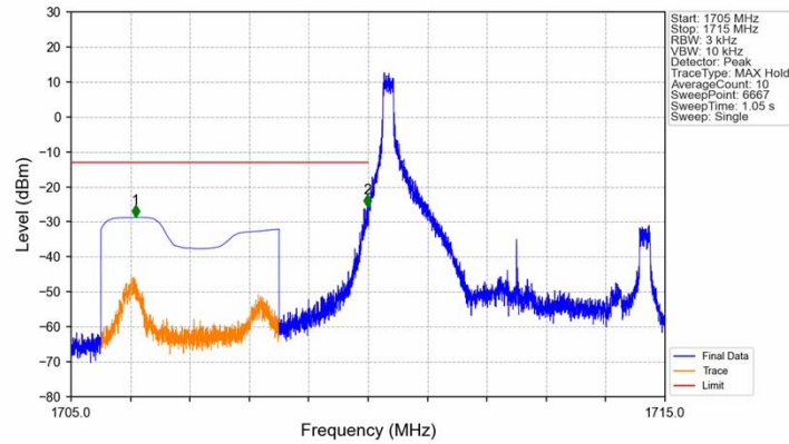
Band4_5MHz_QPSK_LCH_1712.5MHz_RB_1_0_NTNV
