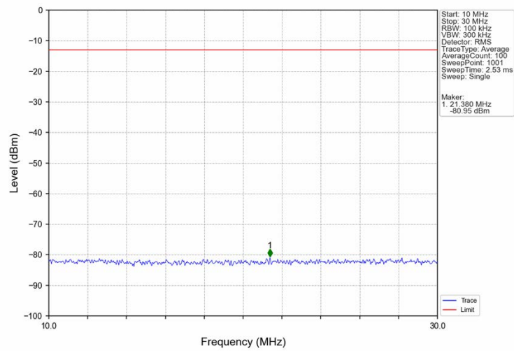
Band5_HSUPA_LCH_826.4MHz_Subtest 1_NTNV
