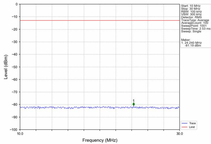
Band5_HSDPA_MCH_836.6MHz_Subtest 1_NTNV
