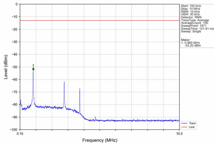
Band5_HSDPA_HCH_846.6MHz_Subtest 1_NTNV
