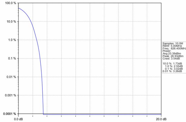
Band5_RMC_LCH_826.4MHz_12.2kbps RMC_NTNV
