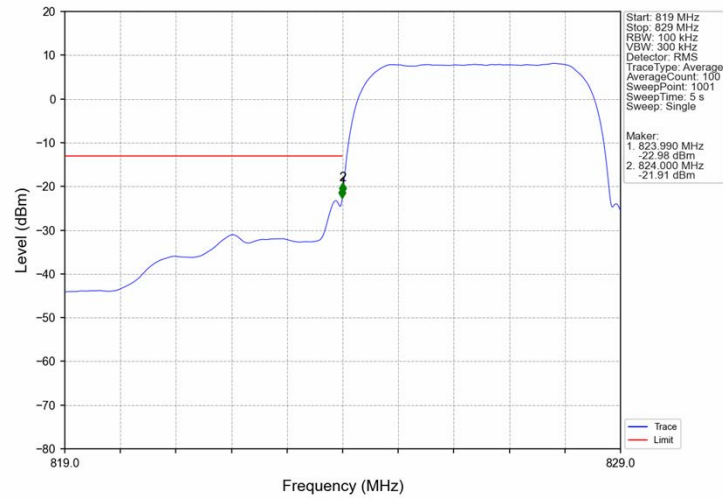
Band5_RMC_LCH_826.4MHz_12.2kbps RMC_NTNV
