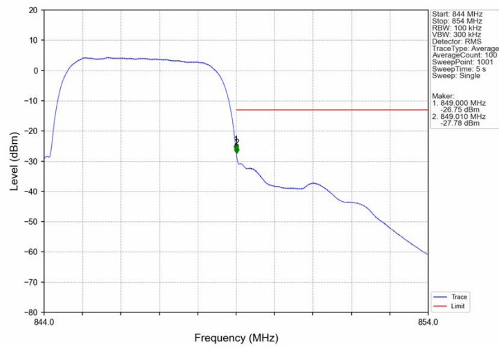
Band5_HSDPA_HCH_846.6MHz_Subtest 1_NTNV
