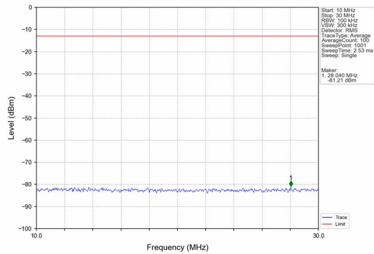
Band5_HSUPA_HCH_846.6MHz_Subtest 1_NTNV
