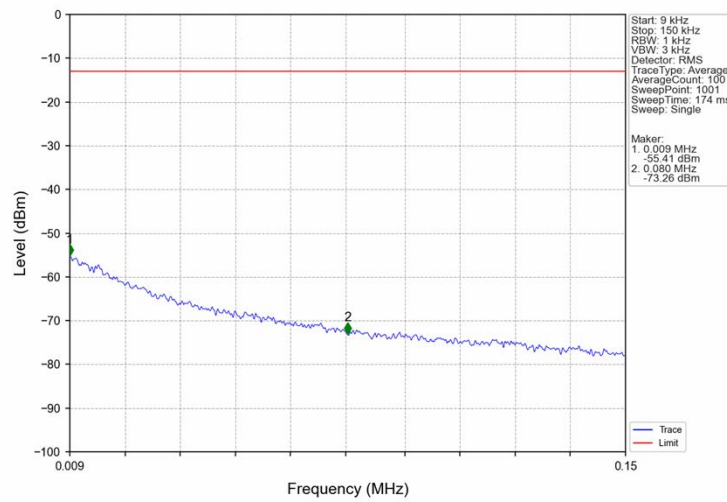
Band5_HSUPA_HCH_846.6MHz_Subtest 1_NTNV
