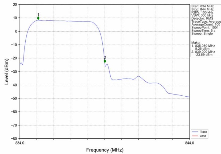
Band5_RMC_MCH_836.6MHz_12.2kbps RMC_NTNV
