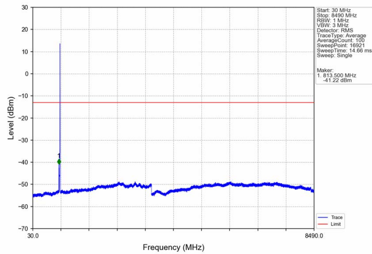
Band5_HSDPA_HCH_846.6MHz_Subtest 1_NTNV
