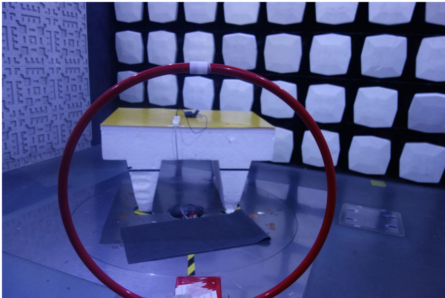
Radiated Emissions Below 1GHz
