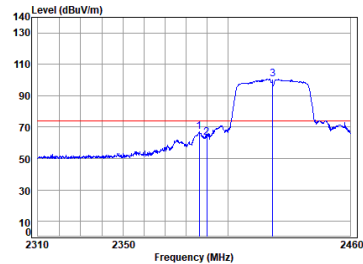
11n_HT(40M)_TX_CH_03_Vertical-Peak
