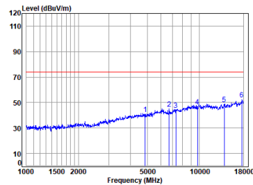
11n_HT(40M)_TX_CH_06_Vertical-Peak
