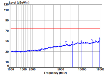
11n_HT(40M)_TX_CH_09_Horizontal-Peak
