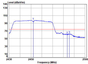
11n_HT(40M)_TX_CH_09_Vertical-Peak
