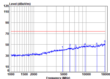
11n_HT(40M)_TX_CH_03_Horizontal-Peak
