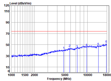
11n_HT(40M)_TX_CH_06_Horizontal-Peak
