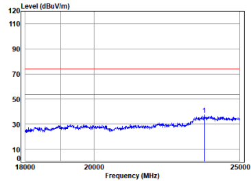
11b_TX_CH_06_Vertical-Peak
