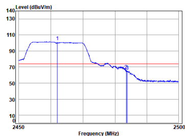
11n_HT(20M)_TX_CH_11_Vertical-Peak
