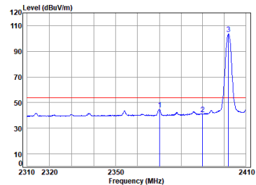
BLE_1M_TX_CH_00_Vertical-Avg
