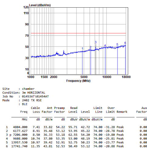
BLE_1M_TX_CH_00_Horizontal-Peak
