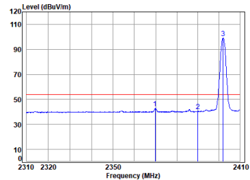
BLE_1M_TX_CH_00_Horizontal-Avg
