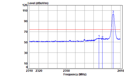
BLE_1M_TX_CH_00_Vertical-Peak
