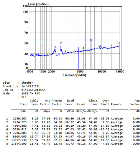
BLE_1M_TX_CH_00_Vertical-Avg
