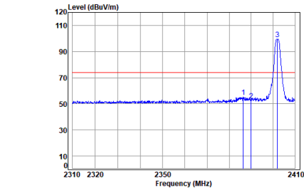
BLE_1M_TX_CH_00_Horizontal-Peak
