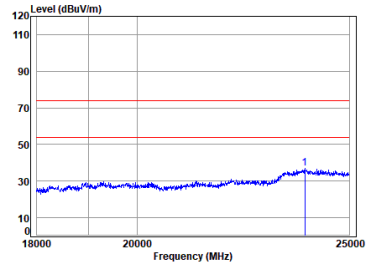
BLE_1M_TX_CH_19_Vertical-Peak
