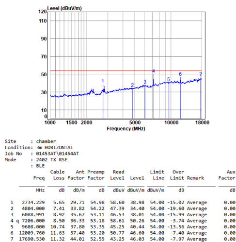
BLE_1M_TX_CH_00_Horizontal-Avg
