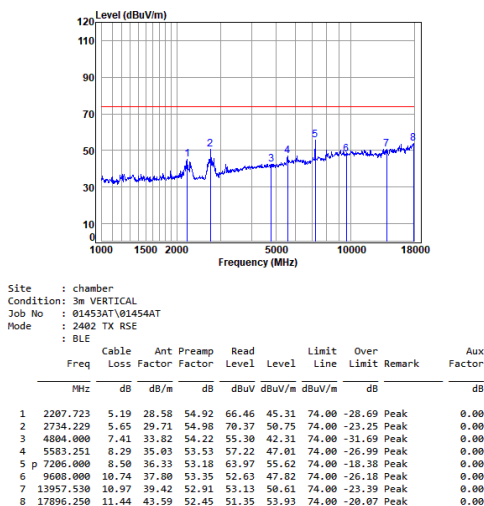
BLE_1M_TX_CH_00_Vertical-Peak
