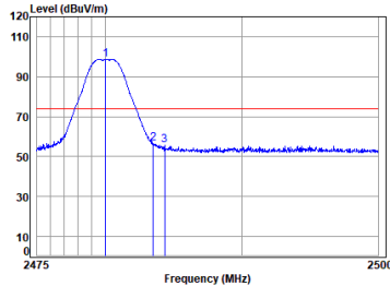
BLE_2M_TX_CH_39_Vertical-Peak
