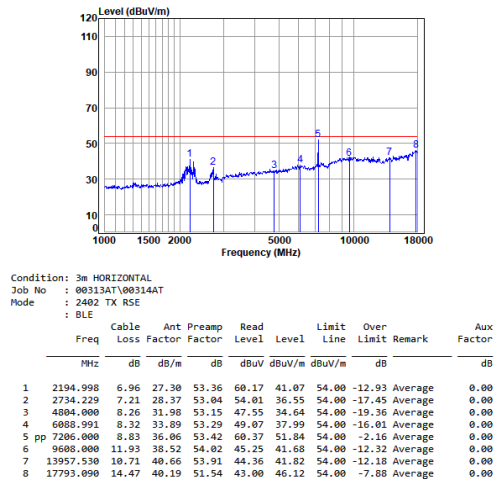
BLE_1M_TX_CH_00_Horizontal-Avg
