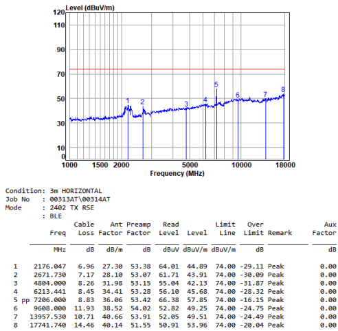
BLE_1M_TX_CH_00_Horizontal-Peak
