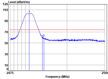
BLE_2M_TX_CH_39_Horizontal-Peak
