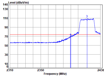
11ax_20M_TX_CH_01_Horizontal-Peak
