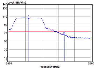
11g_TX_CH_11_Vertical-Peak
