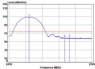
11b_TX_CH_11_Horizontal-Peak
