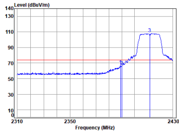
11g_TX_CH_01_Vertical-Peak
