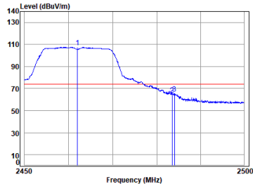
11g_TX_CH_11_Horizontal-Peak
