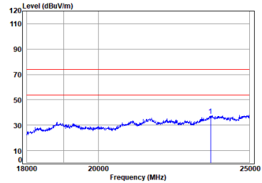
11b_TX_CH_06_Vertical-Peak
