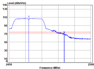
11n_HT(20M)_TX_CH_11_Vertical-Peak
