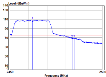
11ax_20M_TX_CH_11_Vertical-Peak
