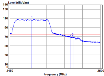
11ax_20M_TX_CH_11_Horizontal-Peak
