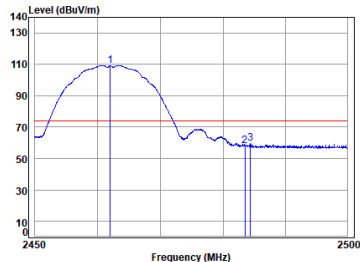
11b_TX_CH_11_Vertical-Peak
