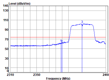
11n_HT(40M)_TX_CH_03_Vertical-Peak
