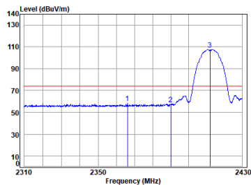
11b_TX_CH_01_Vertical-Peak
