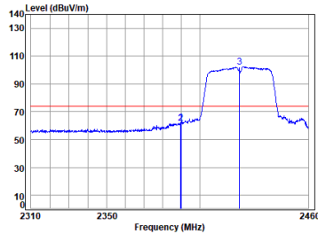
11n_HT(40M)_TX_CH_03_Horizontal-Peak
