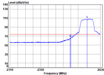
11g_TX_CH_01_Horizontal-Peak
