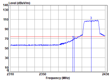
11ax_20M_TX_CH_01_Vertical-Peak
