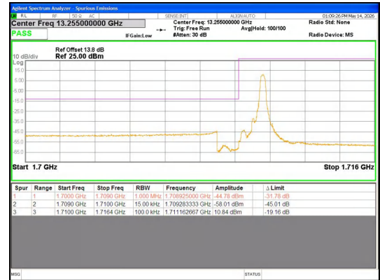
Band 4 1.4MHz/1710.7/Low QPSK 1@5
