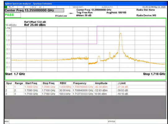
Band 4 3MHz/1711.5/Low QPSK 1@14
