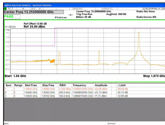
Band 2 20MHz/1860.0/Low QPSK 1@99
