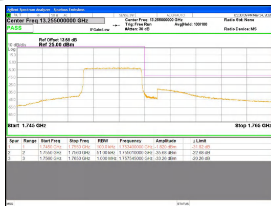
Band 4 5MHz/1752.5/High 16QAM 1@0
