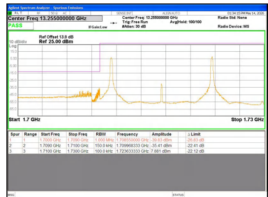
Band 4 15MHz/1717.5/Low 16QAM 1@0
