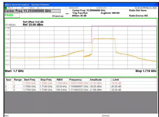
Band 4 3MHz/1711.5/Low 16QAM 1@0
