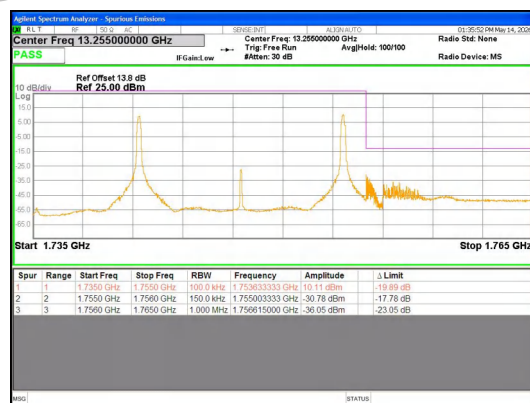
Band 4 15MHz/1747.5/High 16QAM 1@0
