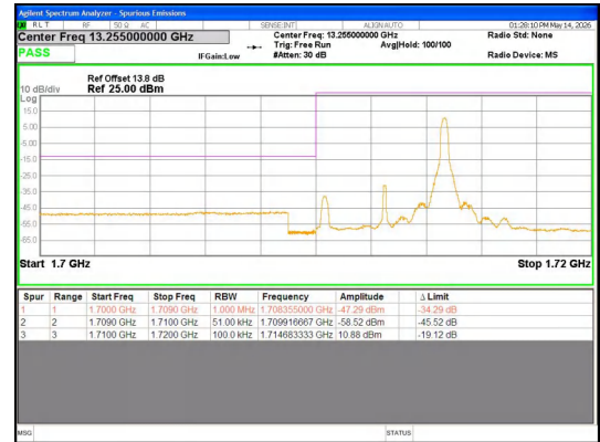
Band 4 5MHz/1712.5/Low QPSK 1@24
