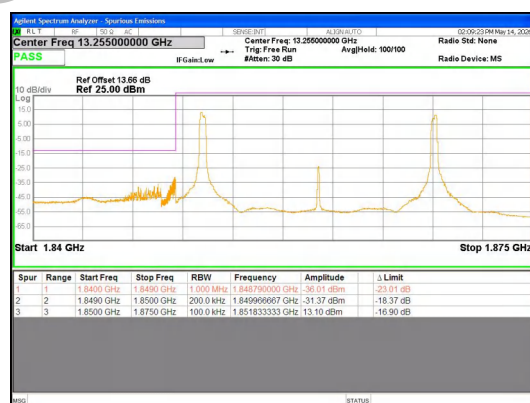
Band 2 20MHz/1860.0/Low 16QAM 1@0
