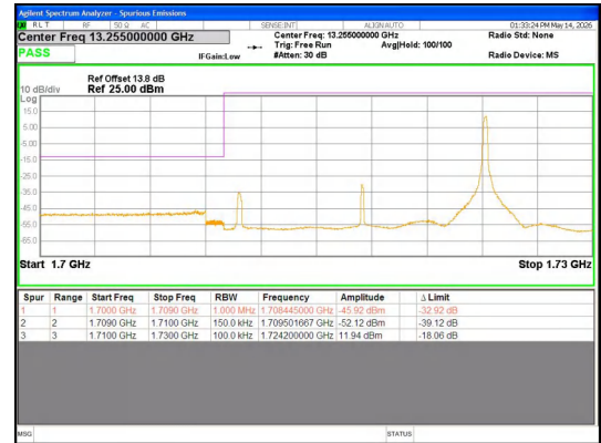
Band 4 15MHz/1717.5/Low QPSK 1@74
