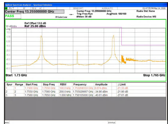
Band 4 20MHz/1745.0/High 16QAM 1@0
