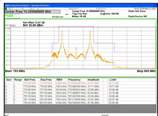
Band 13 10MHz/782.0/High 16QAM 1@0
