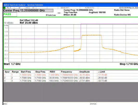
Band 66 3MHz/1711.5/Low 16QAM 1@0
