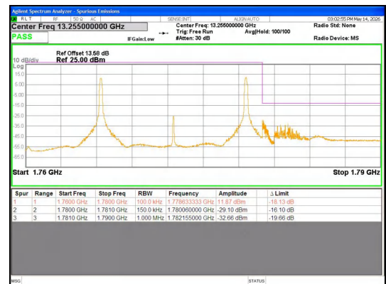
Band 66 15MHz/1772.5/High 16QAM 1@0
