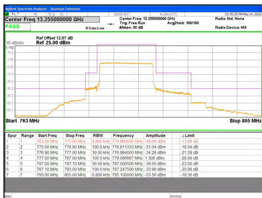
Band 13 10MHz/782.0/High QPSK 1@0
