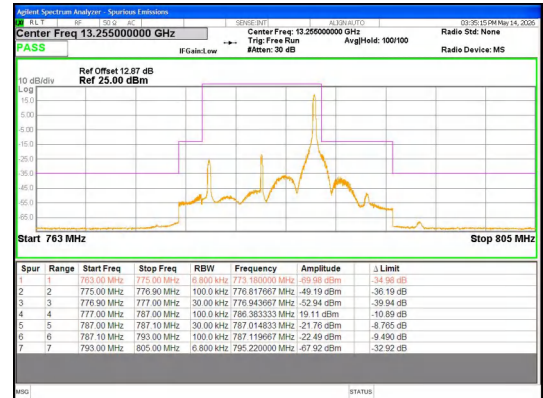
Band 13 10MHz/782.0/High QPSK 1@49
