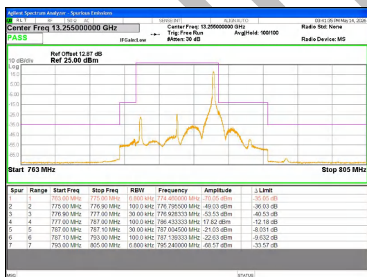
Band 13 10MHz/782.0/High QPSK 50@0
