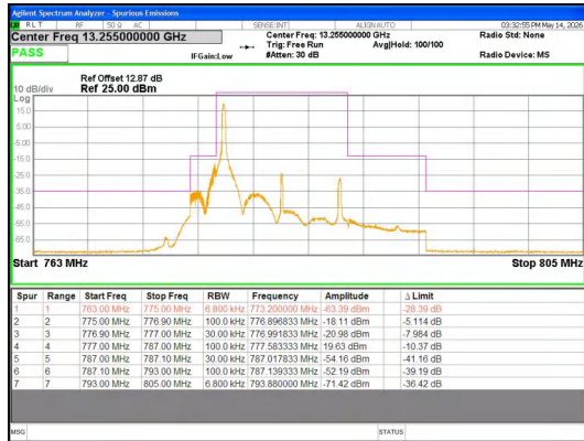
Band 13 10MHz/782.0/Low QPSK 1@0
