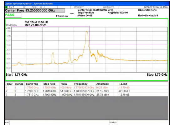
Band 66 5MHz/1777.5/High QPSK 1@24
