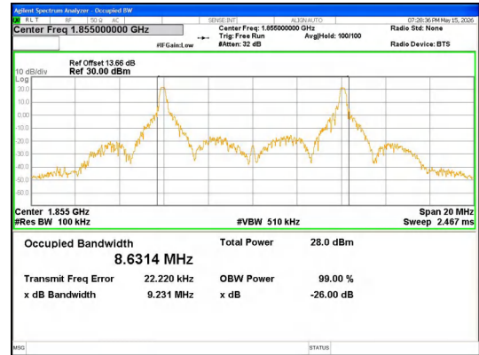
Band 2 10MHz/1855.0/Low 16QAM 50@0
