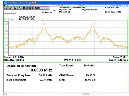
Band 4 10MHz/1715.0/Low 16QAM 50@0
