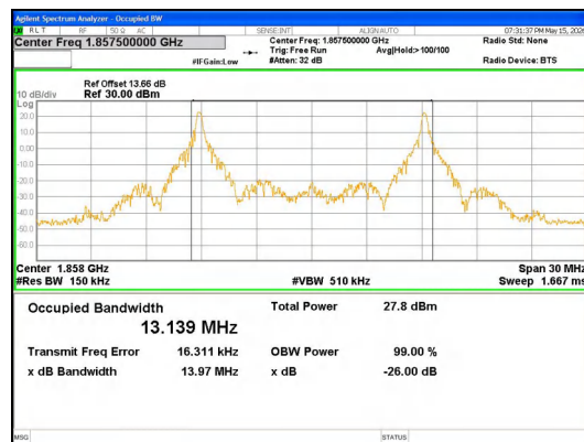
Band 2 15MHz/1857.5/Low 16QAM 75@0
