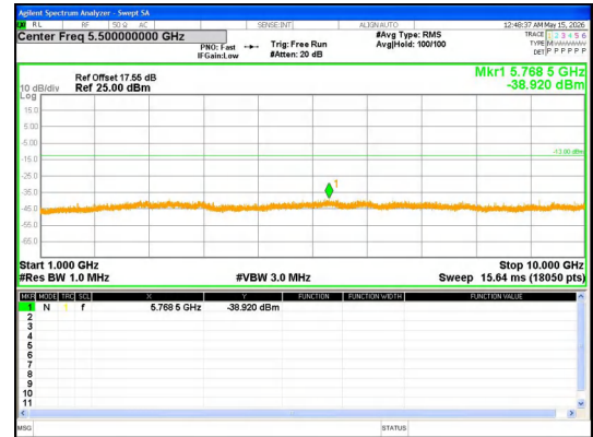
1000.0MHz-10000.0MHz Band 5 1.4MHz/836.5/Mid 16QAM 1@0
