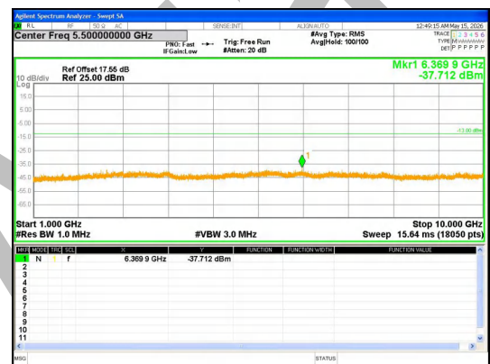
1000.0MHz-10000.0MHz Band 5 1.4MHz/848.3/High QPSK 1@0
