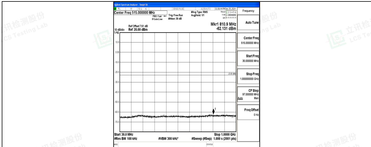
Band2_5MHz_16QAM_18625_1RB#0_30~1000_30~1000
