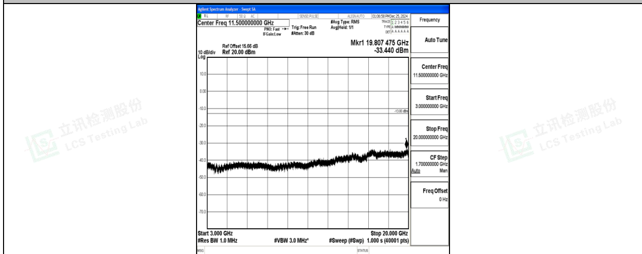
Band2_5MHz_16QAM_18625_1RB#0_3000~20000_3000~20000
