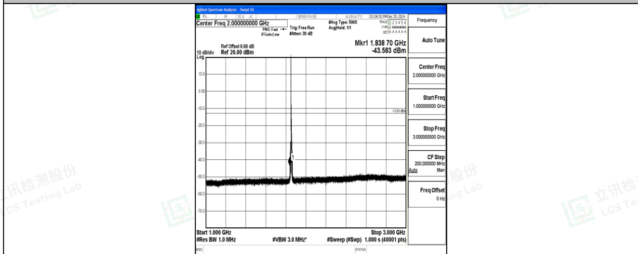
Band2_5MHz_16QAM_18625_1RB#0_1000~3000_1000~3000
