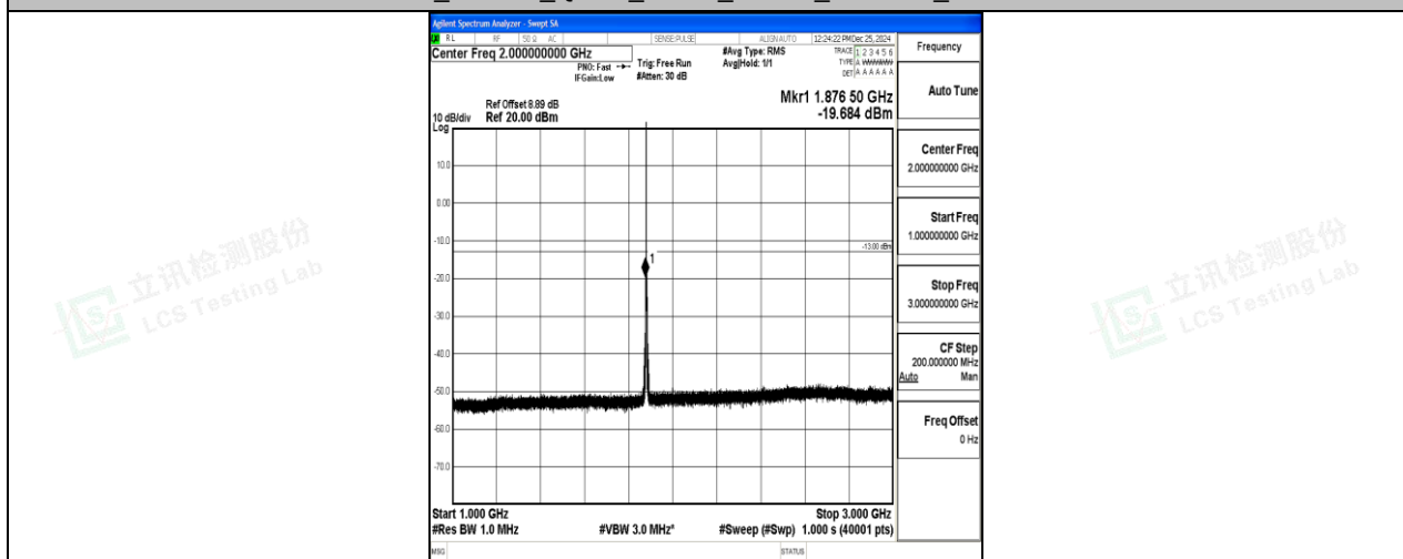
Band2_1.4MHz_QPSK_18900_1RB#0_1000~3000_1000~3000
