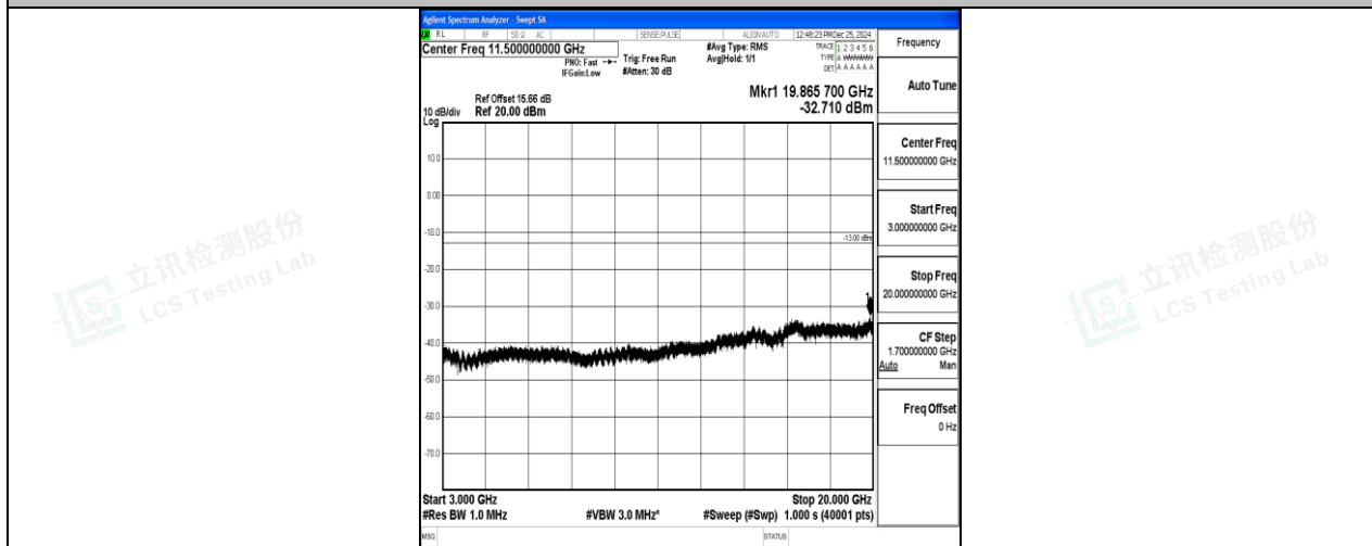
Band2_3MHz_16QAM_18615_1RB#0_3000~20000_3000~20000
