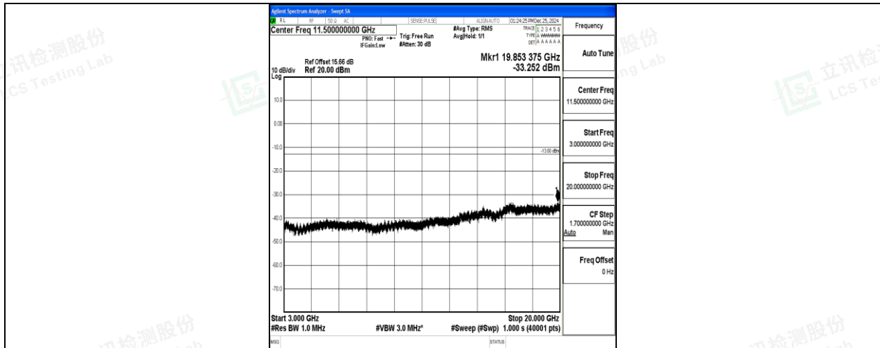
Band2_10MHz_QPSK_18650_1RB#0_3000~20000_3000~20000
