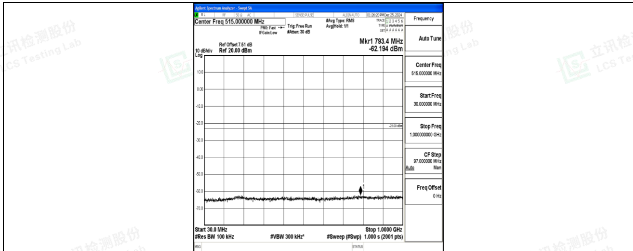
Band2_10MHz_QPSK_19150_1RB#0_30~1000_30~1000
