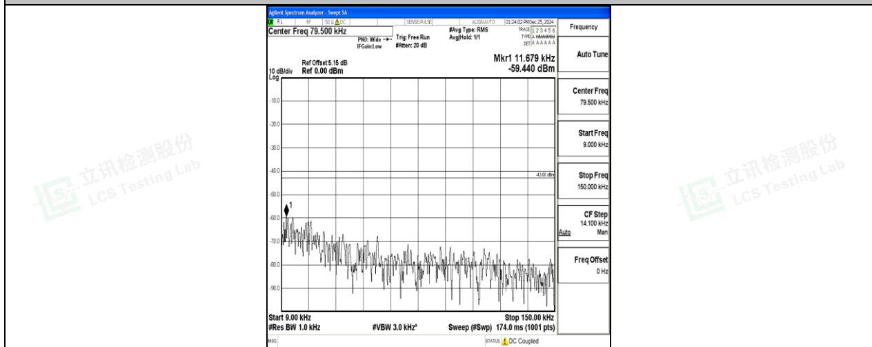
Band2_10MHz_QPSK_18650_1RB#0_0.009~0.15_0.009~0.15
