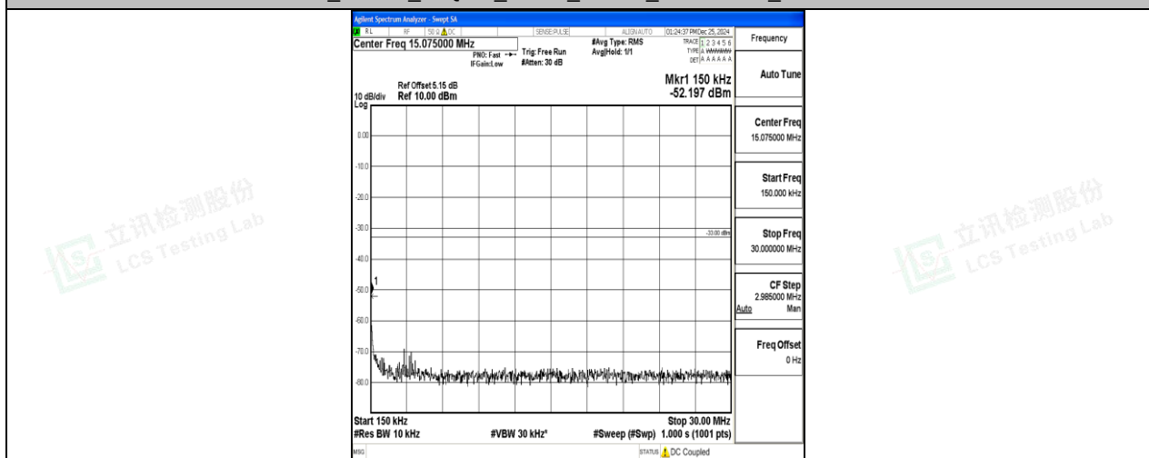
Band2_10MHz_16QAM_18650_1RB#0_0.15~30_0.15~30
