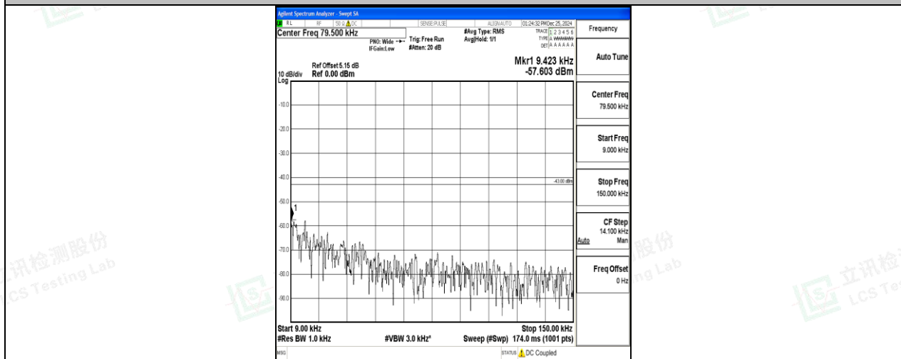
Band2_10MHz_16QAM_18650_1RB#0_0.009~0.15_0.009~0.15
