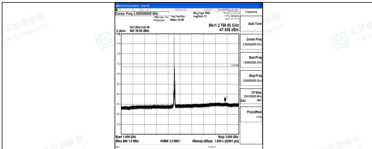
Band2_10MHz_16QAM_19150_1RB#0_1000~3000_1000~3000
