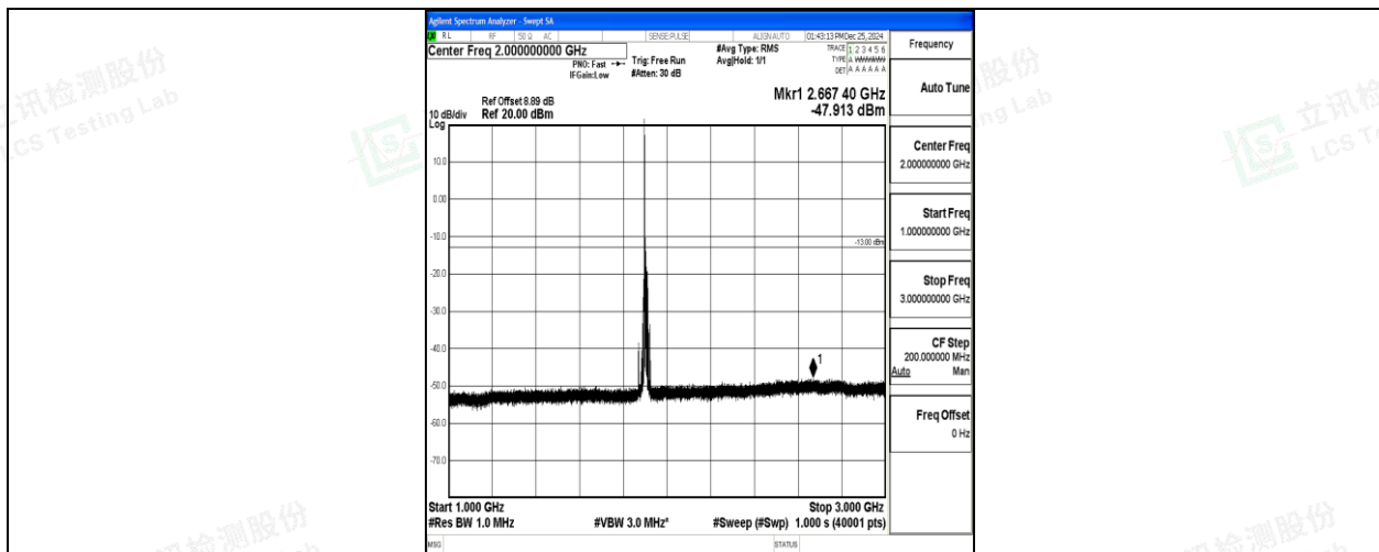
Band2_15MHz_16QAM_19125_1RB#0_1000~3000_1000~3000
