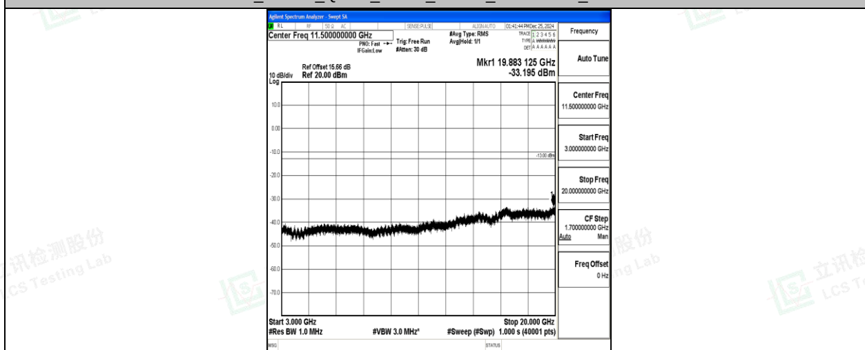
Band2_15MHz_QPSK_18900_1RB#0_3000~20000_3000~20000
