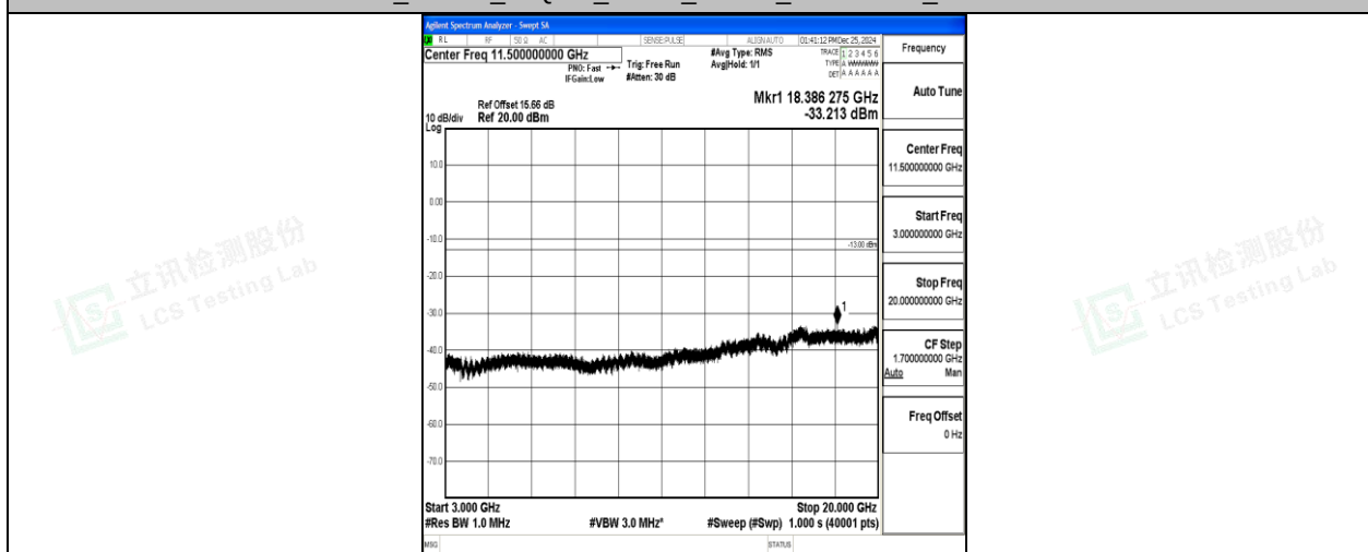
Band2_15MHz_16QAM_18675_1RB#0_3000~20000_3000~20000
