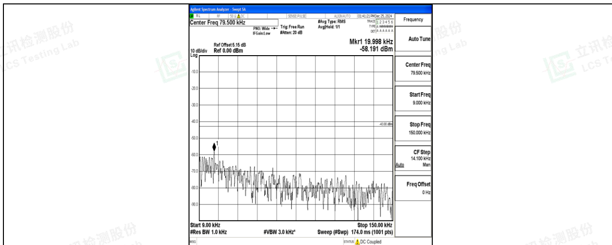
Band2_15MHz_QPSK_18900_1RB#0_0.009~0.15_0.009~0.15
