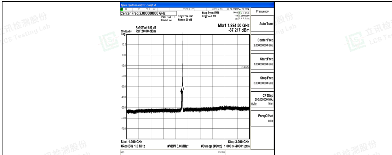
Band2_5MHz_16QAM_19175_1RB#0_1000~3000_1000~3000
