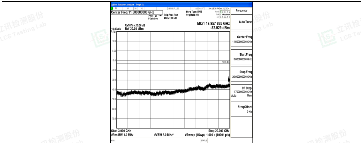
Band2_20MHz_16QAM_18900_1RB#0_3000~20000_3000~20000
