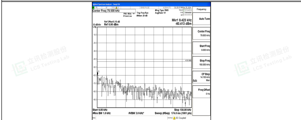
Band2_10MHz_16QAM_18900_1RB#0_0.009~0.15_0.009~0.15
