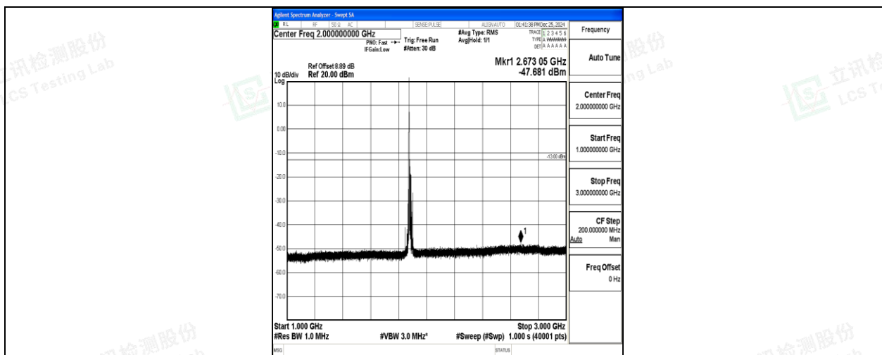
Band2_15MHz_QPSK_18900_1RB#0_1000~3000_1000~3000
