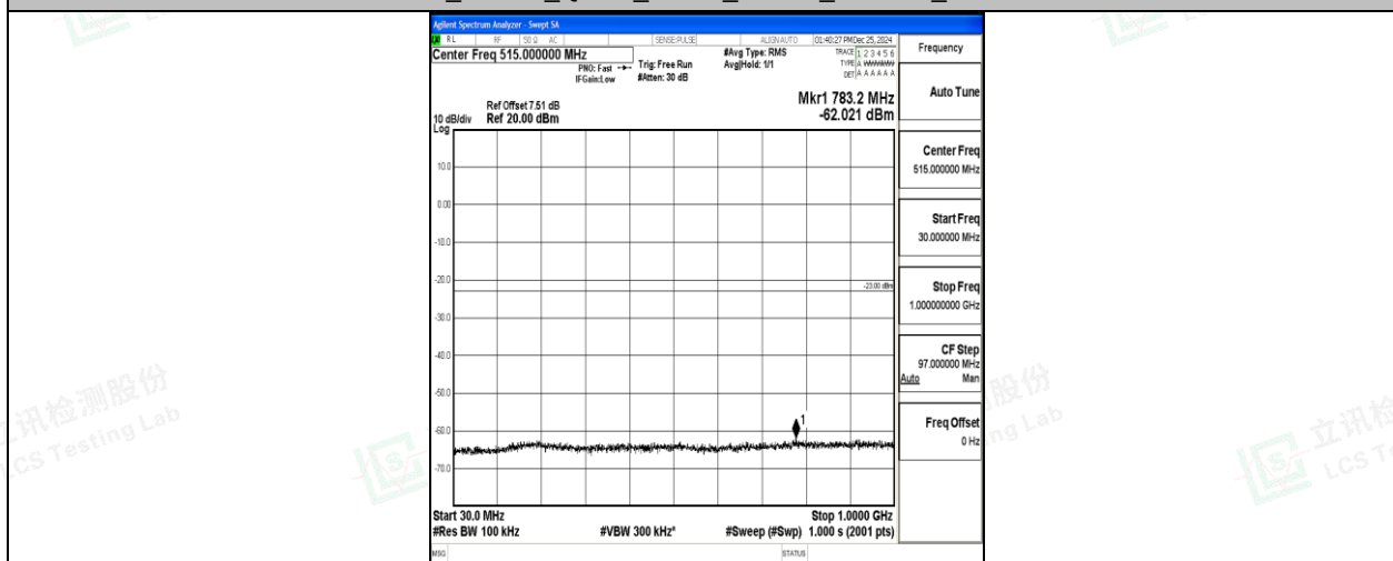
Band2_15MHz_QPSK_18675_1RB#0_30~1000_30~1000
