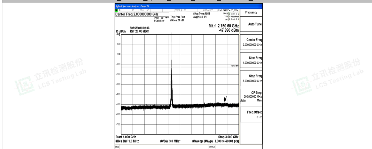
Band2_15MHz_QPSK_18675_1RB#0_1000~3000_1000~3000
