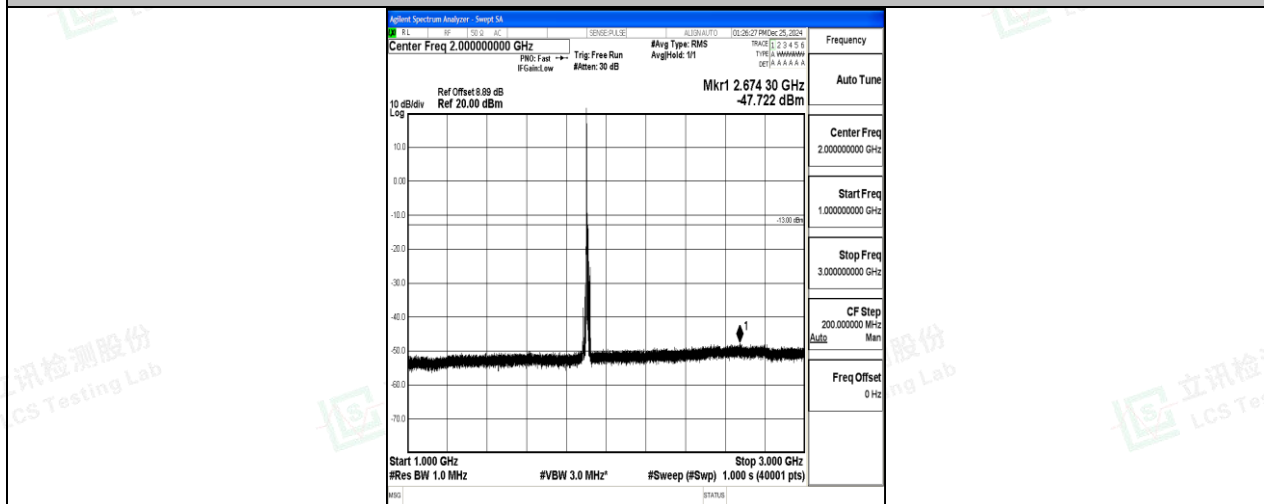
Band2_10MHz_QPSK_19150_1RB#0_1000~3000_1000~3000
