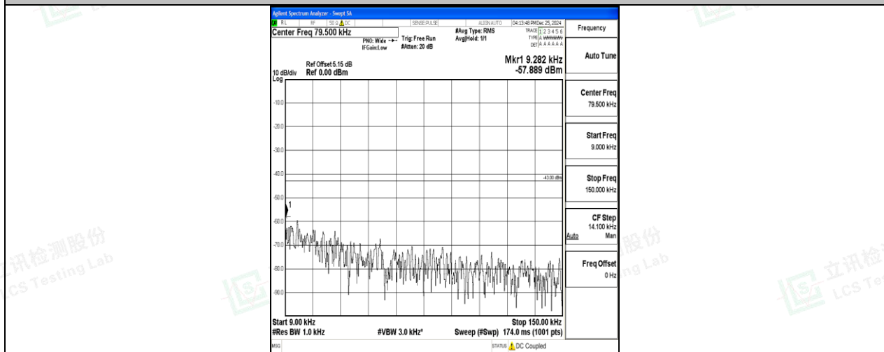
Band2_20MHz_QPSK_19100_1RB#0_0.009~0.15_0.009~0.15
