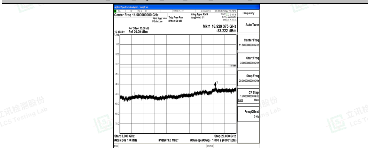
Band2_15MHz_16QAM_19125_1RB#0_3000~20000_3000~20000
