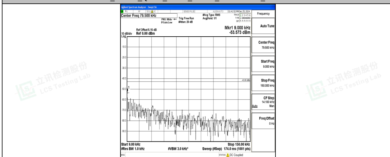
Band2_15MHz_16QAM_18900_1RB#0_0.009~0.15_0.009~0.15
