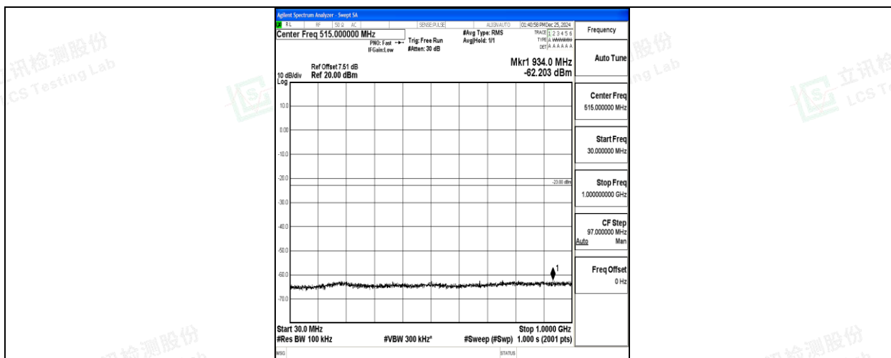
Band2_15MHz_16QAM_18675_1RB#0_30~1000_30~1000
