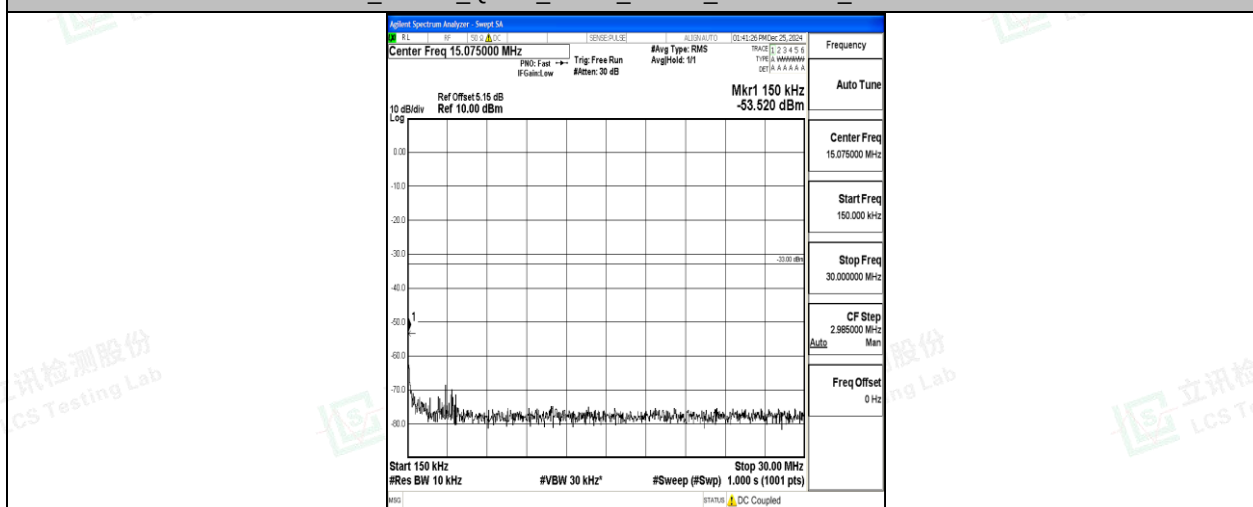
Band2_15MHz_QPSK_18900_1RB#0_0.15~30_0.15~30
