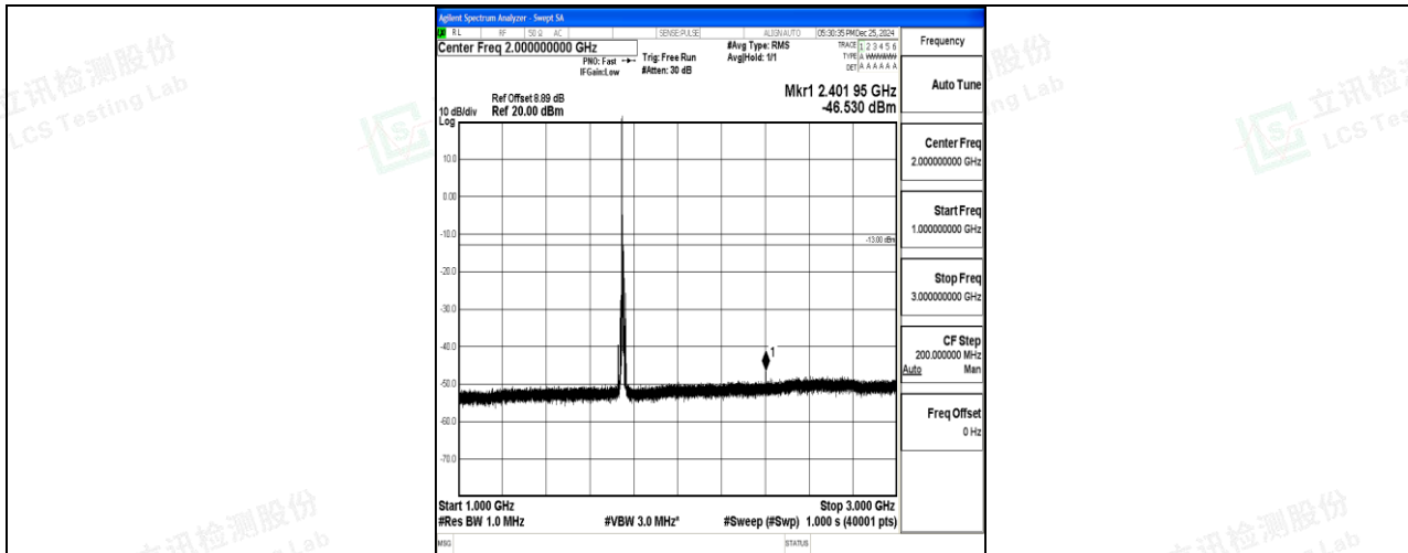
Band4_10MHz_16QAM_20350_1RB#0_1000~3000_1000~3000
