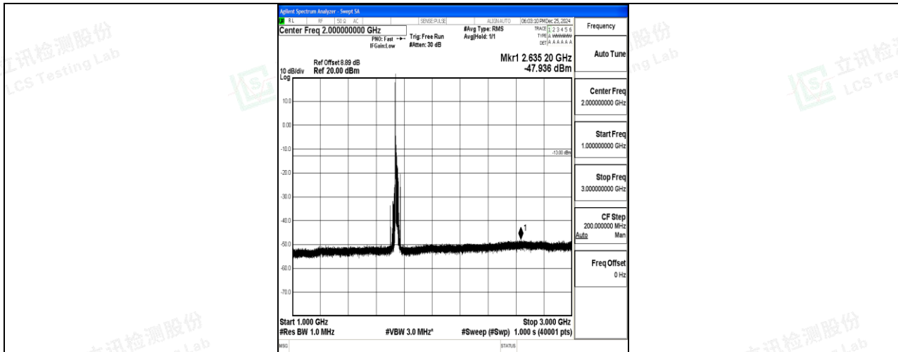
Band4_20MHz_16QAM_20300_1RB#0_1000~3000_1000~3000
