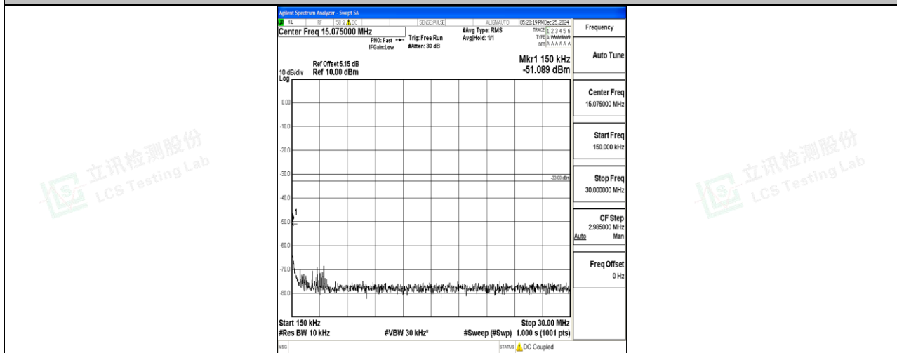
Band4_10MHz_16QAM_20000_1RB#0_0.15~30_0.15~30
