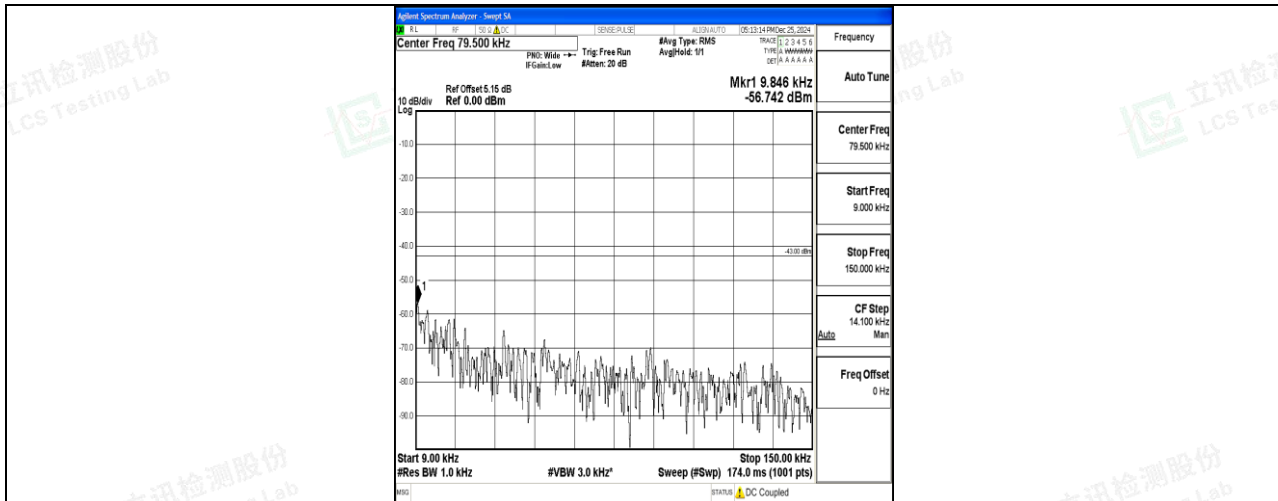
Band4_5MHz_16QAM_20375_1RB#0_0.009~0.15_0.009~0.15
