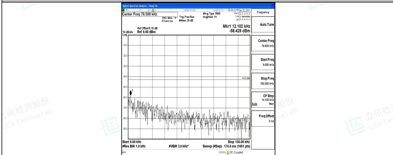
Band4_15MHz_QPSK_20325_1RB#0_0.009~0.15_0.009~0.15
