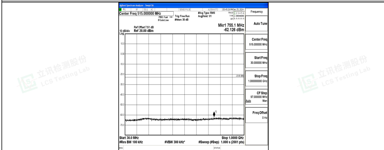
Band4_15MHz_QPSK_20175_1RB#0_30~1000_30~1000
