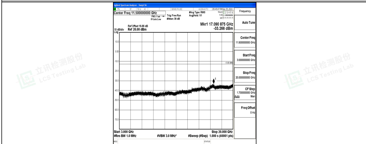
Band4_15MHz_16QAM_20025_1RB#0_3000~20000_3000~20000
