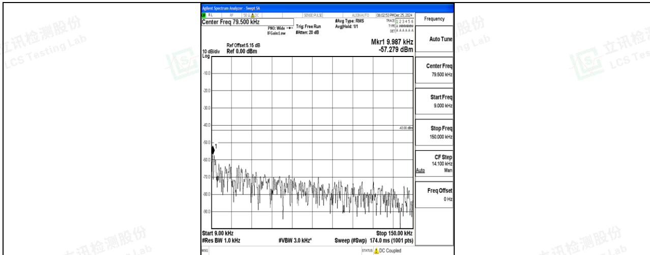
Band4_20MHz_16QAM_20300_1RB#0_0.009~0.15_0.009~0.15
