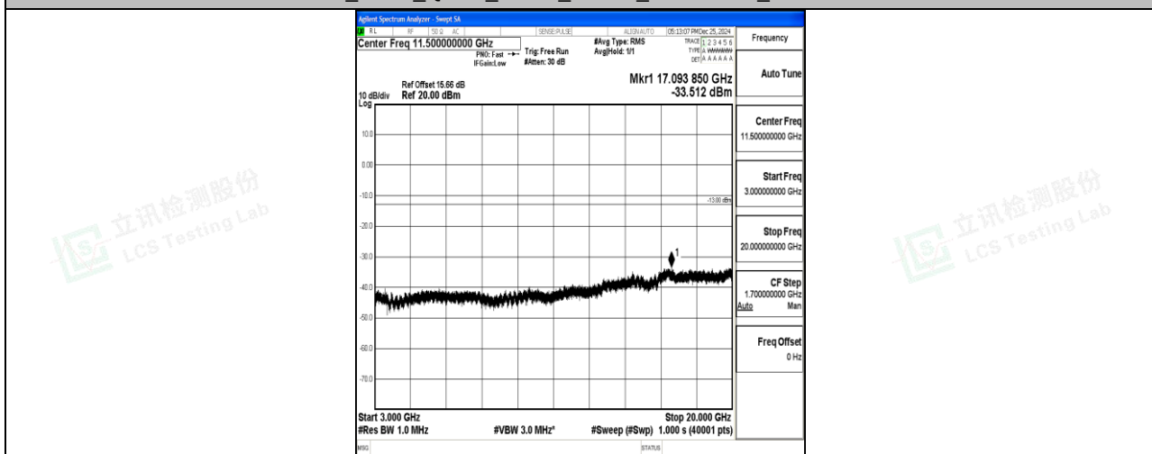
Band4_5MHz_QPSK_20375_1RB#0_3000~20000_3000~20000
