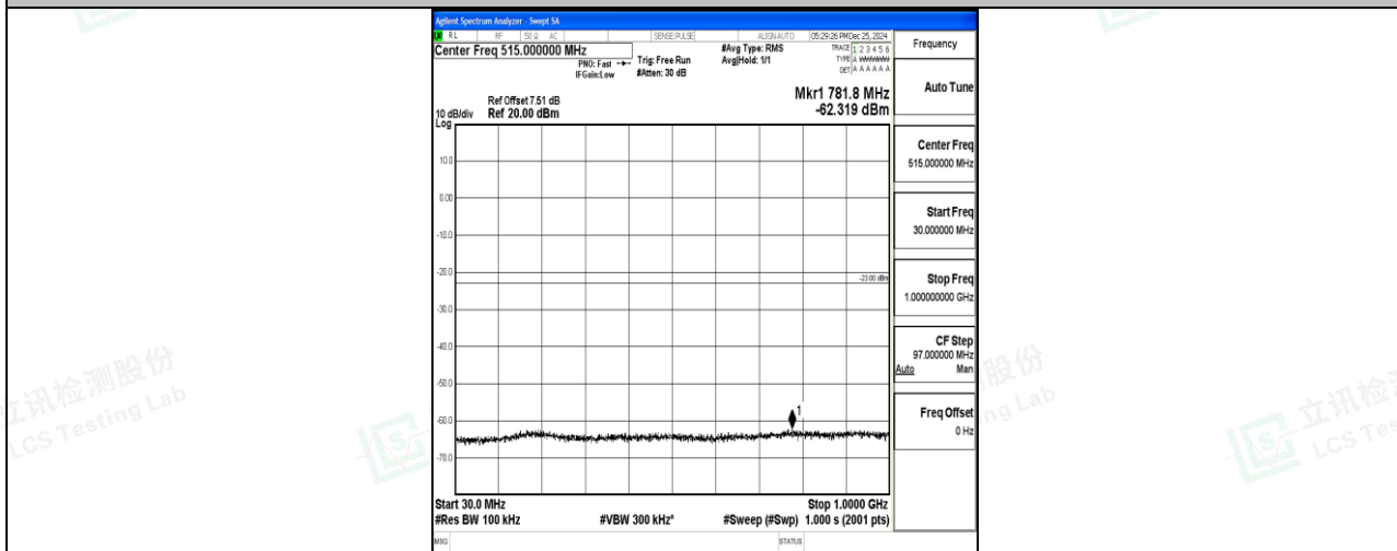
Band4_10MHz_16QAM_20175_1RB#0_30~1000_30~1000
