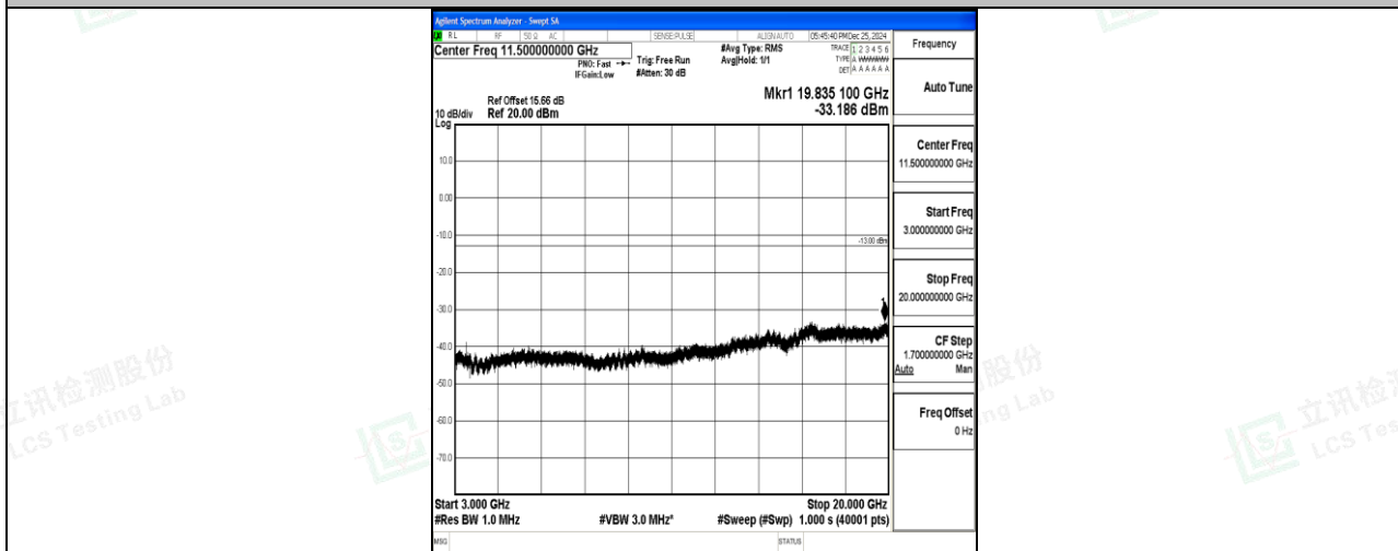
Band4_15MHz_QPSK_20175_1RB#0_3000~20000_3000~20000
