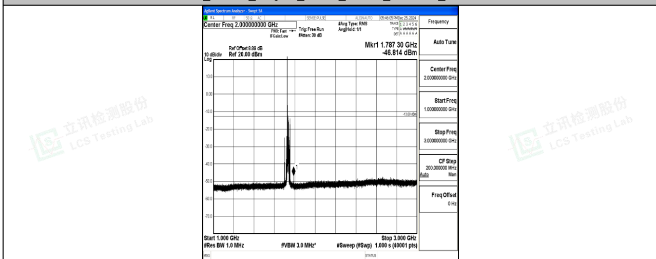
Band4_15MHz_16QAM_20175_1RB#0_1000~3000_1000~3000
