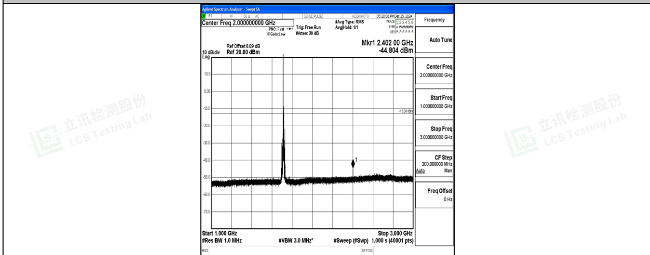
Band4_10MHz_QPSK_20000_1RB#0_1000~3000_1000~3000
