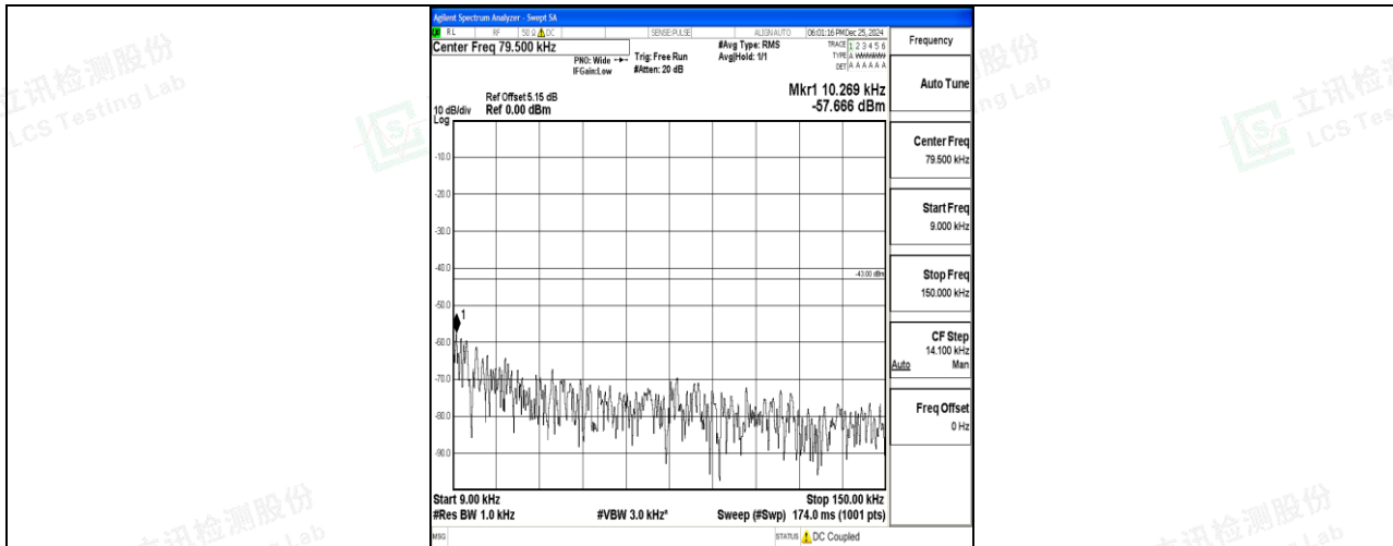
Band4_20MHz_QPSK_20175_1RB#0_0.009~0.15_0.009~0.15
