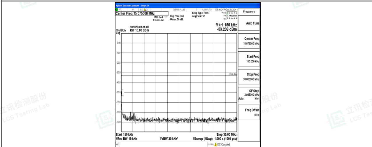
Band4_10MHz_16QAM_20350_1RB#0_0.15~30_0.15~30
