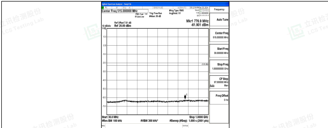
Band4_5MHz_QPSK_20375_1RB#0_30~1000_30~1000
