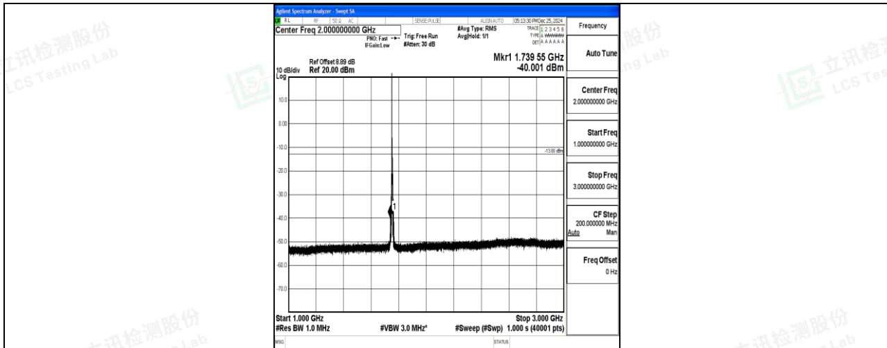
Band4_5MHz_16QAM_20375_1RB#0_1000~3000_1000~3000
