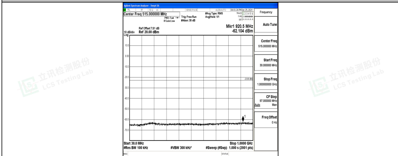
Band4_20MHz_QPSK_20175_1RB#0_30~1000_30~1000
