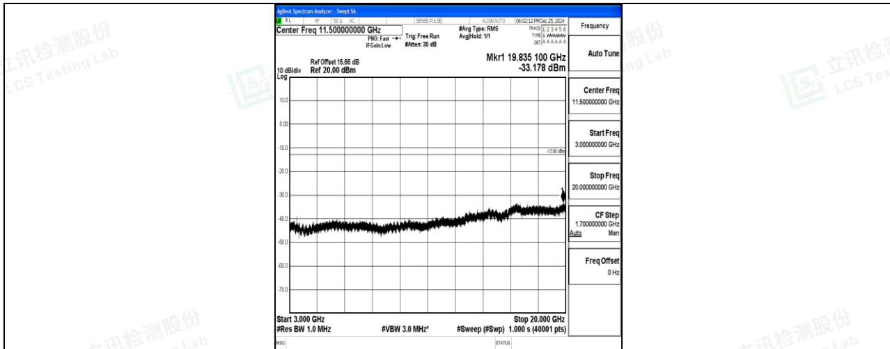
Band4_20MHz_16QAM_20175_1RB#0_3000~20000_3000~20000
