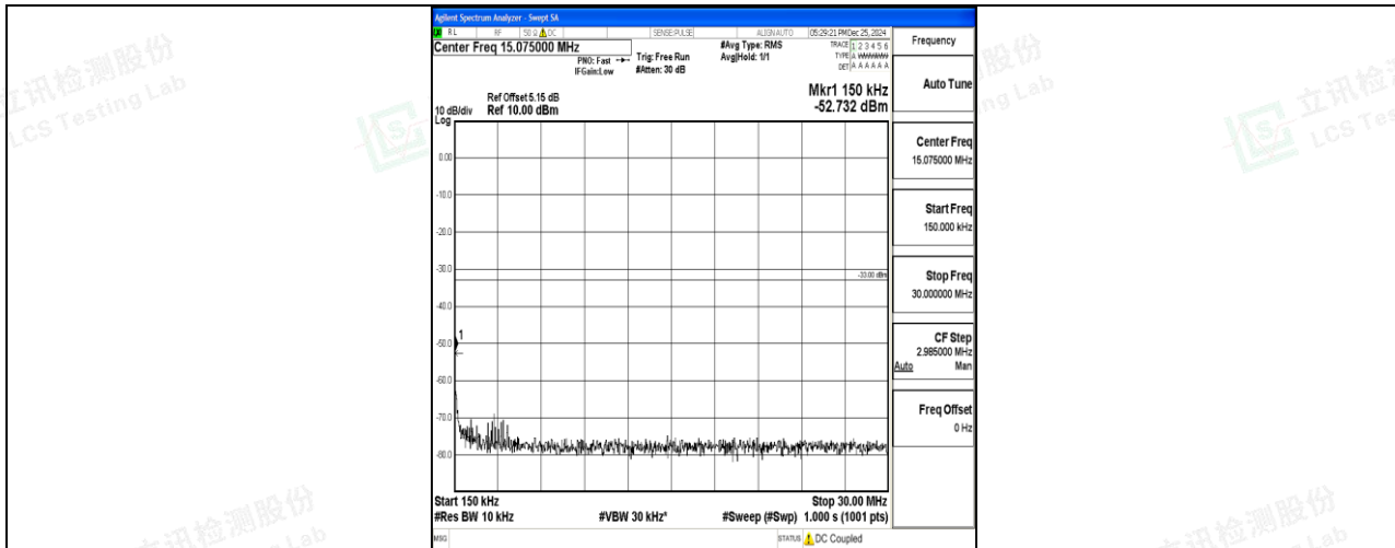
Band4_10MHz_16QAM_20175_1RB#0_0.15~30_0.15~30
