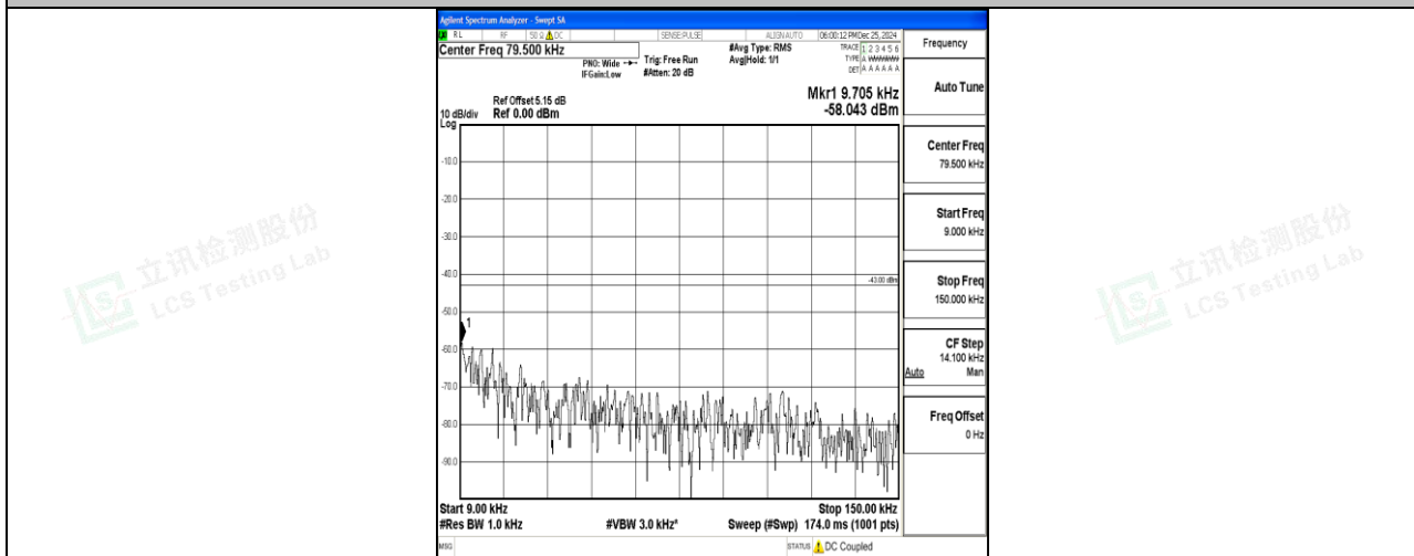
Band4_20MHz_QPSK_20050_1RB#0_0.009~0.15_0.009~0.15
