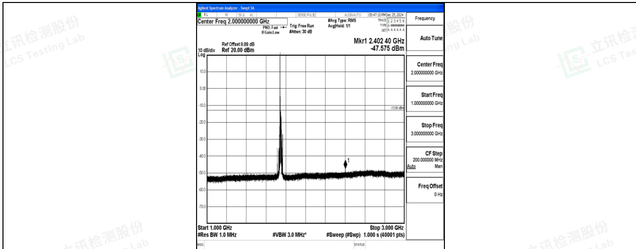
Band4_15MHz_16QAM_20325_1RB#0_1000~3000_1000~3000
