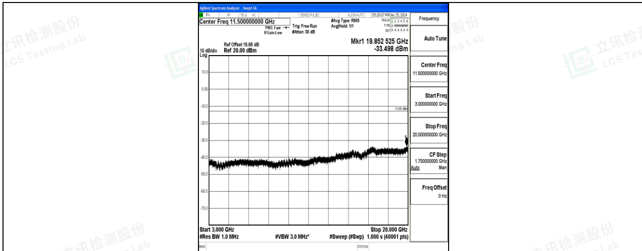
Band4_10MHz_QPSK_20000_1RB#0_3000~20000_3000~20000
