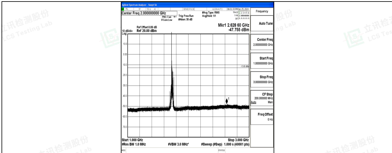
Band4_20MHz_QPSK_20175_1RB#0_1000~3000_1000~3000
