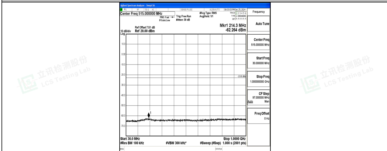
Band4_20MHz_16QAM_20300_1RB#0_30~1000_30~1000
