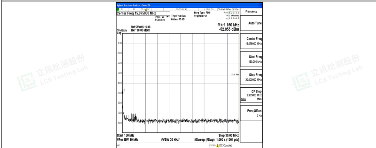
Band4_20MHz_16QAM_20050_1RB#0_0.15~30_0.15~30
