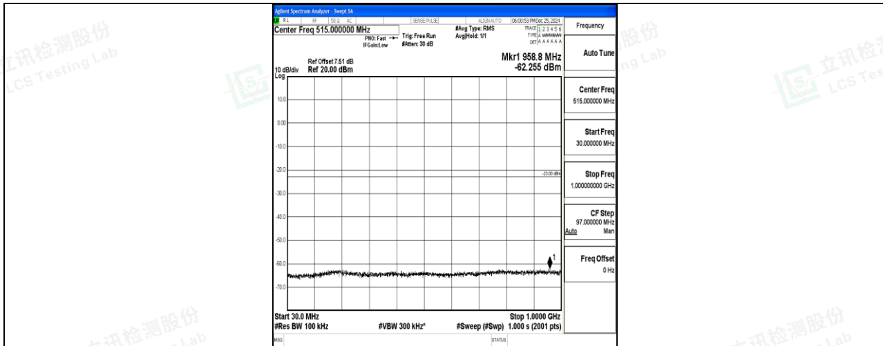
Band4_20MHz_16QAM_20050_1RB#0_30~1000_30~1000
