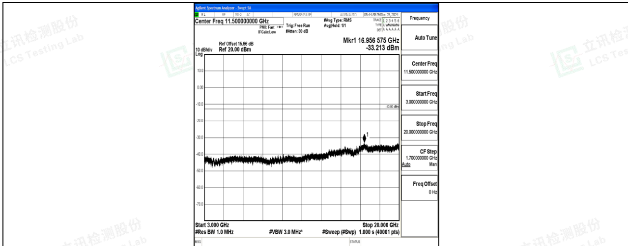
Band4_15MHz_QPSK_20025_1RB#0_3000~20000_3000~20000
