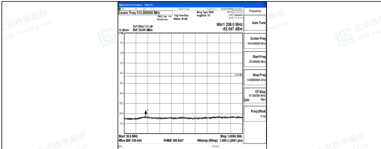
Band4_15MHz_16QAM_20025_1RB#0_30~1000_30~1000
