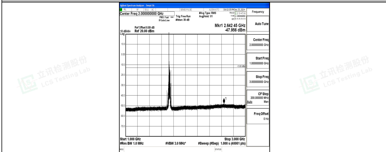
Band4_20MHz_16QAM_20175_1RB#0_1000~3000_1000~3000
