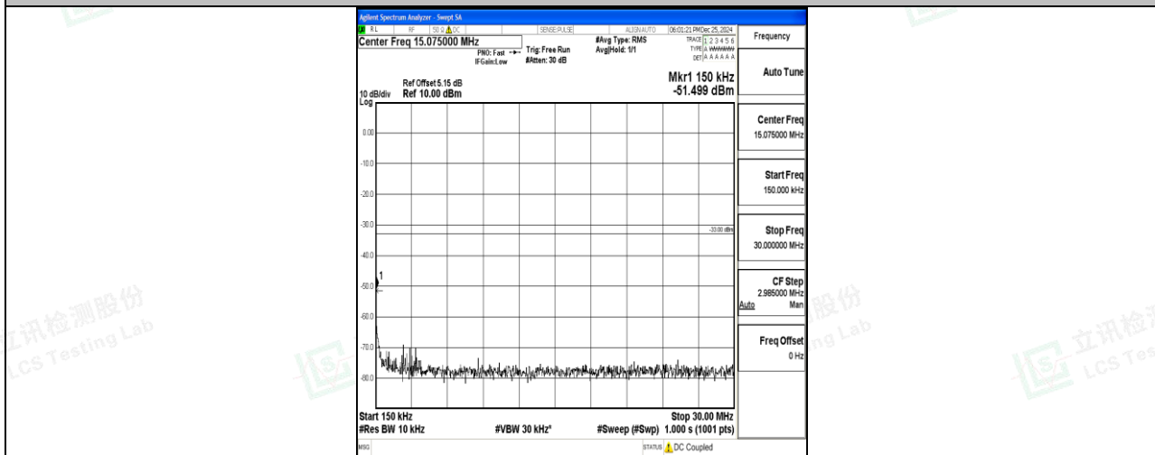
Band4_20MHz_QPSK_20175_1RB#0_0.15~30_0.15~30
