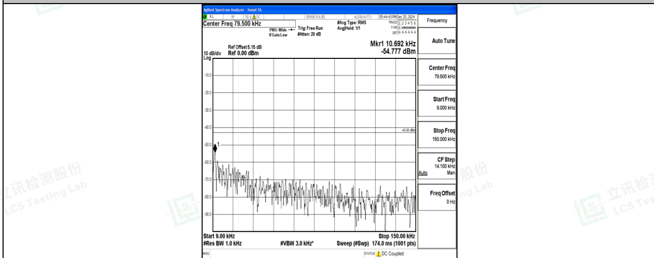
Band4_15MHz_16QAM_20025_1RB#0_0.009~0.15_0.009~0.15
