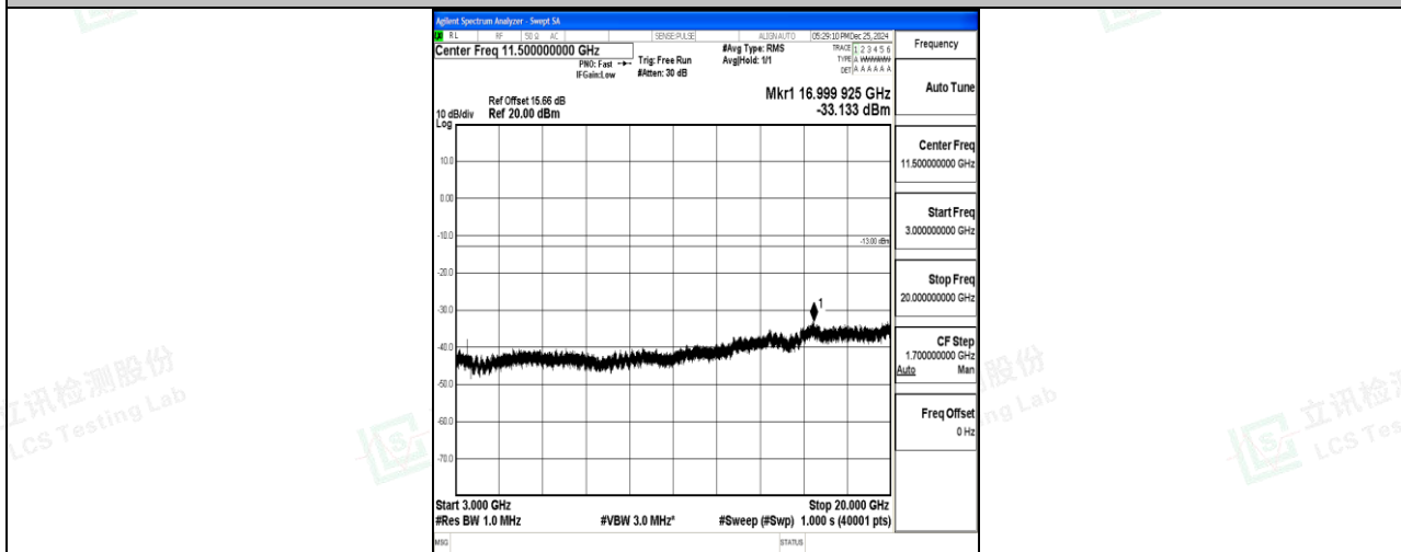
Band4_10MHz_QPSK_20175_1RB#0_3000~20000_3000~20000
