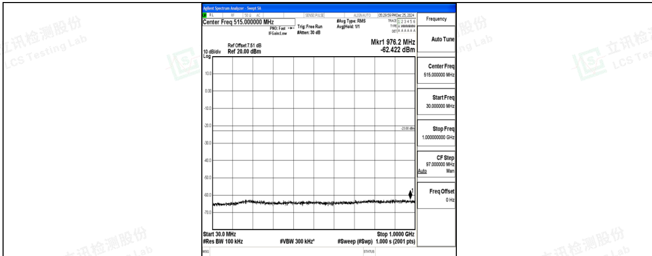
Band4_10MHz_QPSK_20350_1RB#0_30~1000_30~1000
