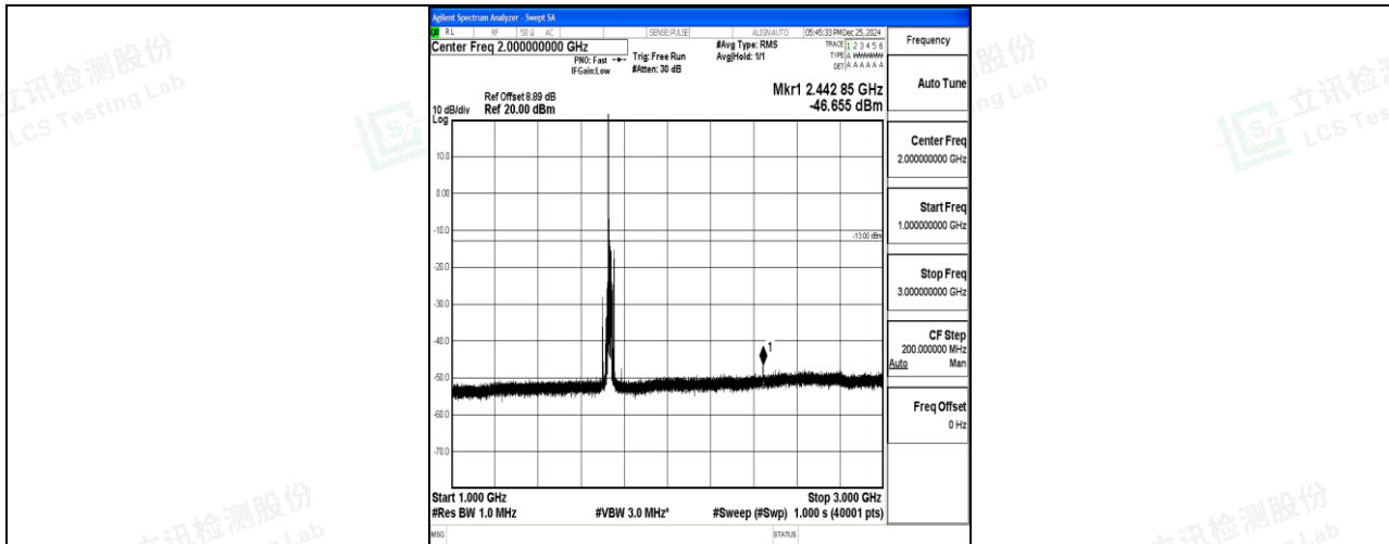
Band4_15MHz_QPSK_20175_1RB#0_1000~3000_1000~3000
