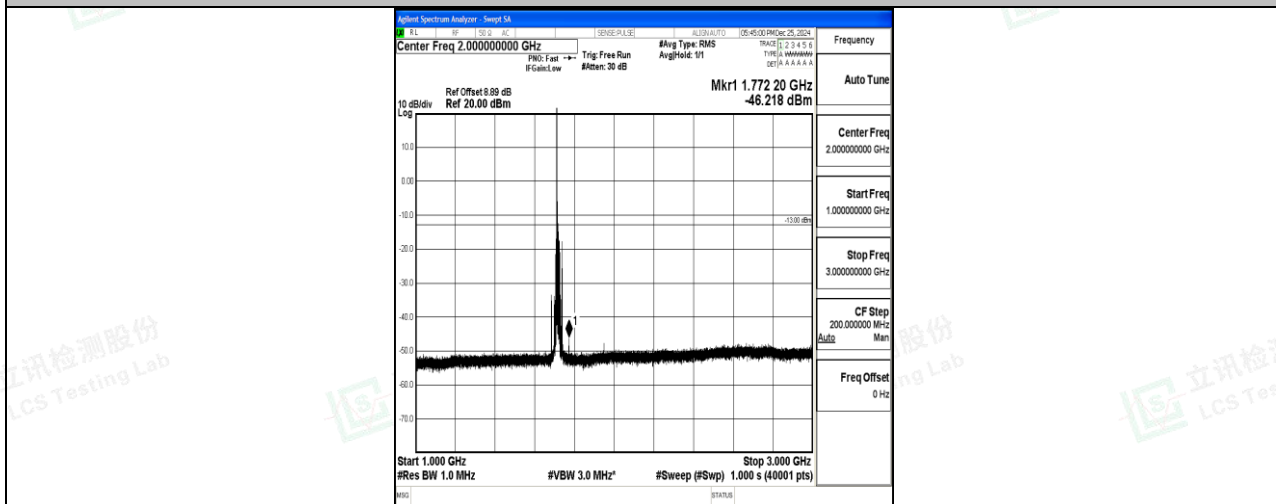
Band4_15MHz_16QAM_20025_1RB#0_1000~3000_1000~3000
