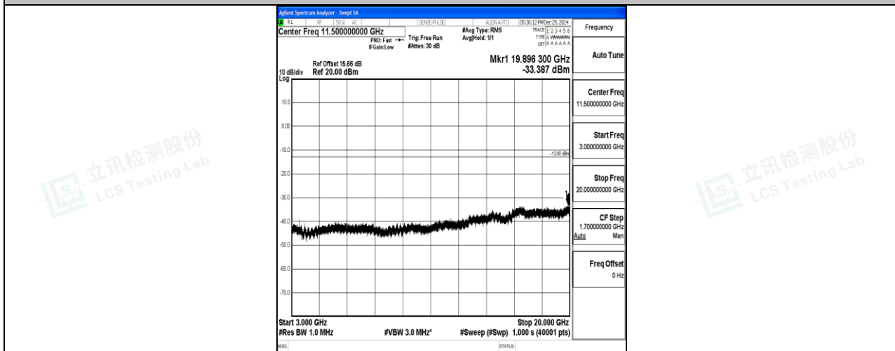
Band4_10MHz_QPSK_20350_1RB#0_3000~20000_3000~20000
