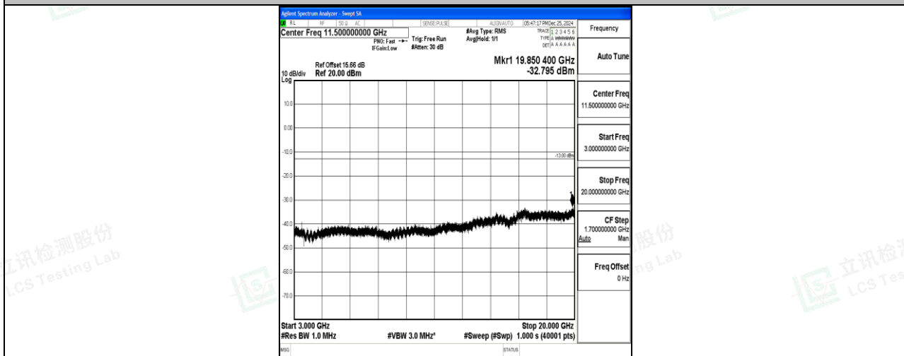
Band4_15MHz_16QAM_20325_1RB#0_3000~20000_3000~20000
