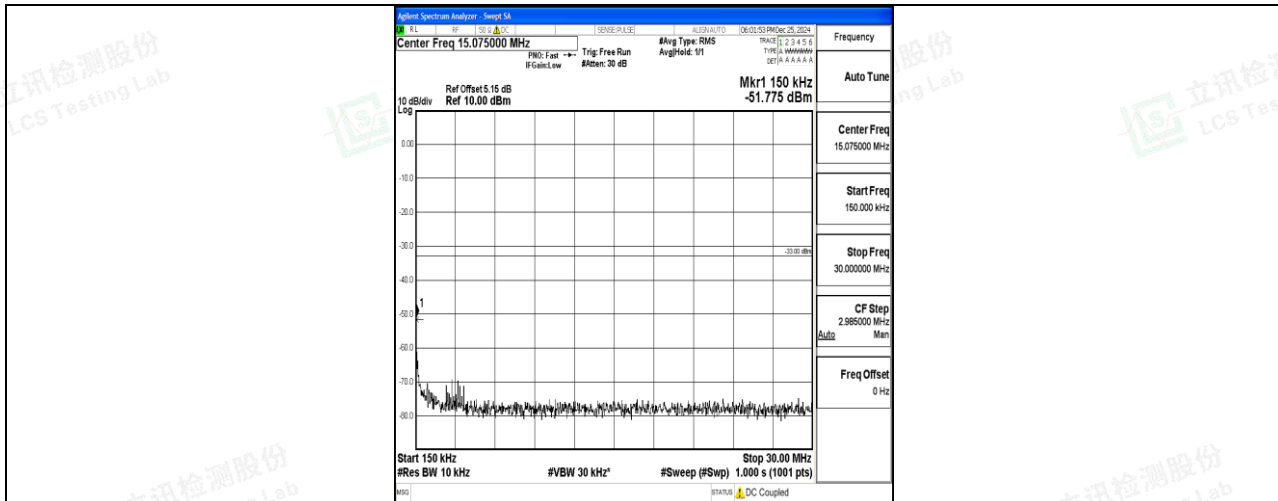
Band4_20MHz_16QAM_20175_1RB#0_0.15~30_0.15~30
