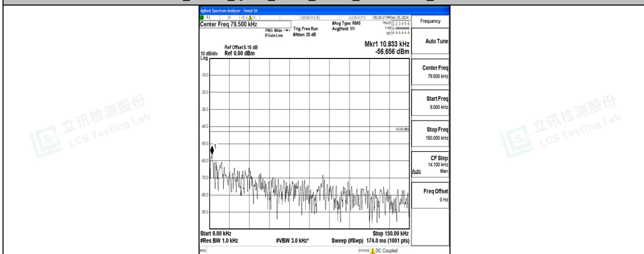
Band4_10MHz_16QAM_20175_1RB#0_0.009~0.15_0.009~0.15
