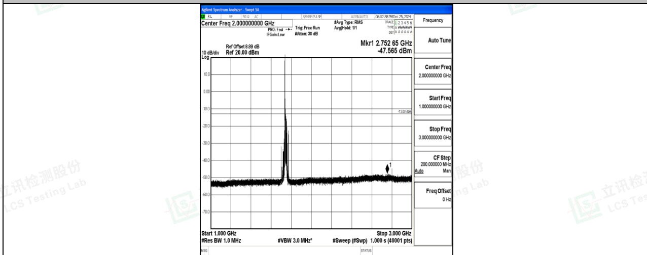
Band4_20MHz_QPSK_20300_1RB#0_1000~3000_1000~3000
