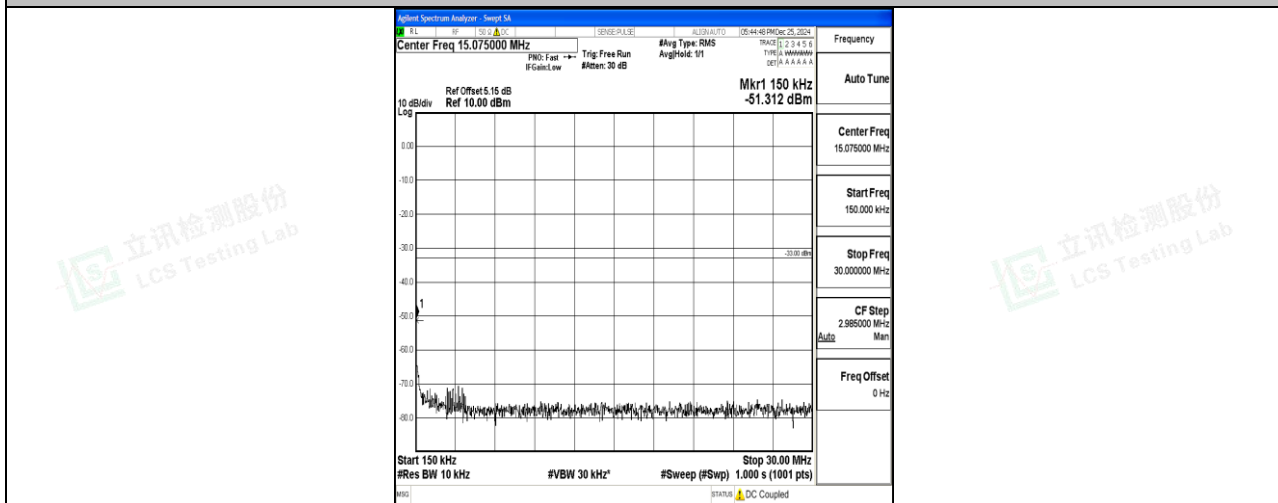
Band4_15MHz_16QAM_20025_1RB#0_0.15~30_0.15~30
