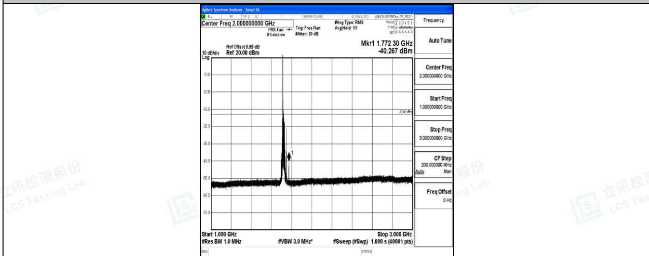
Band4_20MHz_16QAM_20050_1RB#0_1000~3000_1000~3000
