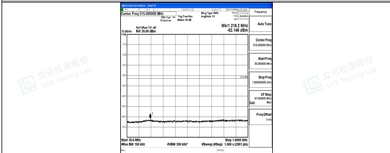
Band4_15MHz_16QAM_20325_1RB#0_30~1000_30~1000
