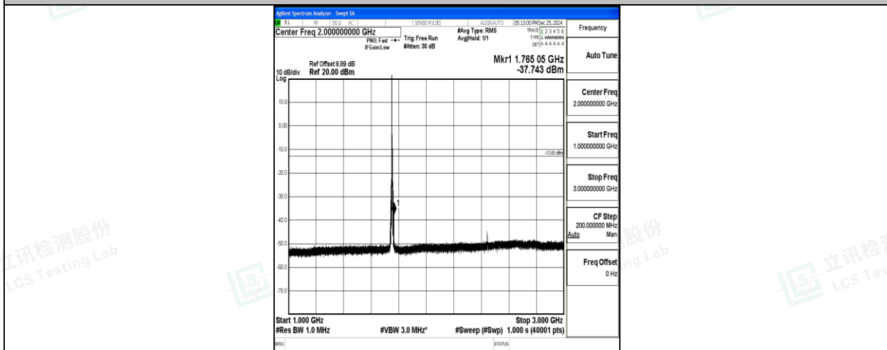
Band4_5MHz_QPSK_20375_1RB#0_1000~3000_1000~3000
