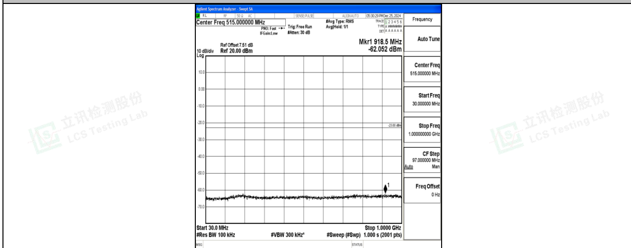
Band4_10MHz_16QAM_20350_1RB#0_30~1000_30~1000
