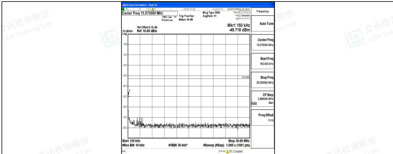
Band4_15MHz_16QAM_20175_1RB#0_0.15~30_0.15~30
