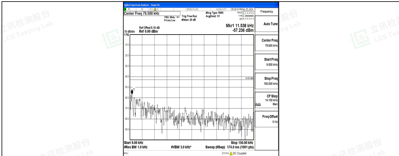
Band4_10MHz_QPSK_20175_1RB#0_0.009~0.15_0.009~0.15
