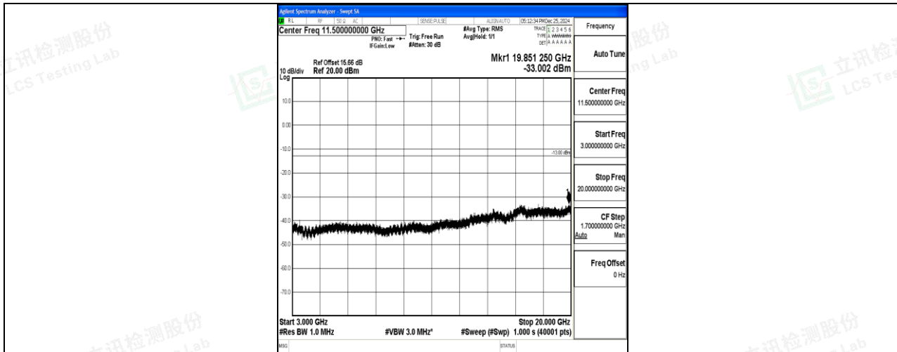
Band4_5MHz_16QAM_20175_1RB#0_3000~20000_3000~20000
