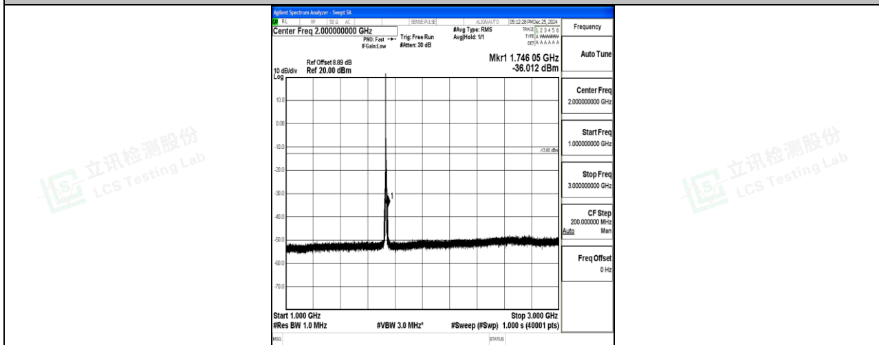
Band4_5MHz_16QAM_20175_1RB#0_1000~3000_1000~3000
