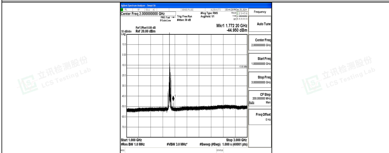
Band4_15MHz_QPSK_20025_1RB#0_1000~3000_1000~3000
