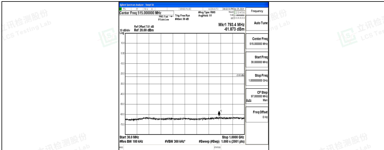
Band4_20MHz_QPSK_20300_1RB#0_30~1000_30~1000
