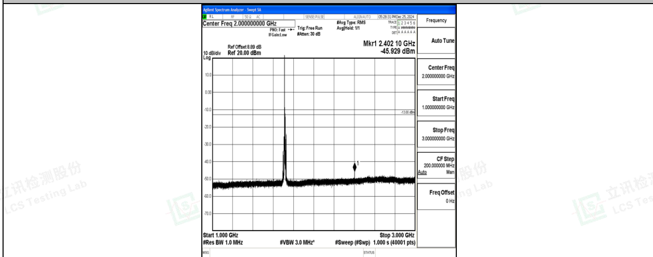
Band4_10MHz_16QAM_20000_1RB#0_1000-3000_1000-3000
