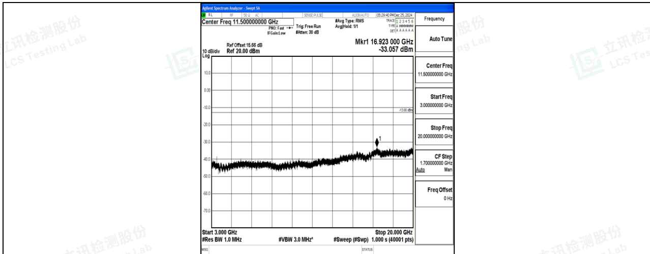
Band4_10MHz_16QAM_20175_1RB#0_3000~20000_3000~20000
