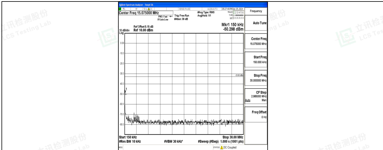
Band4_10MHz_QPSK_20000_1RB#0_0.15~30_0.15~30
