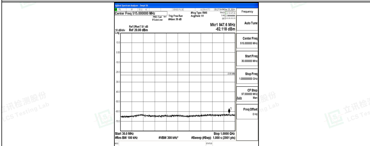
Band4_10MHz_QPSK_20000_1RB#0_30~1000_30~1000
