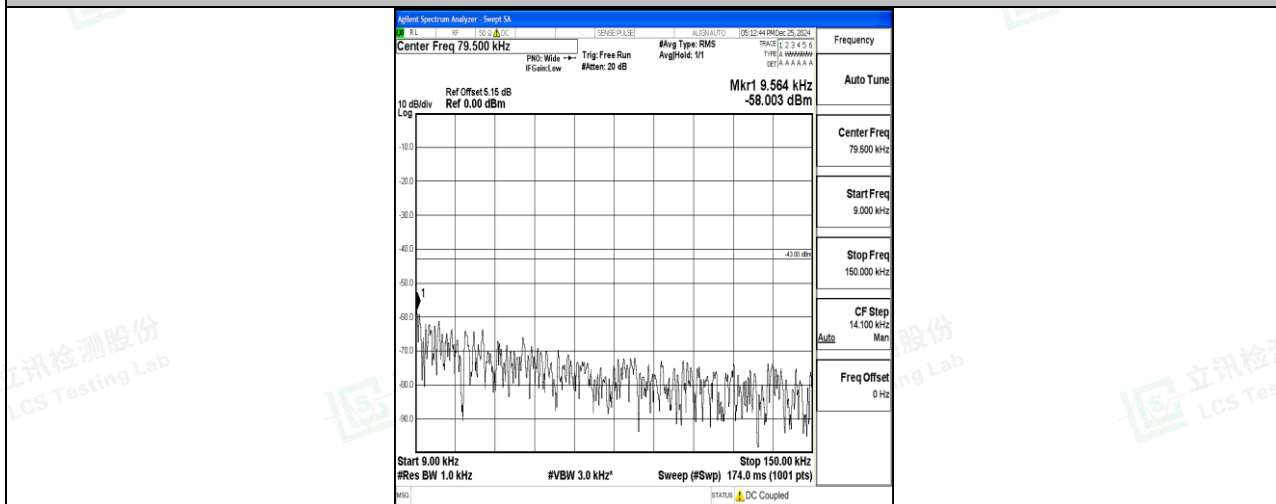
Band4_5MHz_QPSK_20375_1RB#0_0.009~0.15_0.009~0.15
