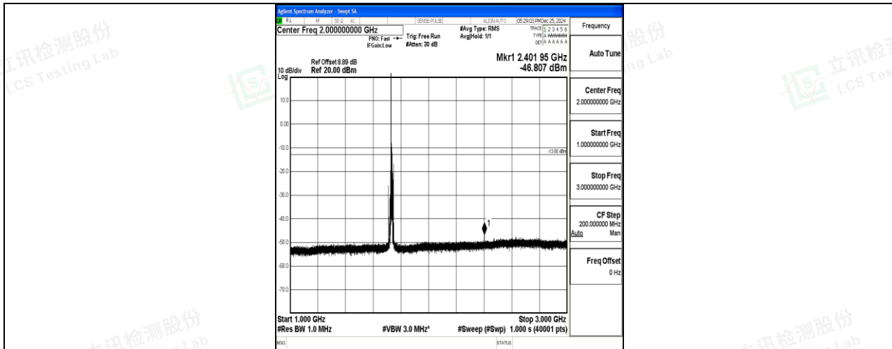
Band4_10MHz_QPSK_20175_1RB#0_1000~3000_1000~3000
