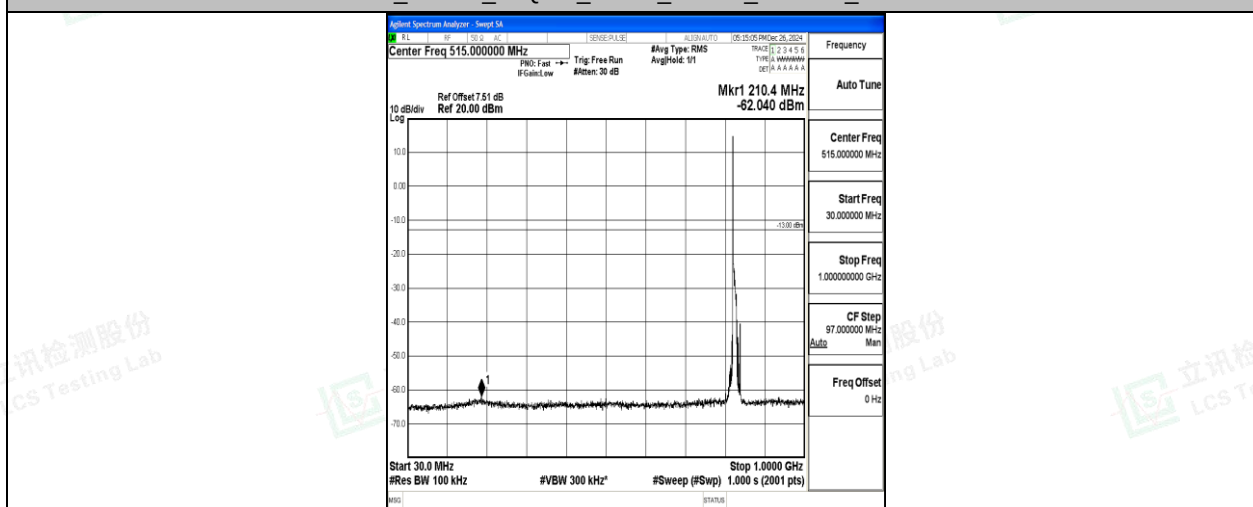
Band5_10MHz_16QAM_20450_1RB#0_30~1000_30~1000
