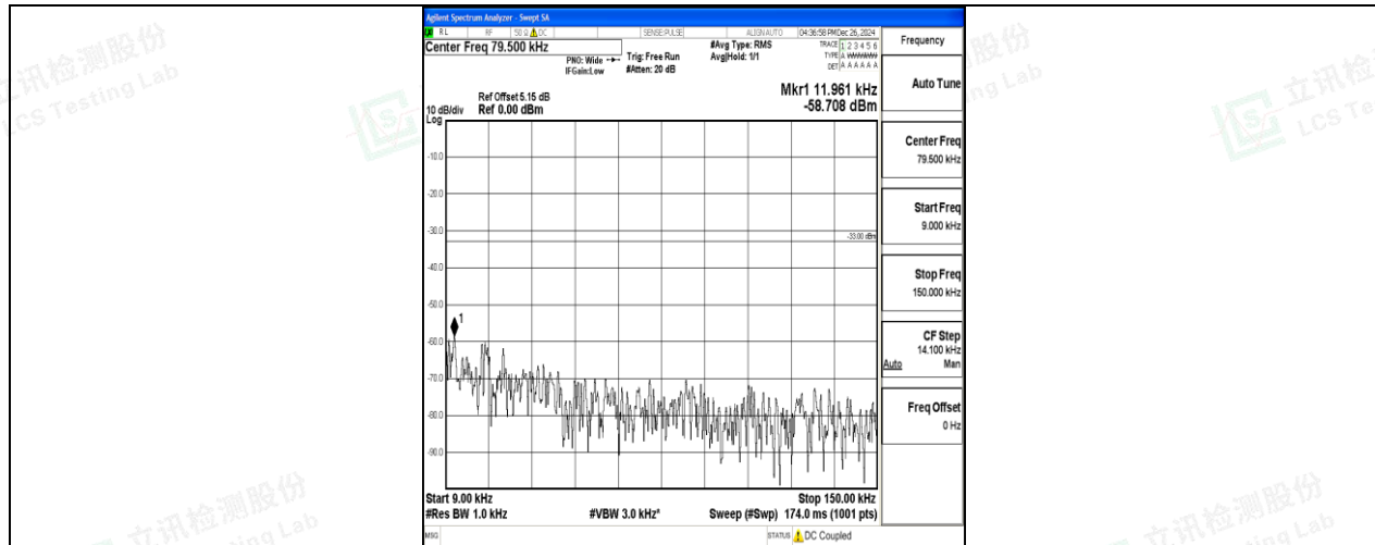
Band5_3MHz_16QAM_20525_1RB#0_0.009~0.15_0.009~0.15
