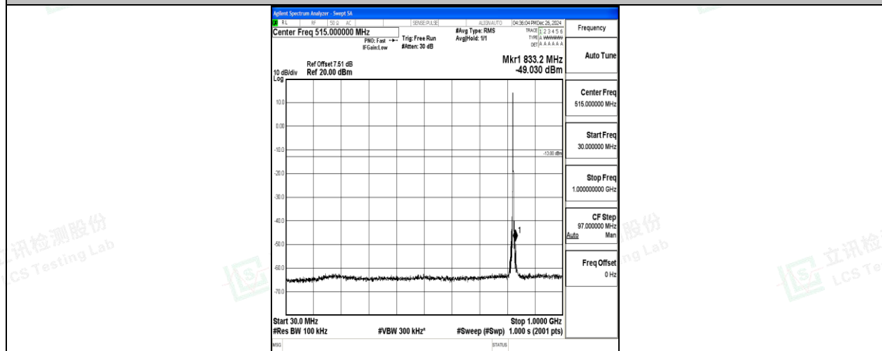
Band5_3MHz_16QAM_20415_1RB#0_30~1000_30~1000
