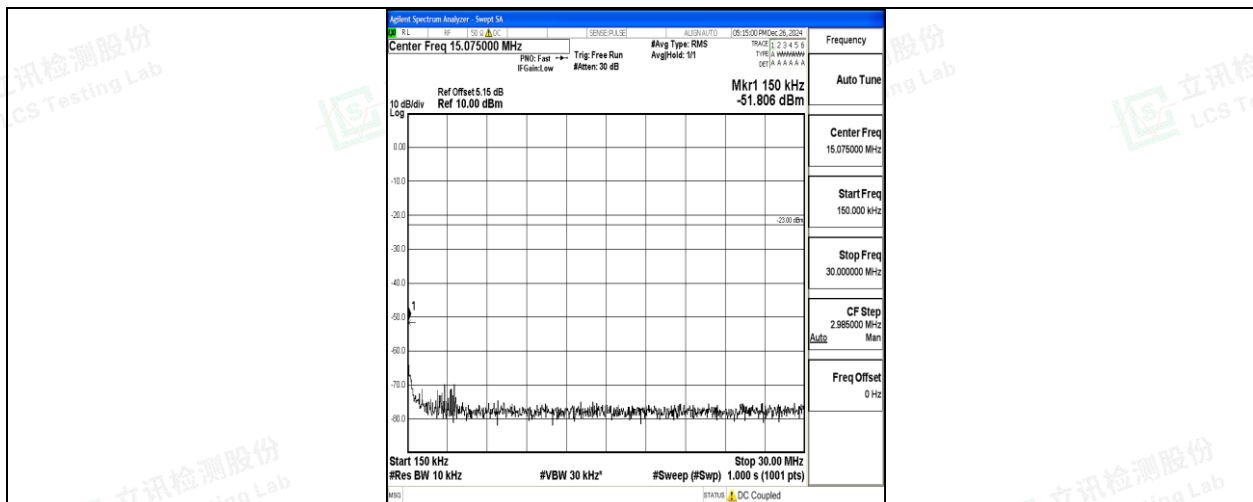
Band5_10MHz_16QAM_20450_1RB#0_0.15~30_0.15~30
