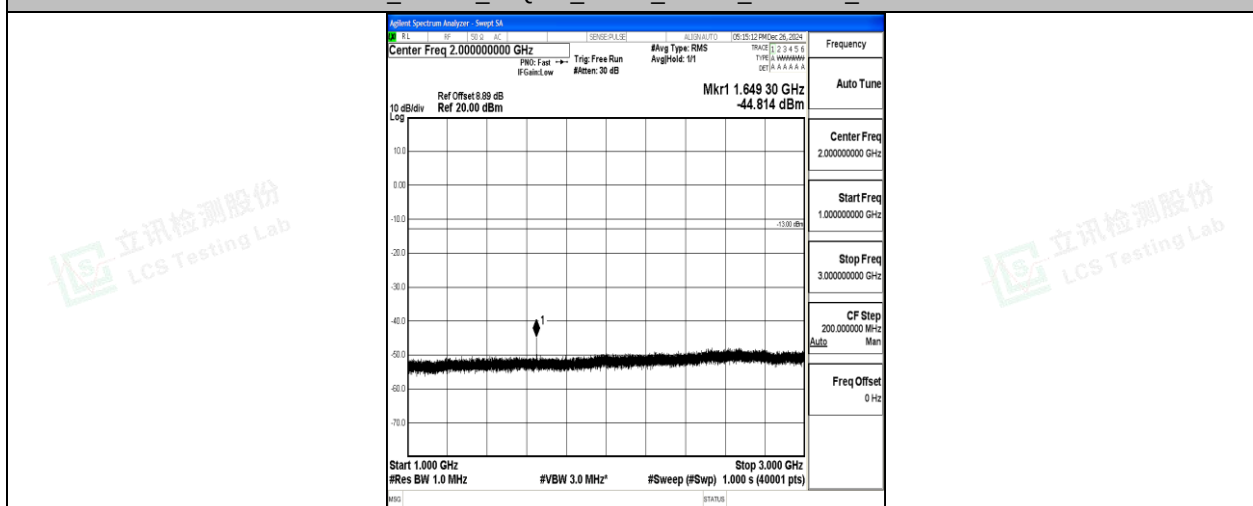
Band5_10MHz_16QAM_20450_1RB#0_1000~3000_1000~3000
