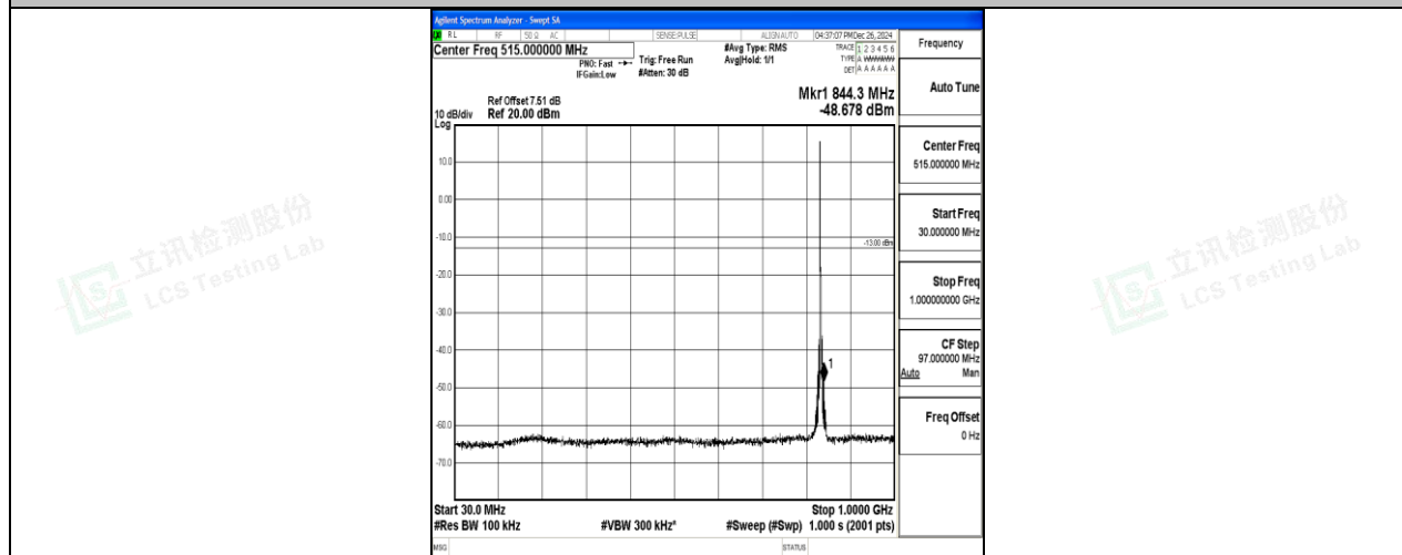
Band5_3MHz_16QAM_20525_1RB#0_30~1000_30~1000
