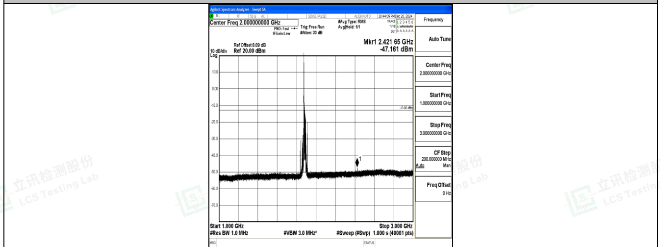
Band25_20MHz_16QAM_26365_1RB#0_1000~3000_1000~3000
