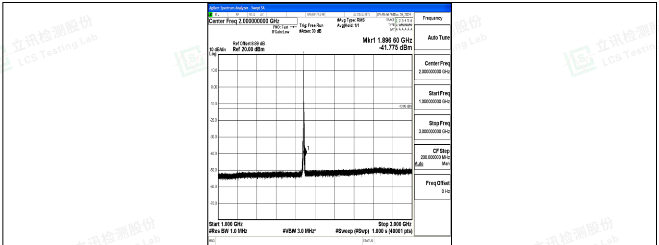
Band25_5MHz_QPSK_26365_1RB#0_1000~3000_1000~3000
