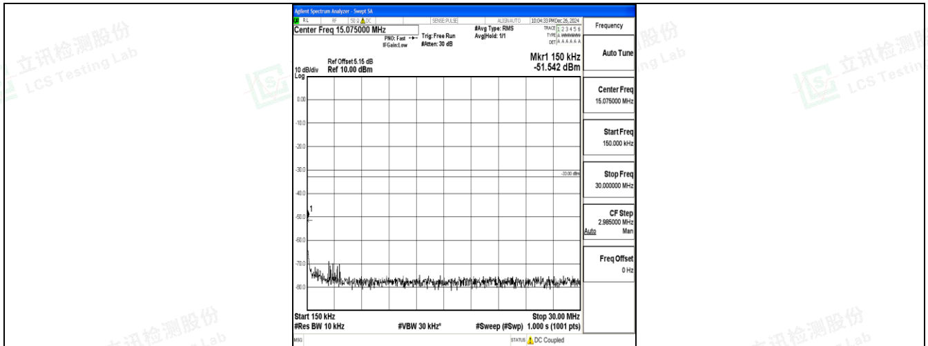
Band25_10MHz_QPSK_26090_1RB#0_0.15~30_0.15~30
