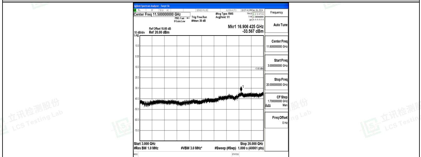
Band25_10MHz_16QAM_26640_1RB#0_3000~20000_3000~20000
