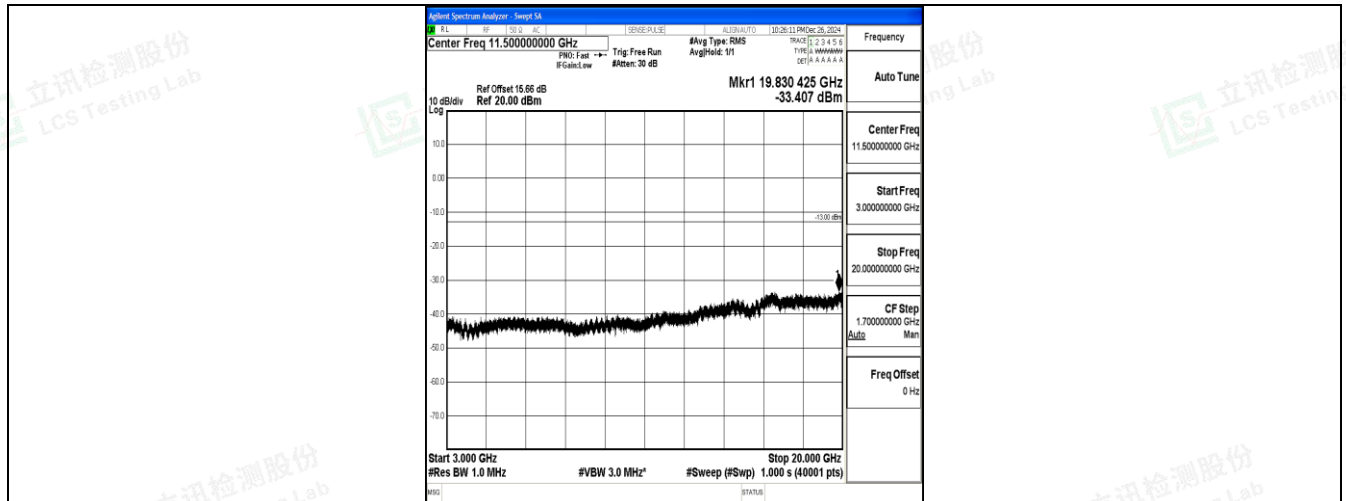
Band25_15MHz_QPSK_26615_1RB#0_3000~20000_3000~20000
