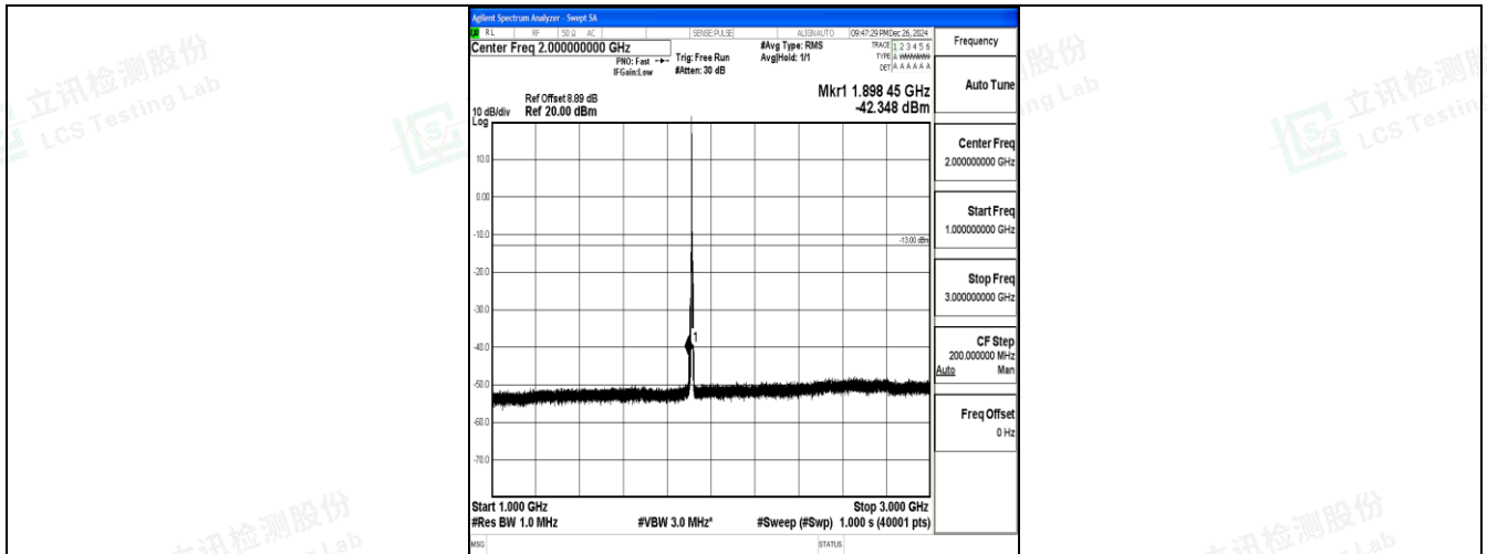
Band25_5MHz_16QAM_26665_1RB#0_1000~3000_1000~3000
