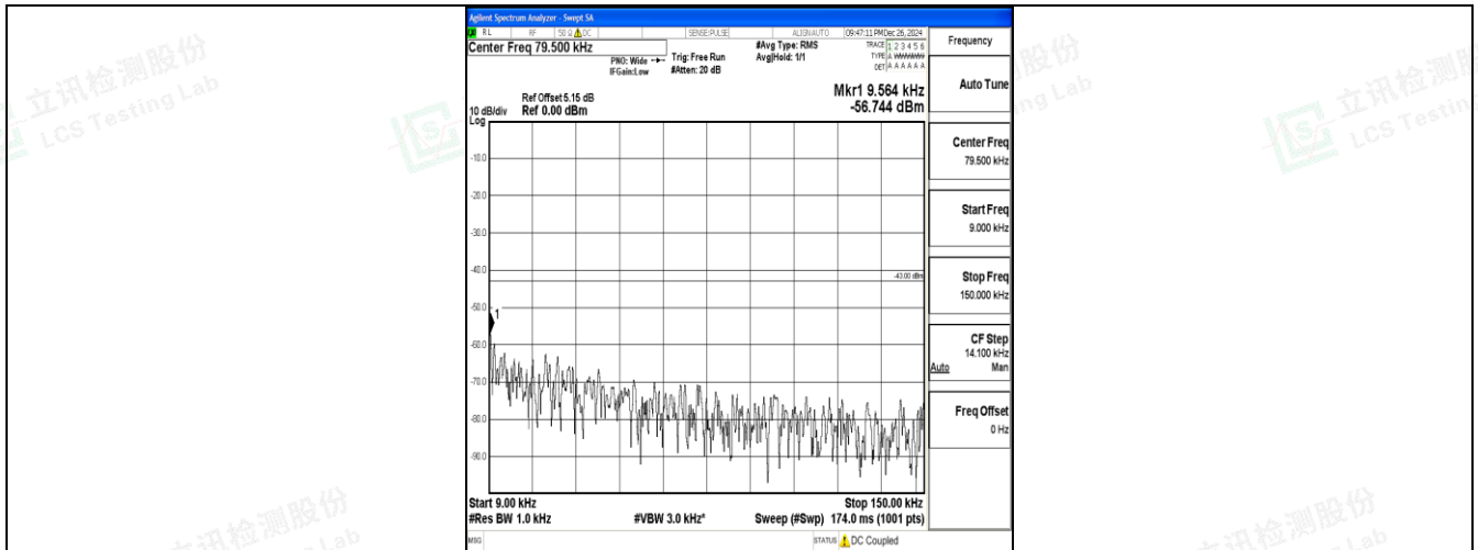
Band25_5MHz_16QAM_26665_1RB#0_0.009~0.15_0.009~0.15
