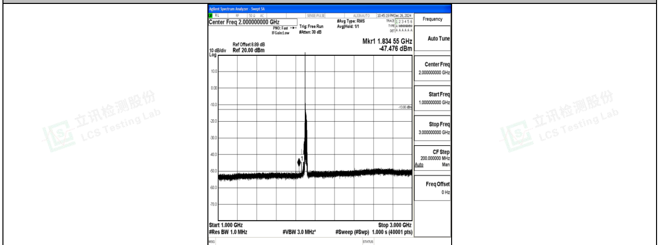
Band25_20MHz_16QAM_26590_1RB#0_1000~3000_1000~3000
