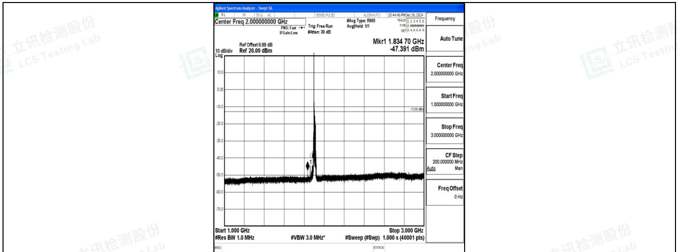
Band25_20MHz_QPSK_26590_1RB#0_1000~3000_1000~3000
