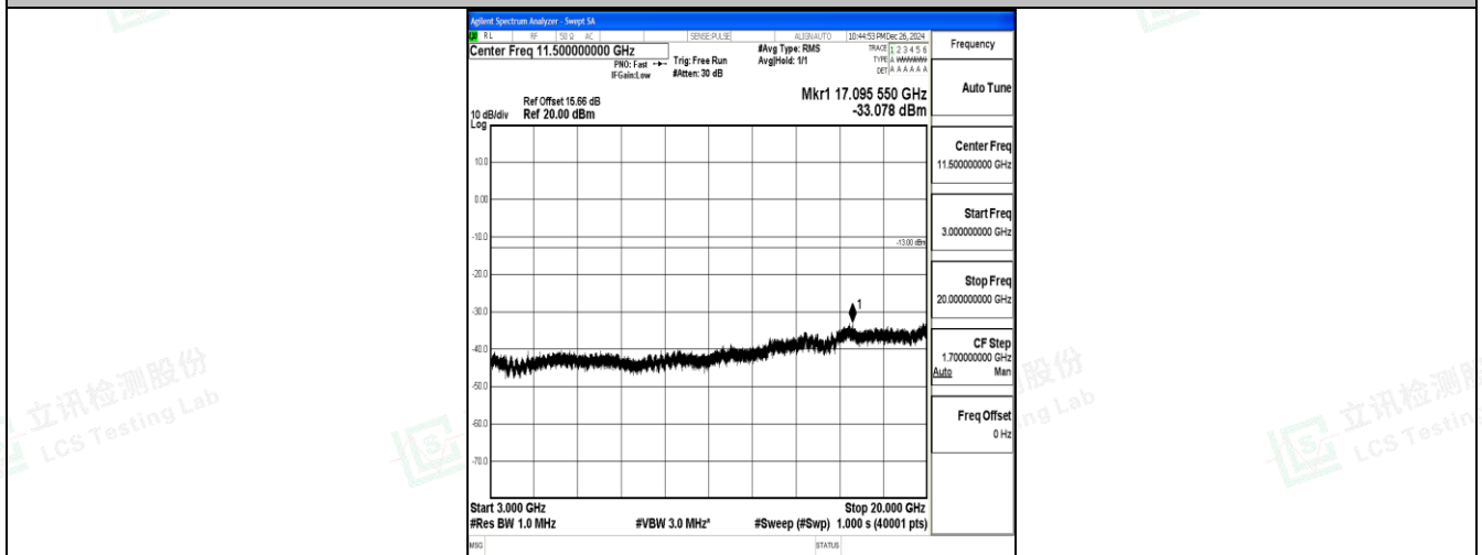
Band25_20MHz_QPSK_26590_1RB#0_3000~20000_3000~20000
