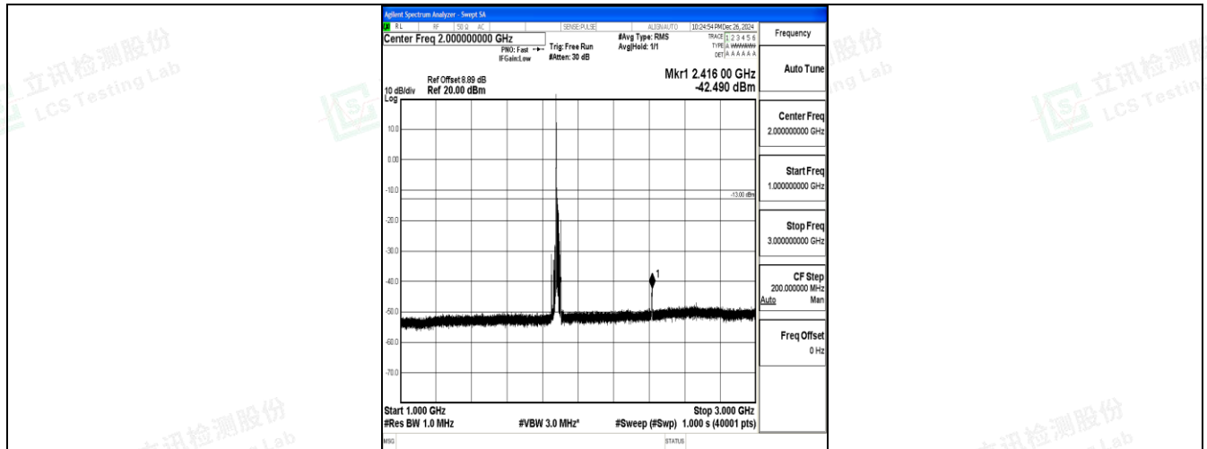
Band25_15MHz_QPSK_26365_1RB#0_1000~3000_1000~3000
