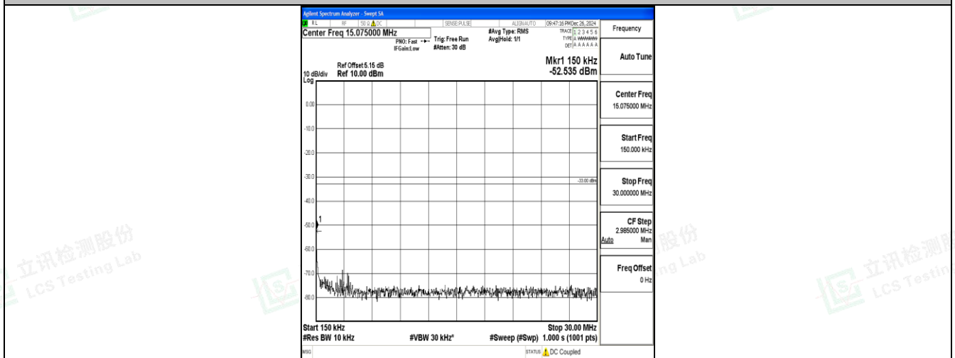
Band25_5MHz_16QAM_26665_1RB#0_0.15~30_0.15~30
