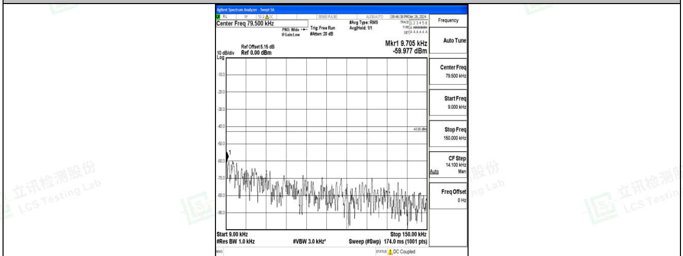
Band25_5MHz_QPSK_26665_1RB#0_0.009~0.15_0.009~0.15
