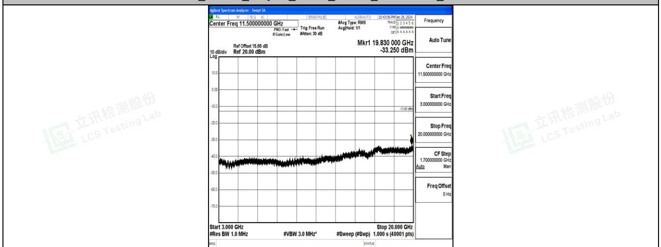
Band25_20MHz_16QAM_26140_1RB#0_3000~20000_3000~20000
