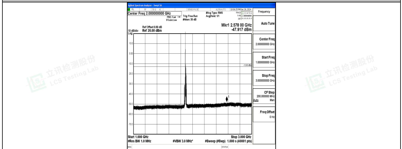
Band25_10MHz_16QAM_26365_1RB#0_1000~3000_1000~3000
