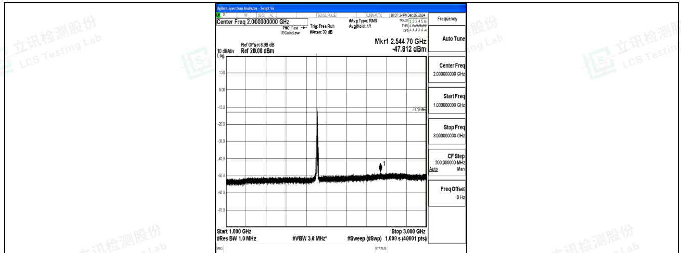
Band25_10MHz_16QAM_26640_1RB#0_1000~3000_1000~3000
