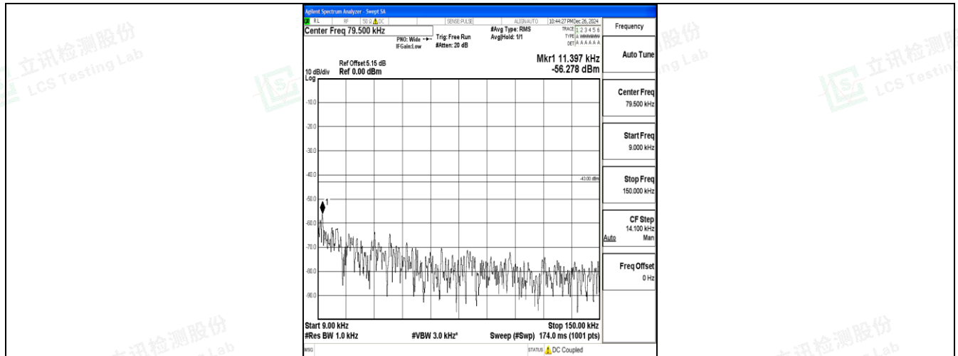
Band25_20MHz_QPSK_26590_1RB#0_0.009~0.15_0.009~0.15
