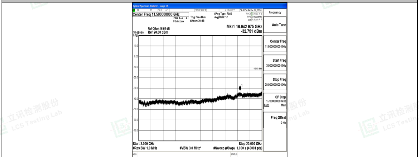
Band25_5MHz_QPSK_26365_1RB#0_3000~20000_3000~20000
