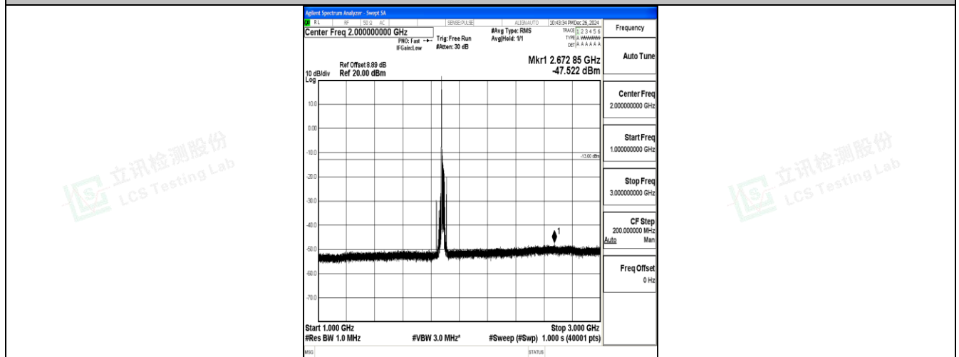
Band25_20MHz_QPSK_26365_1RB#0_1000~3000_1000~3000
