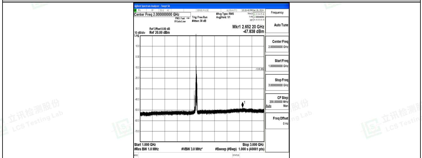
Band25_15MHz_16QAM_26615_1RB#0_1000~3000_1000~3000
