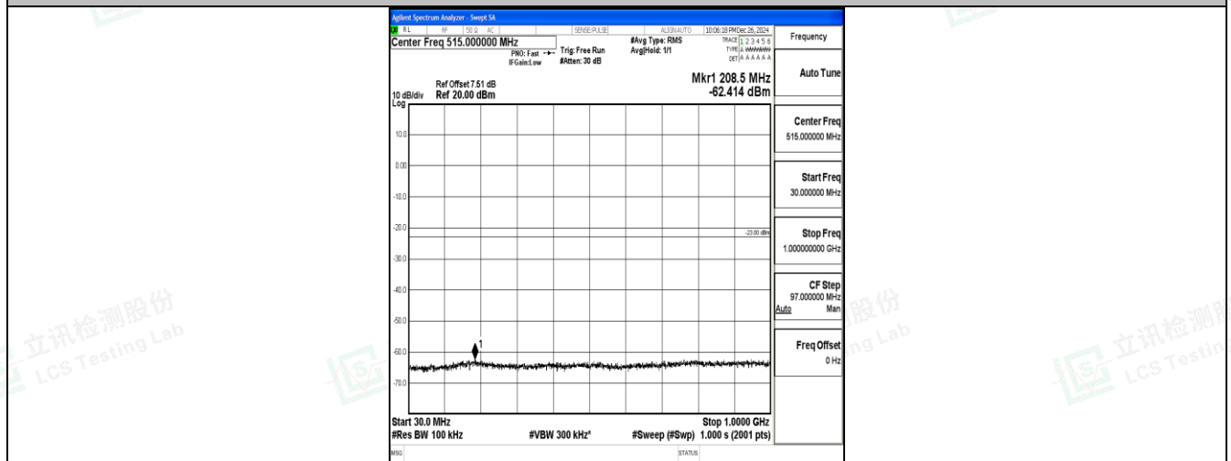
Band25_10MHz_16QAM_26365_1RB#0_30~1000_30~1000
