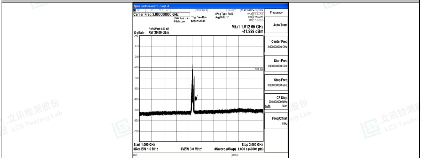
Band25_20MHz_16QAM_26140_1RB#0_1000~3000_1000~3000
