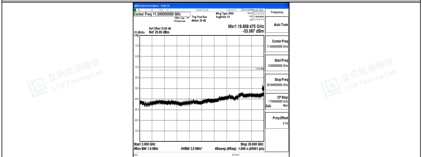
Band25_5MHz_QPSK_26665_1RB#0_3000~20000_3000~20000
