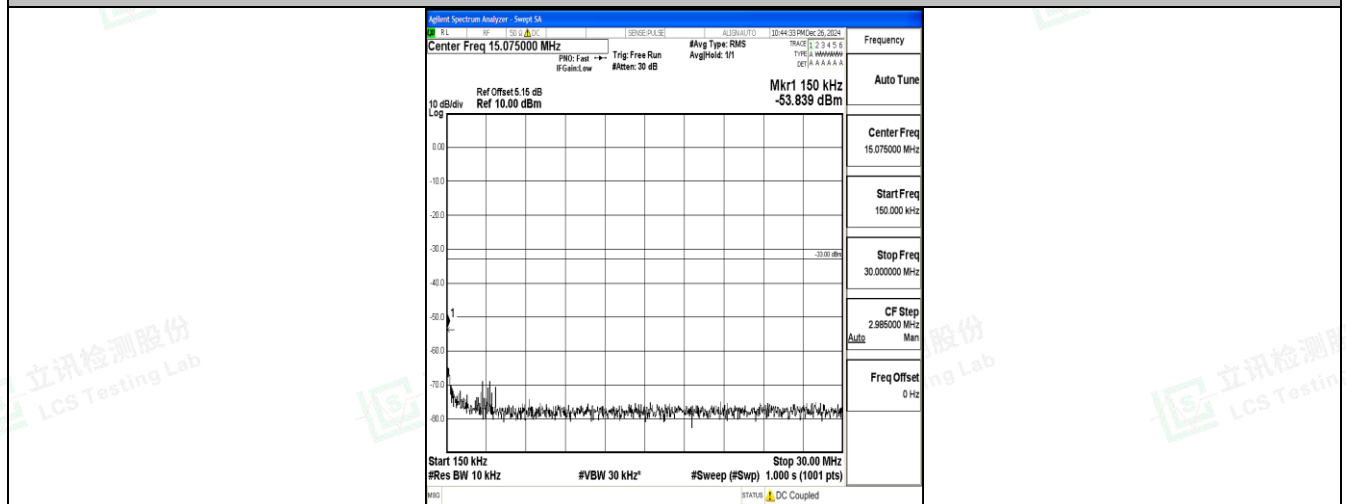
Band25_20MHz_QPSK_26590_1RB#0_0.15~30_0.15~30
