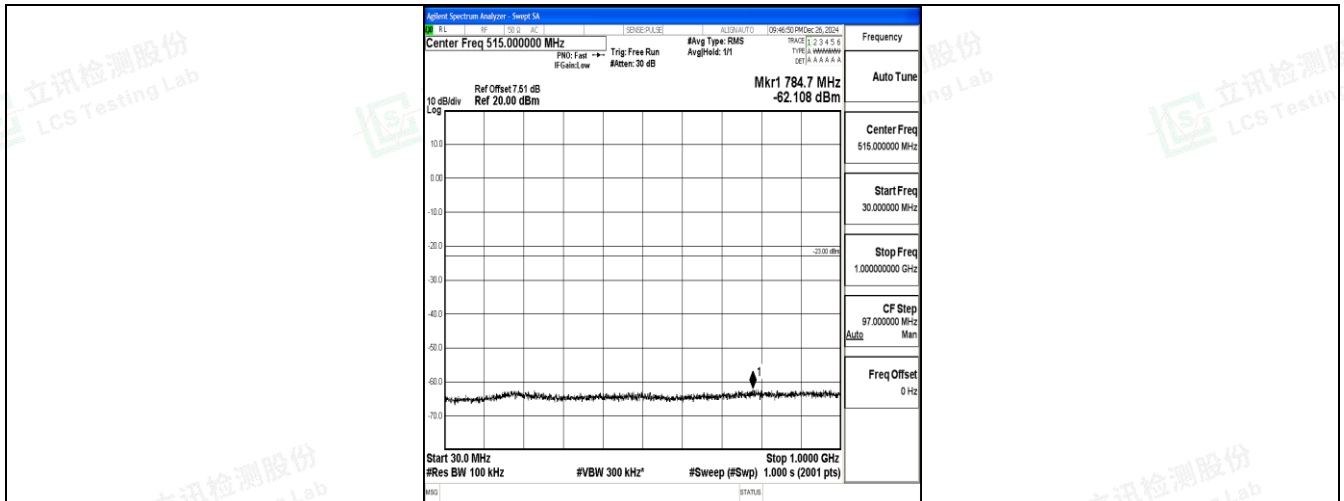
Band25_5MHz_QPSK_26665_1RB#0_30~1000_30~1000
