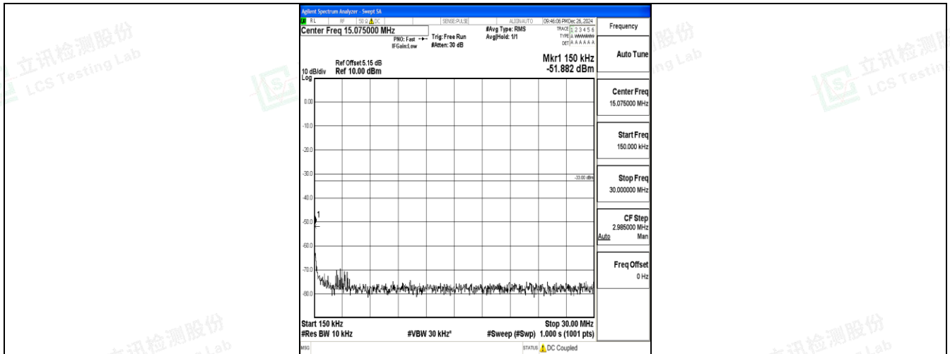
Band25_5MHz_16QAM_26365_1RB#0_0.15~30_0.15~30
