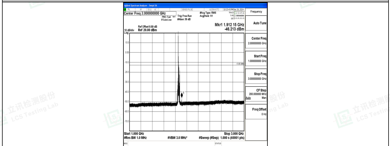
Band25_15MHz_QPSK_26115_1RB#0_1000~3000_1000~3000
