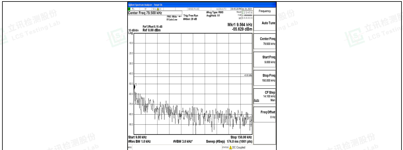
Band25_5MHz_QPSK_26365_1RB#0_0.009~0.15_0.009~0.15
