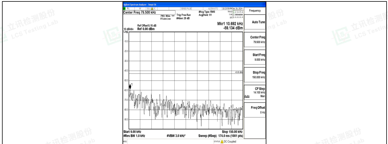
Band25_15MHz_16QAM_26115_1RB#0_0.009~0.15_0.009~0.15
