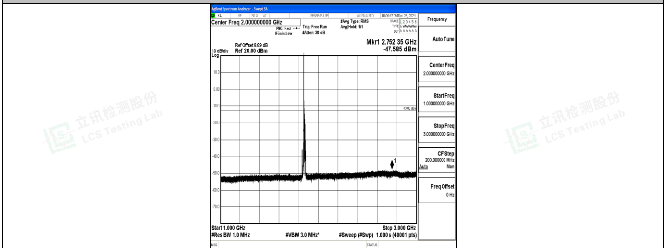
Band25_10MHz_QPSK_26090_1RB#0_1000~3000_1000~3000
