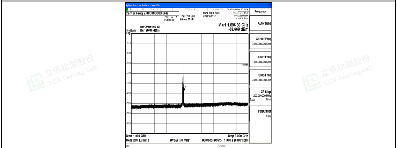
Band25_5MHz_16QAM_26365_1RB#0_1000~3000_1000~3000
