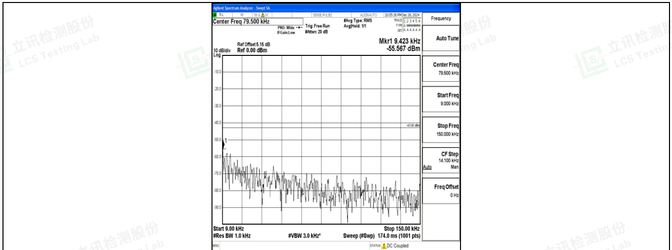
Band25_10MHz_QPSK_26365_1RB#0_0.009~0.15_0.009~0.15
