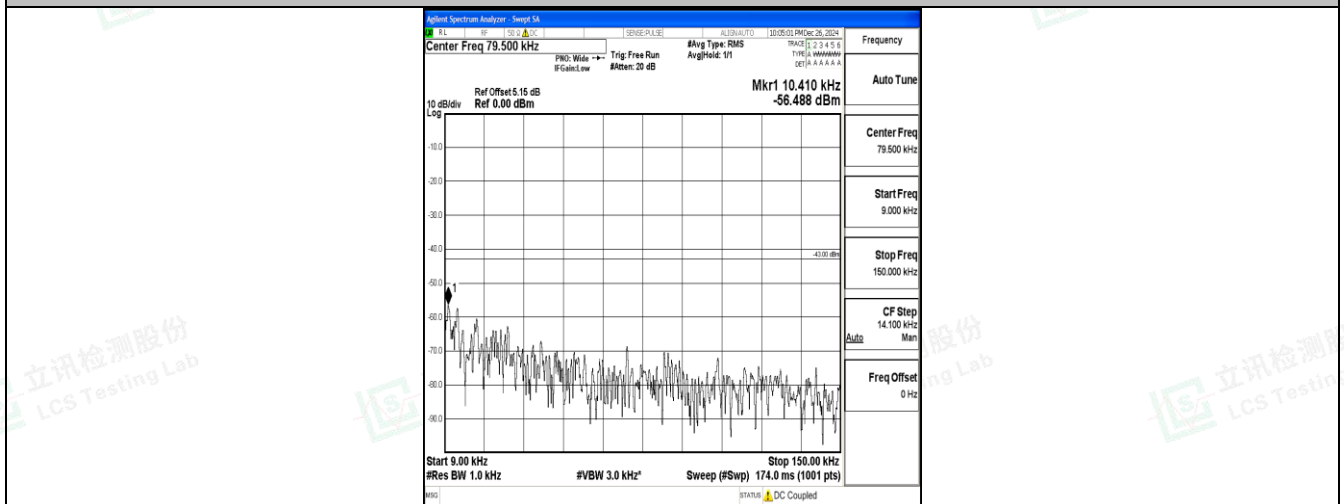
Band25_10MHz_16QAM_26090_1RB#0_0.009~0.15_0.009~0.15
