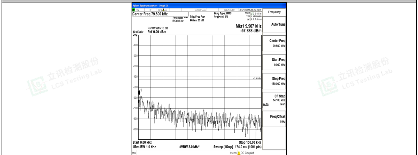
Band25_10MHz_QPSK_26090_1RB#0_0.009~0.15_0.009~0.15
