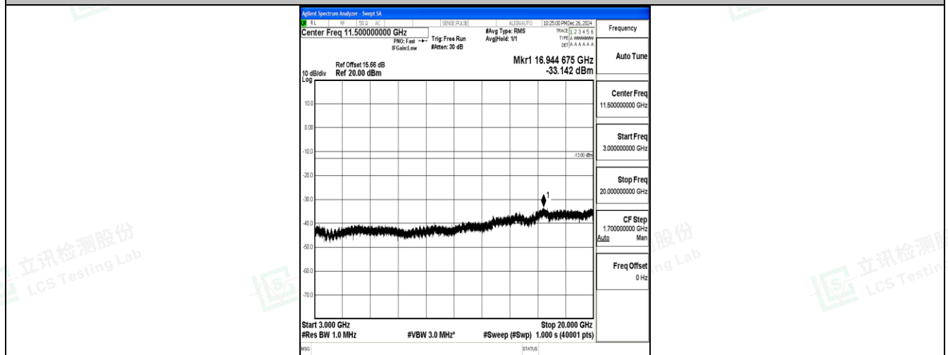
Band25_15MHz_QPSK_26365_1RB#0_3000~20000_3000~20000
