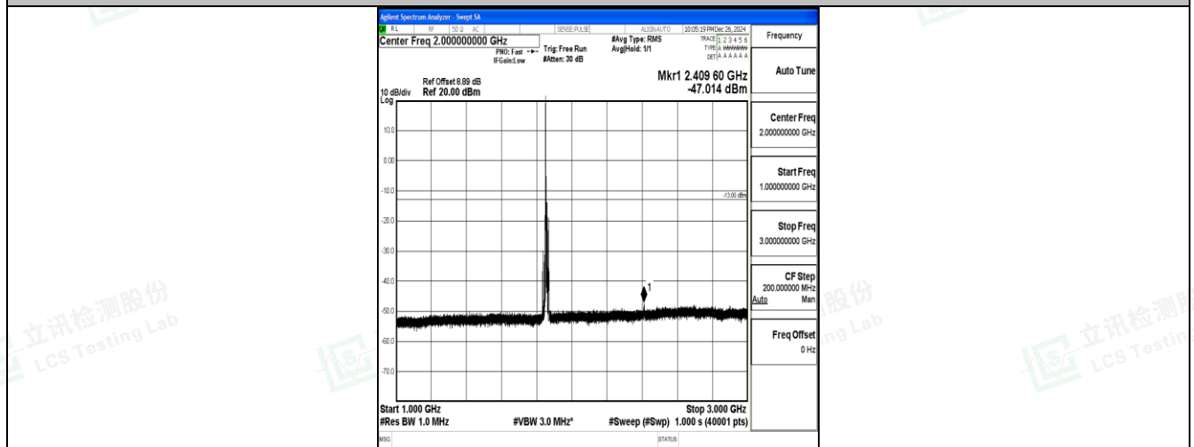
Band25_10MHz_16QAM_26090_1RB#0_1000~3000_1000~3000
