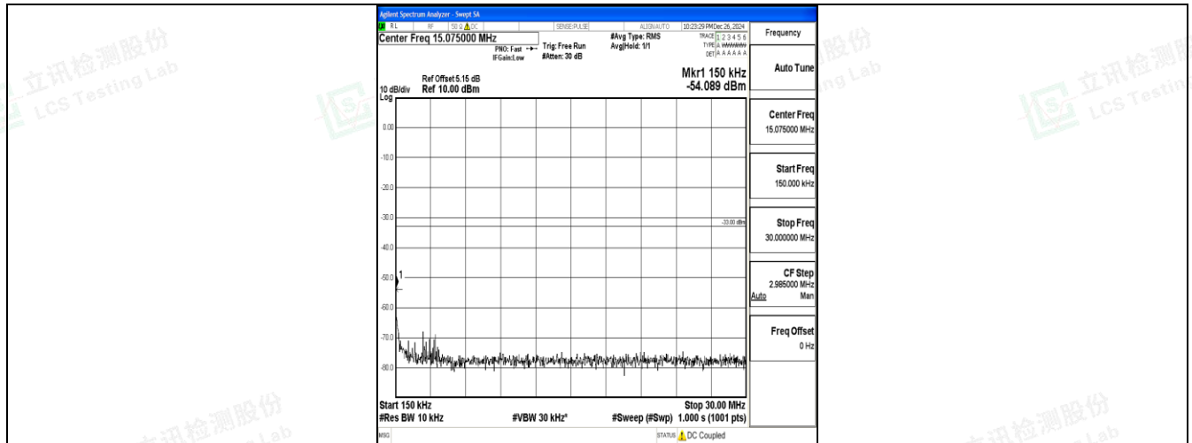
Band25_15MHz_QPSK_26115_1RB#0_0.15~30_0.15~30
