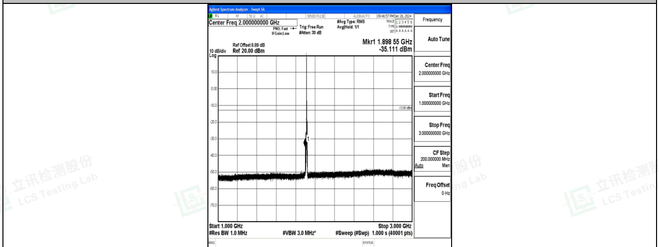
Band25_5MHz_QPSK_26665_1RB#0_1000~3000_1000~3000
