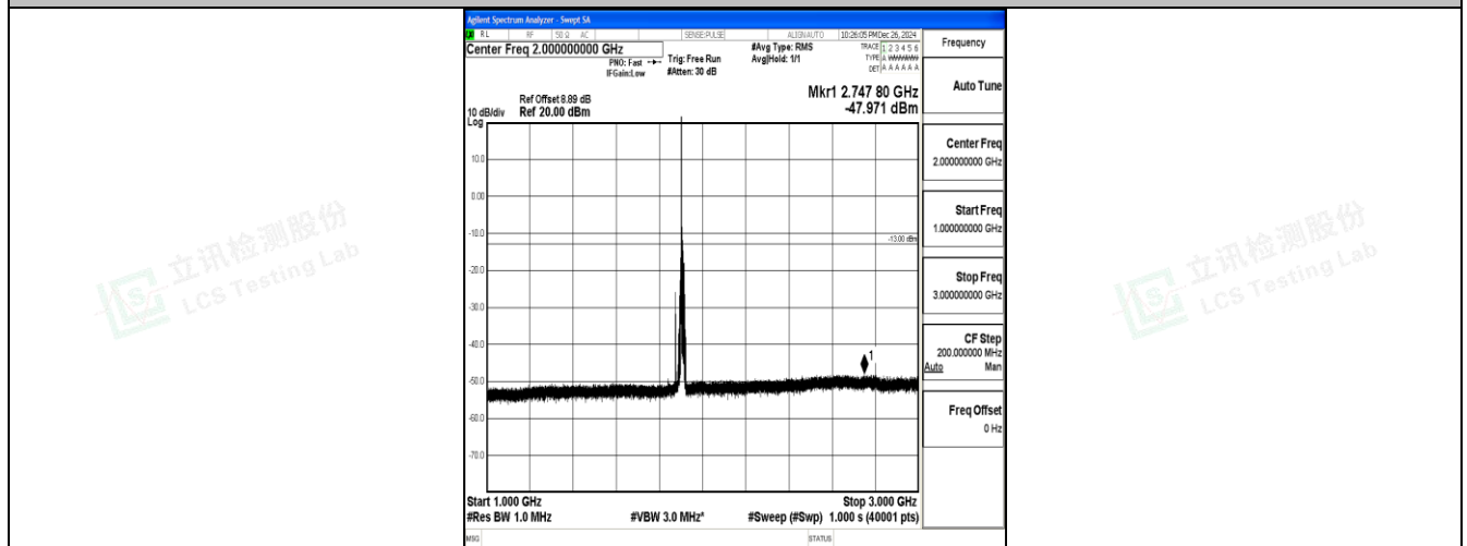
Band25_15MHz_QPSK_26615_1RB#0_1000~3000_1000~3000
