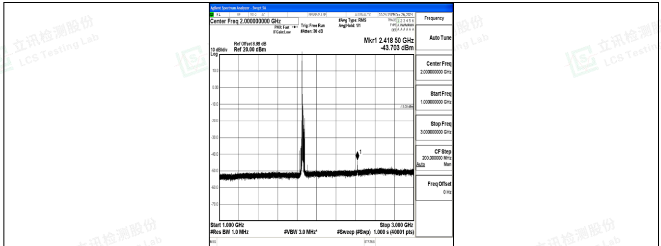
Band25_15MHz_16QAM_26115_1RB#0_1000~3000_1000~3000
