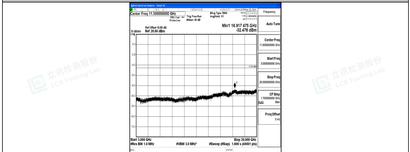
Band25_20MHz_16QAM_26365_1RB#0_3000~20000_3000~20000
