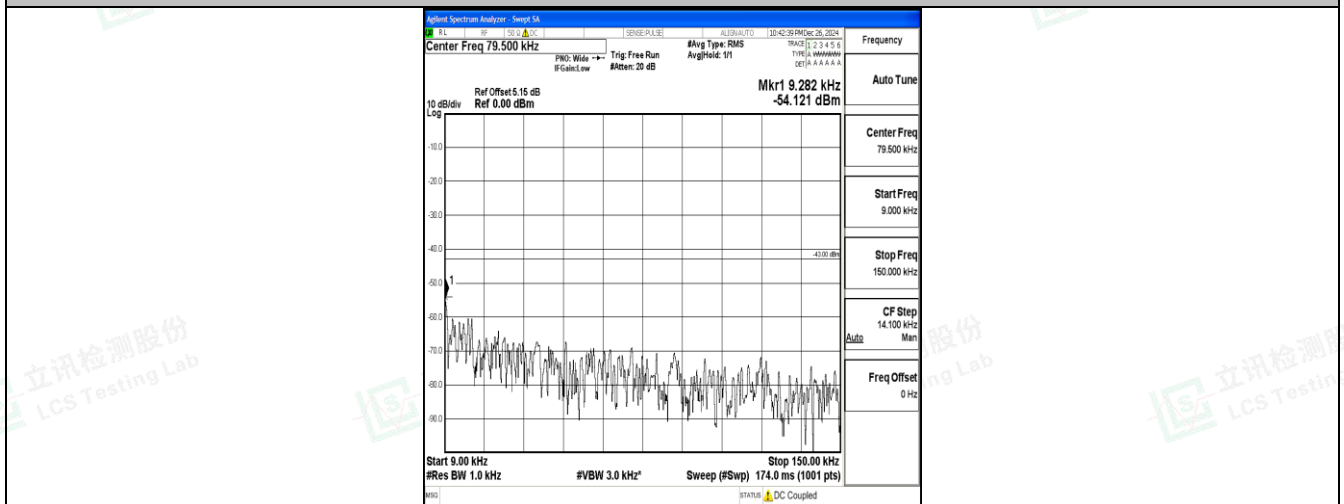
Band25_20MHz_16QAM_26140_1RB#0_0.009~0.15_0.009~0.15
