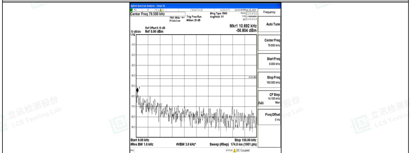
Band25_20MHz_16QAM_26365_1RB#0_0.009~0.15_0.009~0.15
