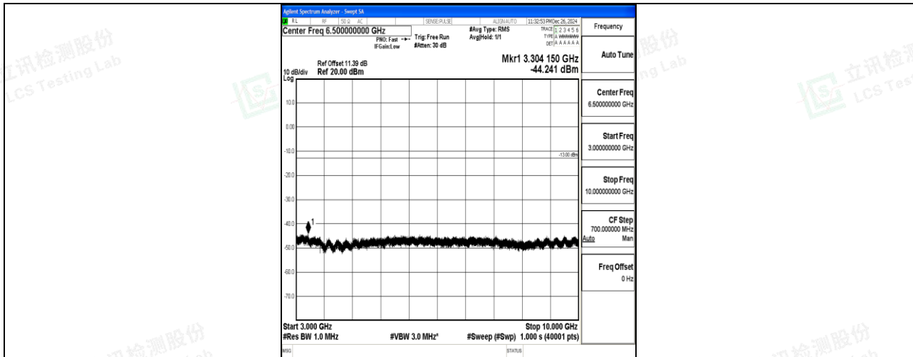
Band26_3MHz_16QAM_26775_1RB#0_3000~10000_3000~10000
