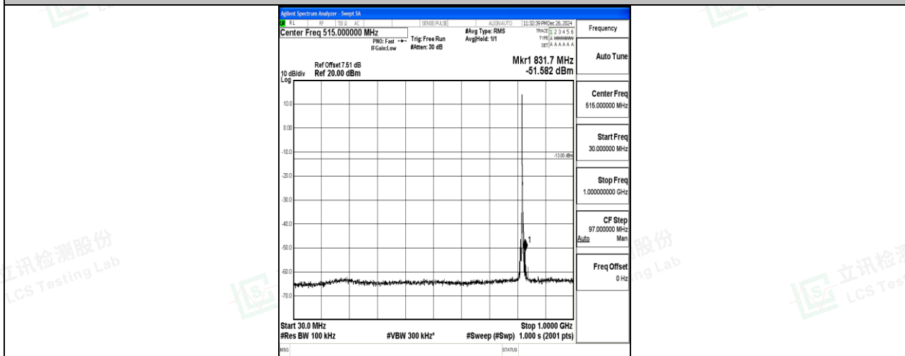
Band26_3MHz_16QAM_26775_1RB#0_30~1000_30~1000
