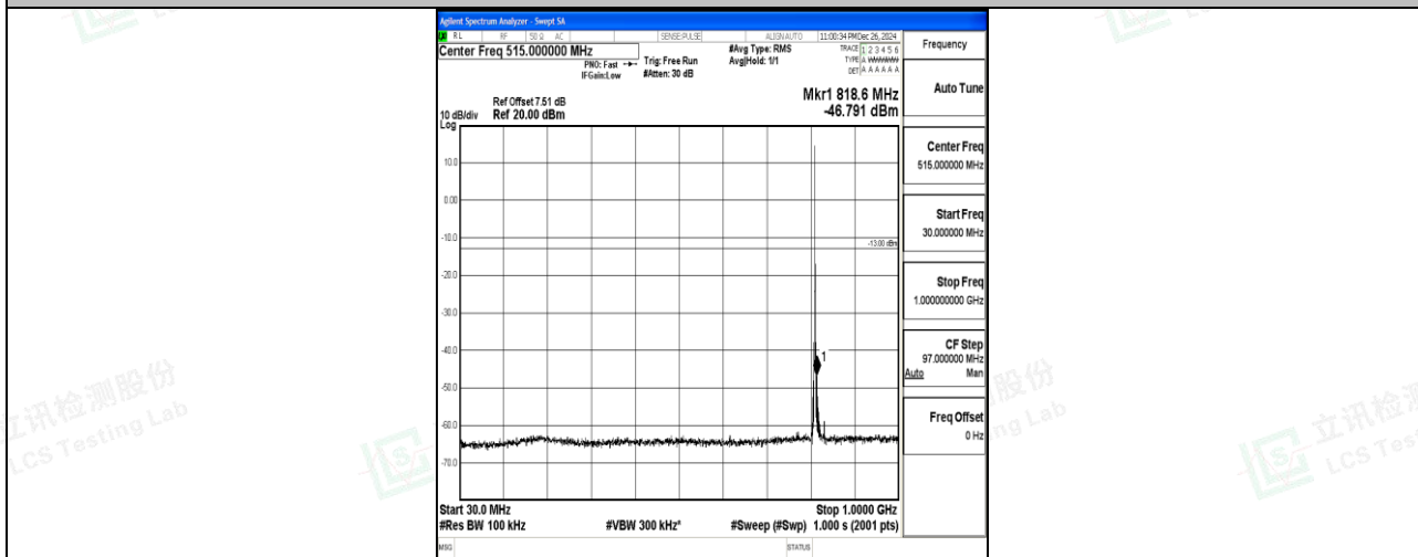
Band26_1.4MHz_QPSK_26697_1RB#0_30~1000_30~1000
