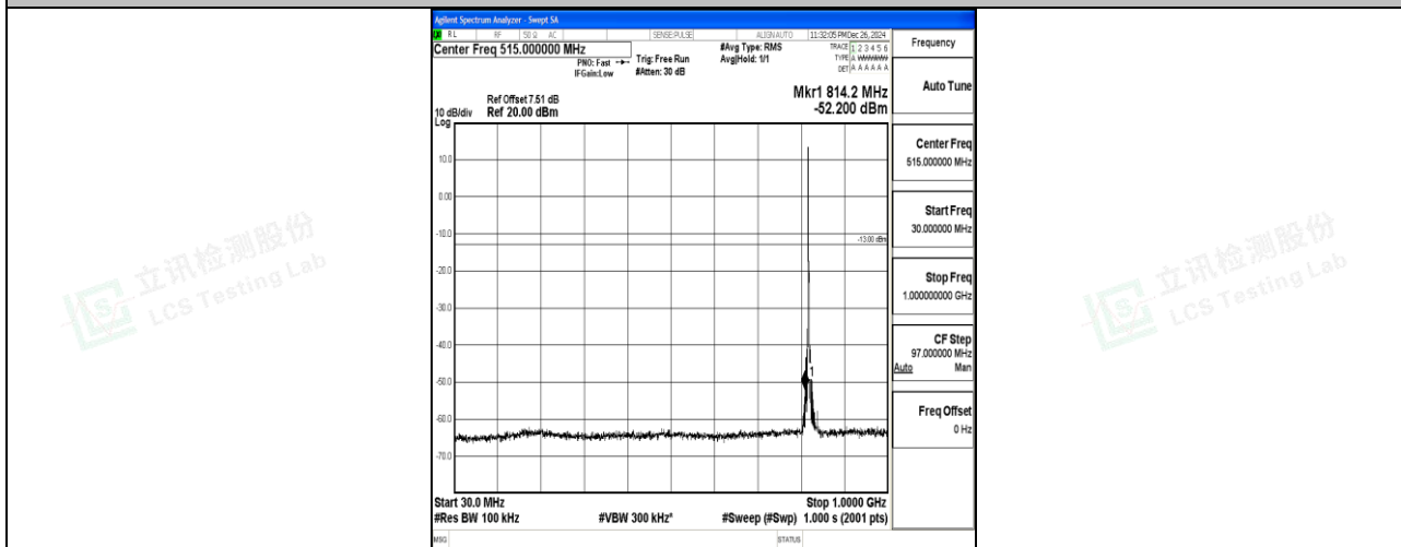
Band26_3MHz_QPSK_26775_1RB#0_30~1000_30~1000
