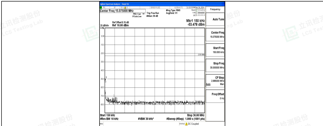
Band26_3MHz_16QAM_26775_1RB#0_0.15~30_0.15~30
