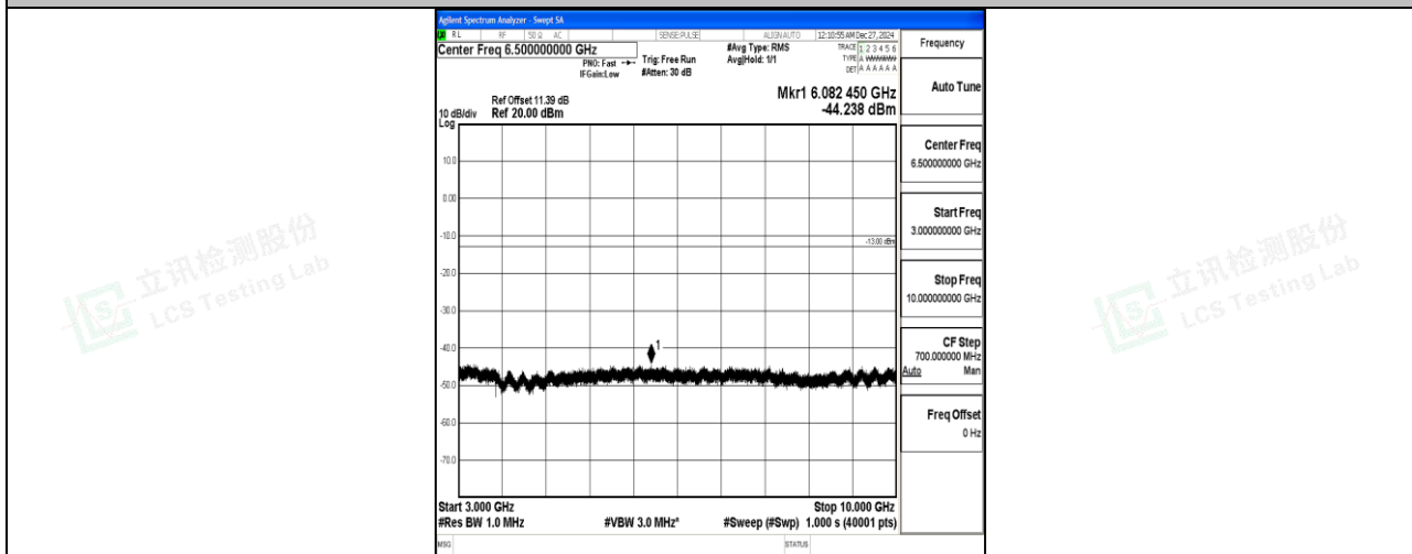
Band26_10MHz_16QAM_26740_1RB#0_3000~10000_3000~10000
