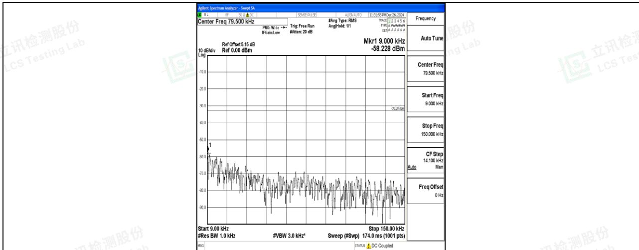
Band26_3MHz_QPSK_26775_1RB#0_0.009~0.15_0.009~0.15
