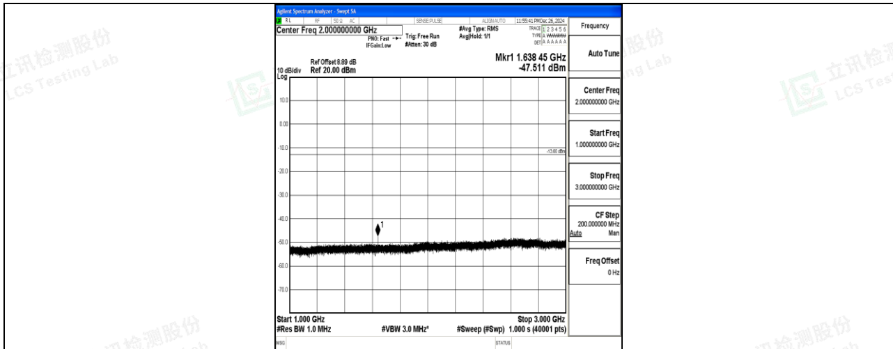
Band26_5MHz_16QAM_26765_1RB#0_1000~3000_1000~3000
