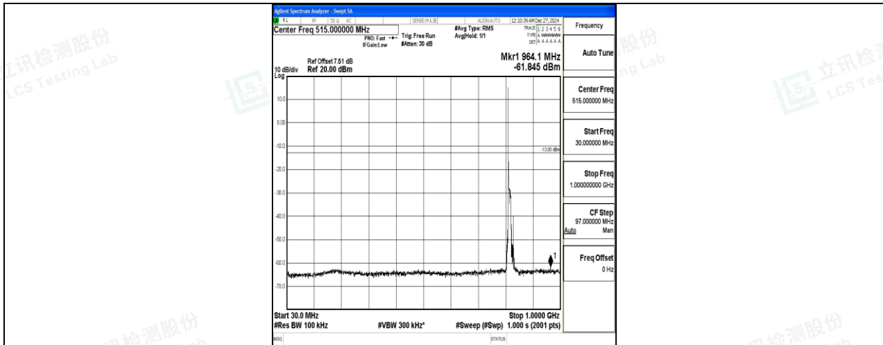
Band26_10MHz_16QAM_26740_1RB#0_30~1000_30~1000
