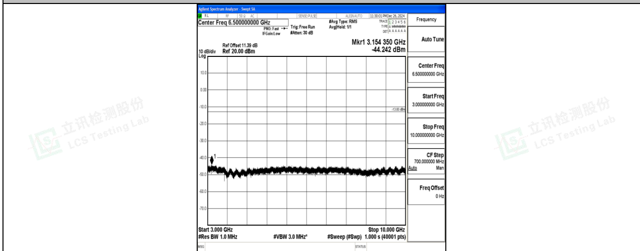
Band26_3MHz_QPSK_26705_1RB#0_3000~10000_3000~10000
