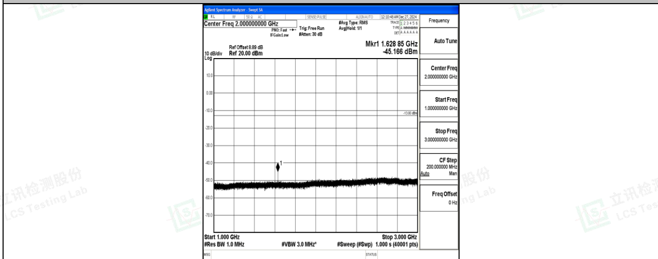
Band26_10MHz_16QAM_26740_1RB#0_1000~3000_1000~3000
