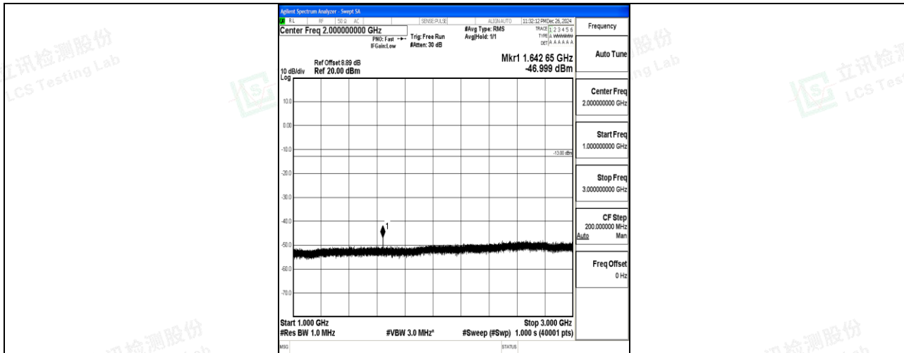
Band26_3MHz_QPSK_26775_1RB#0_1000~3000_1000~3000
