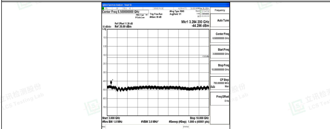
Band26_3MHz_QPSK_26775_1RB#0_3000~10000_3000~10000
