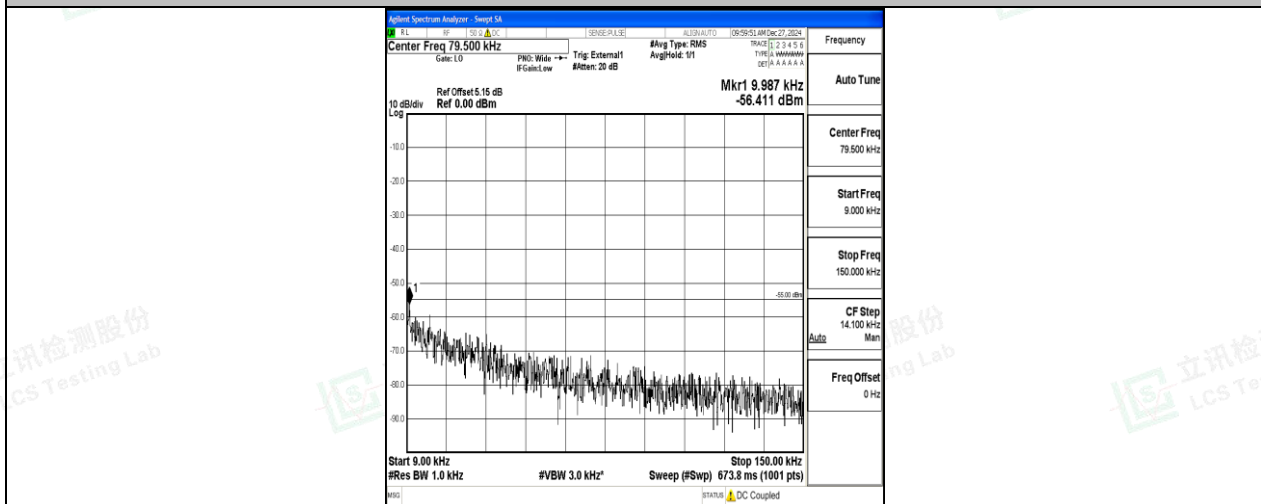
Band38_15MHz_QPSK_37825_1RB#0_0.009~0.15_0.009~0.15
