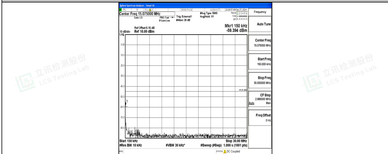
Band38_15MHz_16QAM_38175_1RB#0_0.15~30_0.15~30
