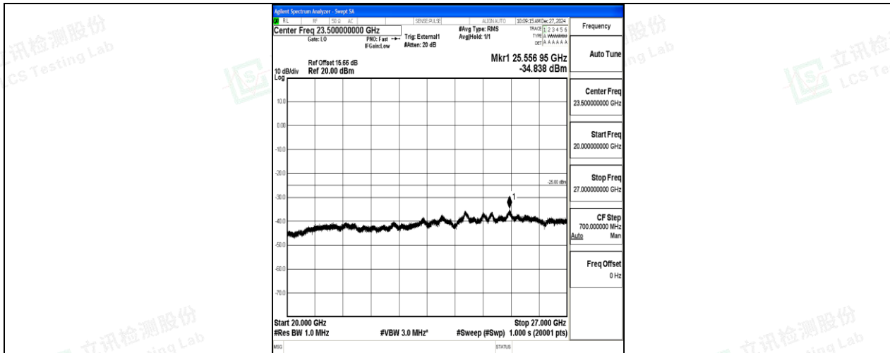
Band38_15MHz_QPSK_38175_1RB#0_20000~27000_20000~27000
