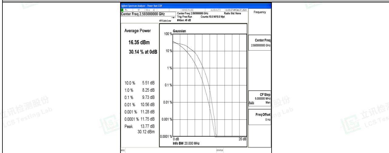
Band41-20MHz-16QAM-40620-100RB#0-PASS
