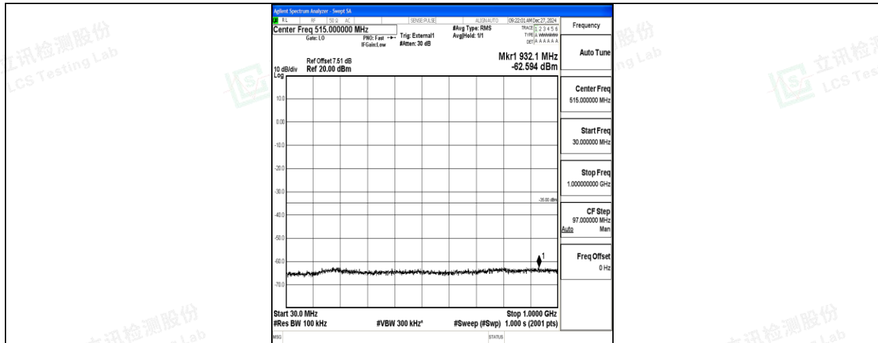
Band41_5MHz_QPSK_40620_1RB#0_30~1000_30~1000
