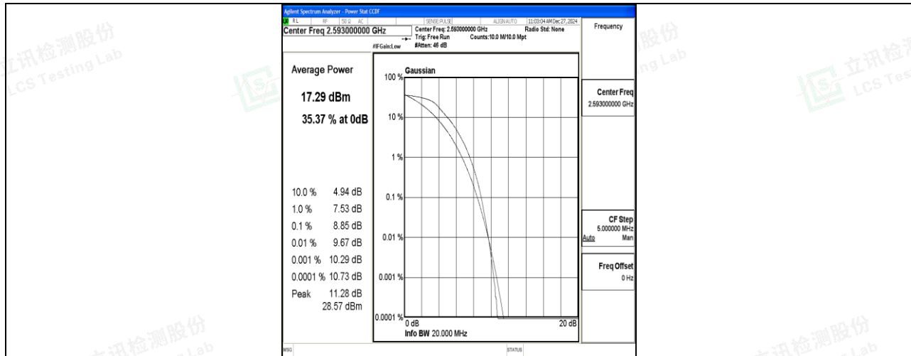
Band41-20MHz-QPSK-40620-100RB#0-PASS
