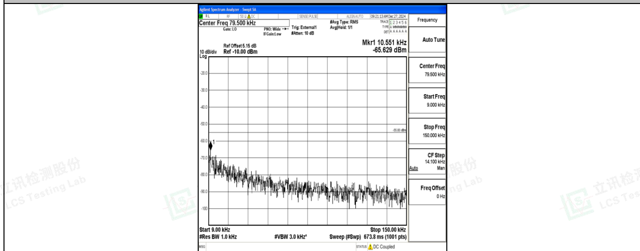
Band41_5MHz_QPSK_40620_1RB#0_0.009~0.15_0.009~0.15
