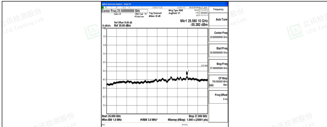
Band41_5MHz_16QAM_39675_1RB#0_20000~27000_20000~27000
