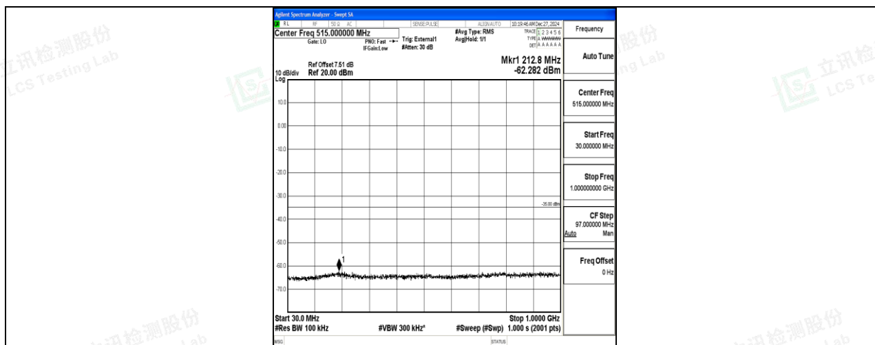
Band41_15MHz_QPSK_39725_1RB#0_30~1000_30~1000
