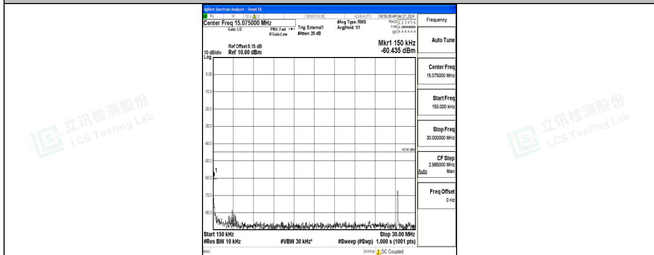
Band41_10MHz_16QAM_40620_1RB#0_0.15~30_0.15~30
