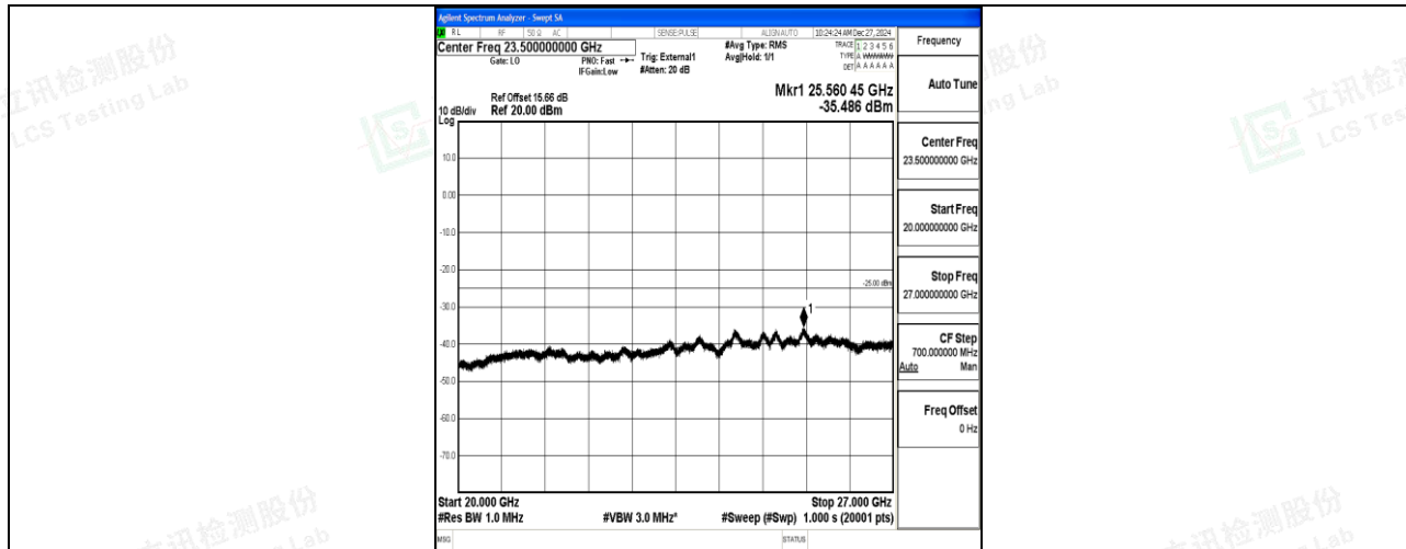
Band41_15MHz_QPSK_40620_1RB#0_20000~27000_20000~27000
