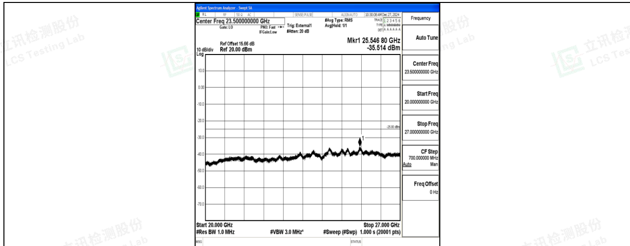
Band41_15MHz_16QAM_41515_1RB#0_20000~27000_20000~27000
