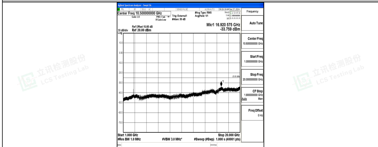
Band41_5MHz_QPSK_41565_1RB#0_1000~20000_1000~20000
