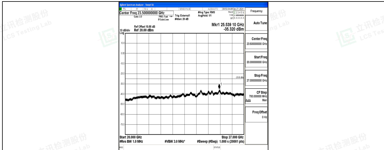
Band41_10MHz_16QAM_39700_1RB#0_20000~27000_20000~27000
