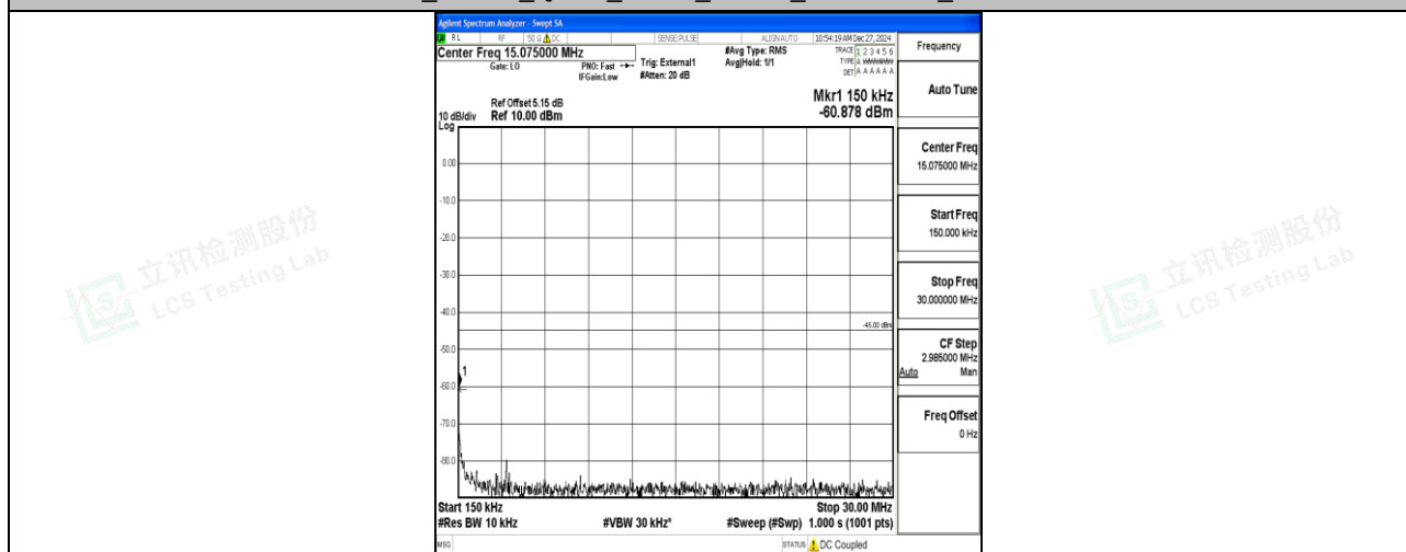
Band41_20MHz_QPSK_41490_1RB#0_0.15~30_0.15~30
