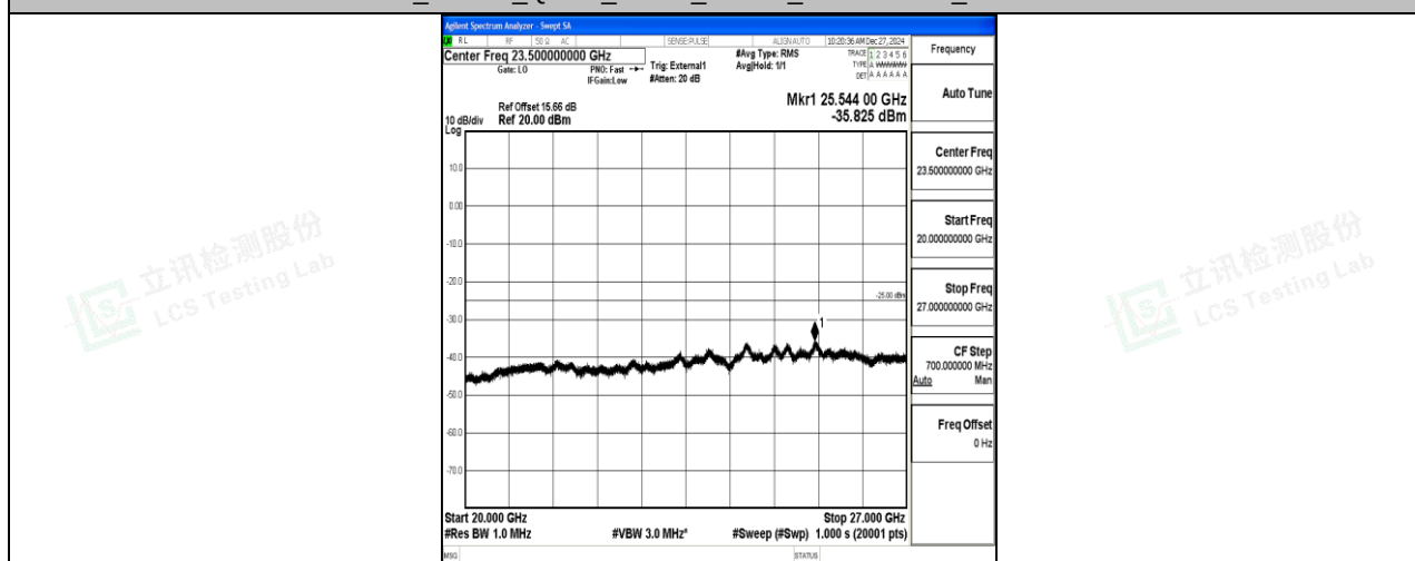
Band41_15MHz_QPSK_39725_1RB#0_20000~27000_20000~27000
