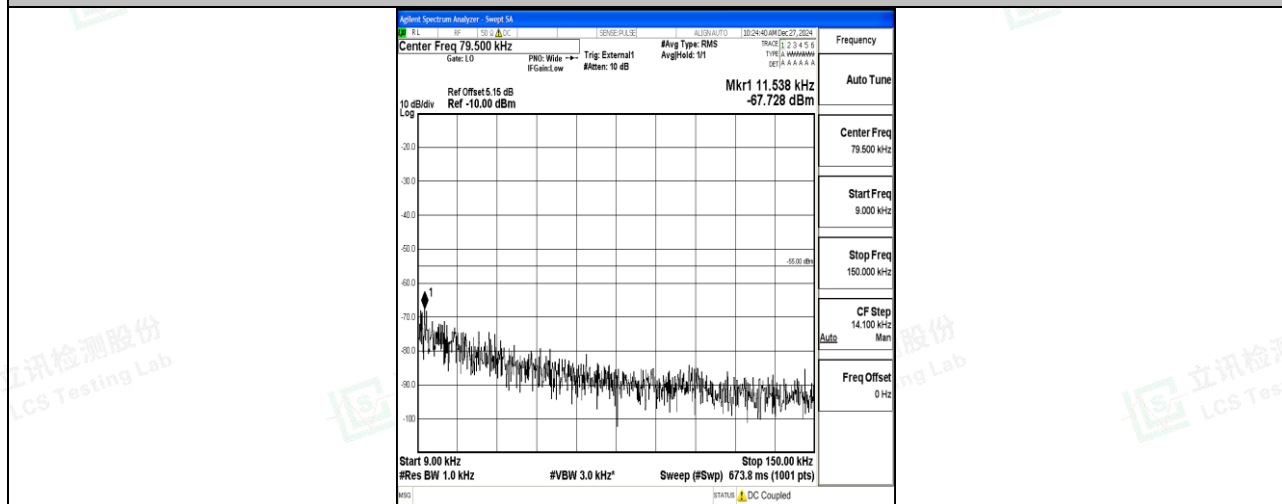
Band41_15MHz_16QAM_40620_1RB#0_0.009~0.15_0.009~0.15
