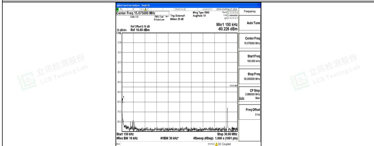
Band41_10MHz_QPSK_40620_1RB#0_0.15~30_0.15~30
