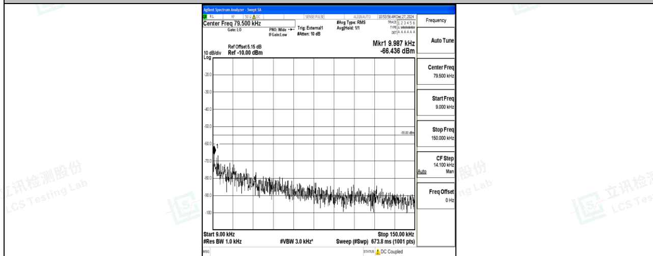
Band41_20MHz_QPSK_41490_1RB#0_0.009~0.15_0.009~0.15
