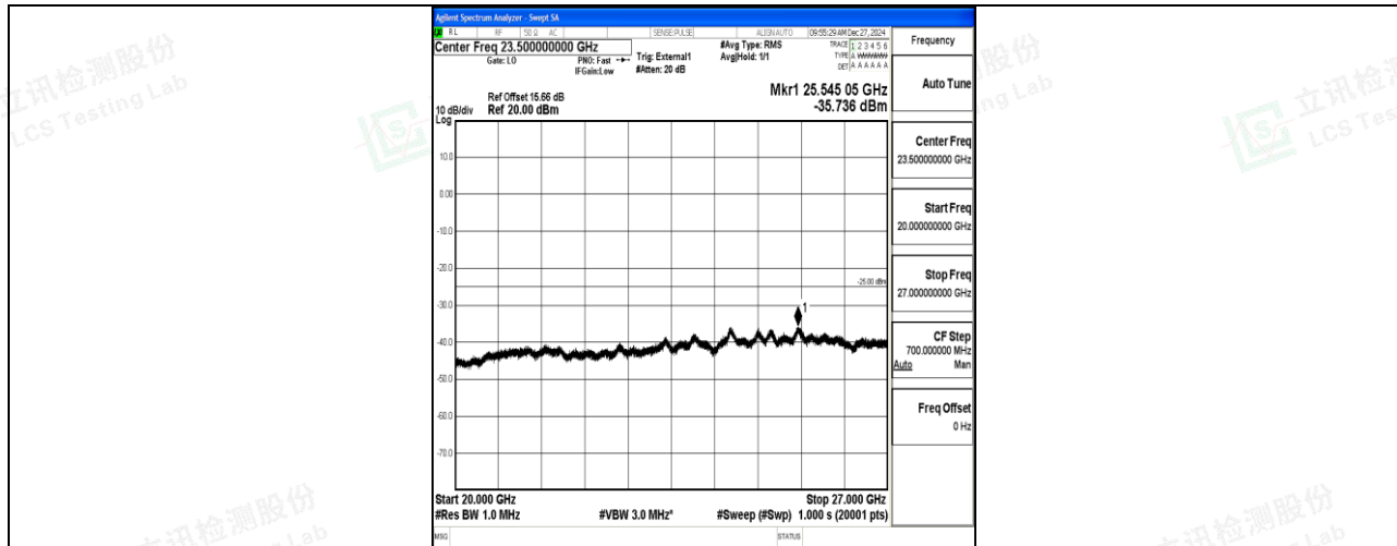
Band41_10MHz_QPSK_40620_1RB#0_20000~27000_20000~27000
