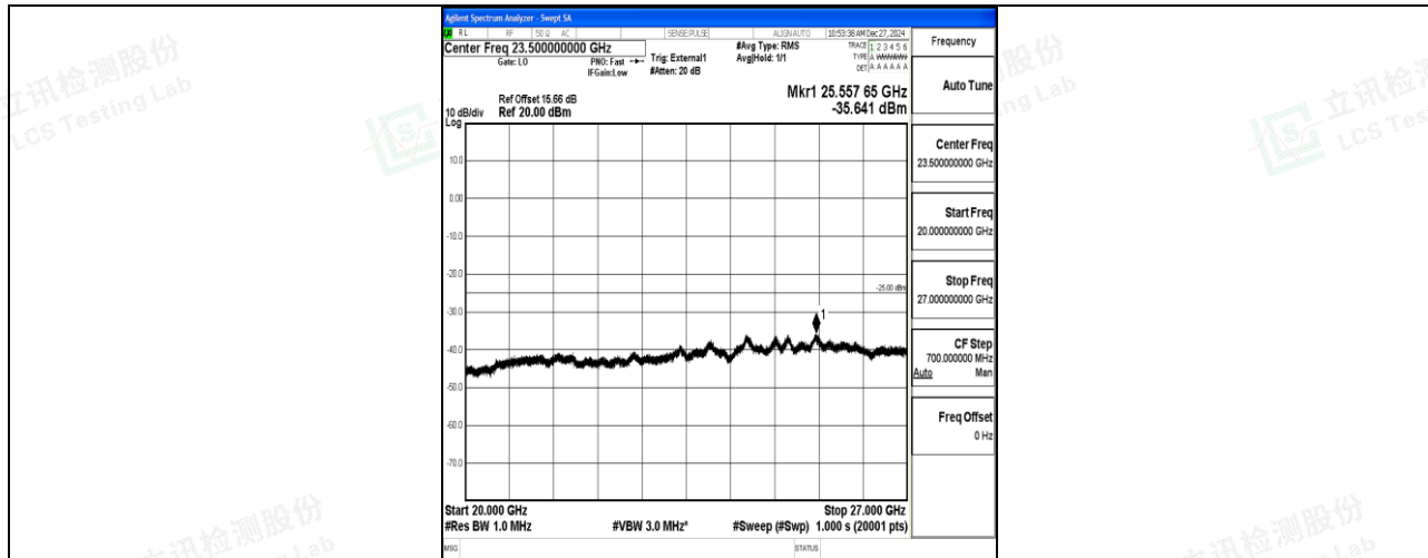
Band41_20MHz_16QAM_40620_1RB#0_20000~27000_20000~27000
