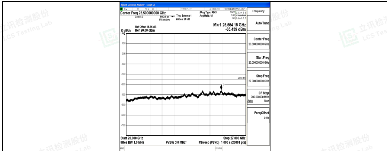
Band41_10MHz_16QAM_41540_1RB#0_20000~27000_20000~27000
