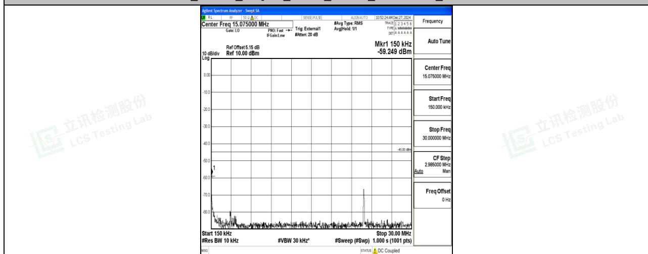
Band41_20MHz_16QAM_40620_1RB#0_0.15~30_0.15~30
