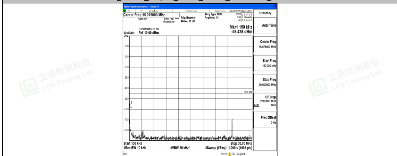
Band41_15MHz_16QAM_40620_1RB#0_0.15~30_0.15~30
