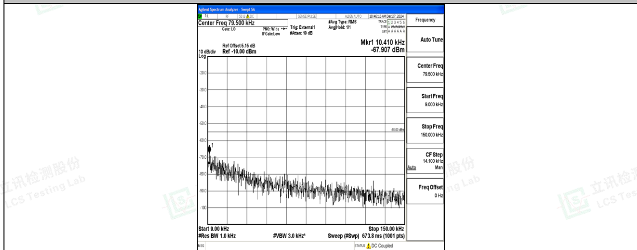
Band41_20MHz_QPSK_39750_1RB#0_0.009~0.15_0.009~0.15
