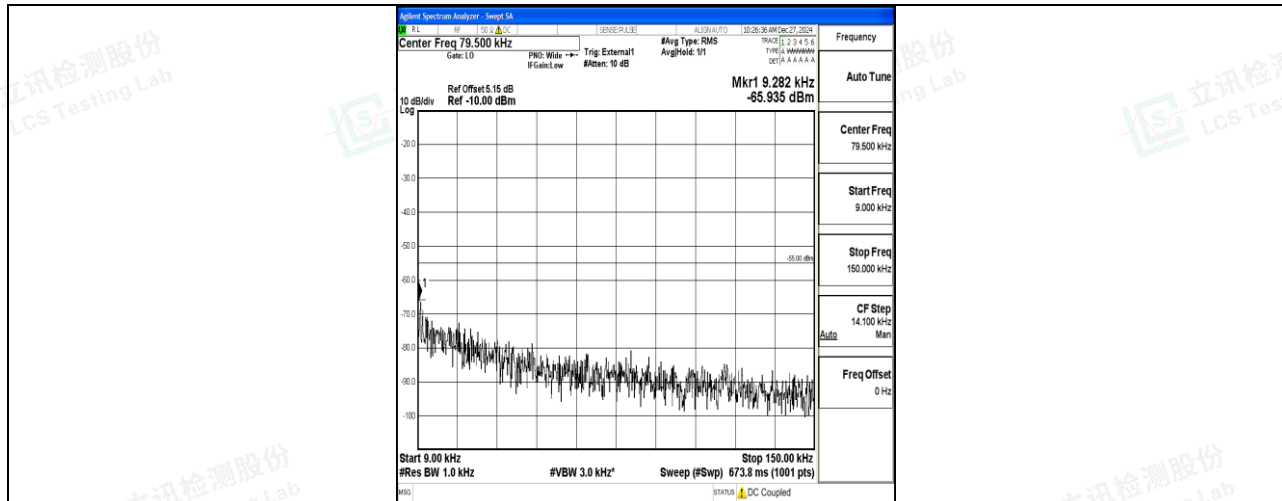
Band41_15MHz_QPSK_41515_1RB#0_0.009~0.15_0.009~0.15
