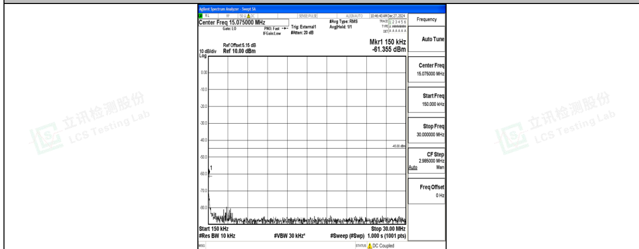
Band41_20MHz_QPSK_39750_1RB#0_0.15~30_0.15~30
