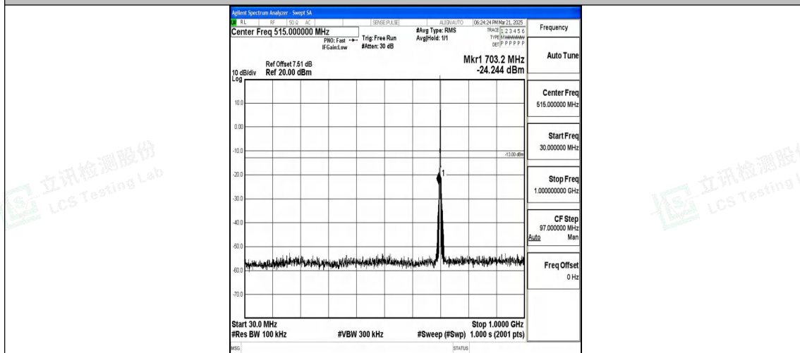
Band12_1.4MHz_QPSK_23095_1RB#0_30~1000_30~1000
