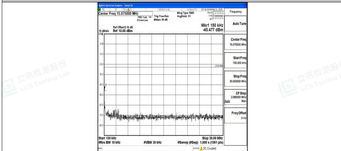
Band12_10MHz_16QAM_23060_1RB#0_0.15~30_0.15~30
