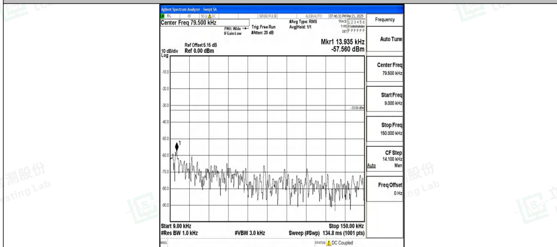
Band12_10MHz_16QAM_23060_1RB#0_0.009~0.15_0.009~0.15
