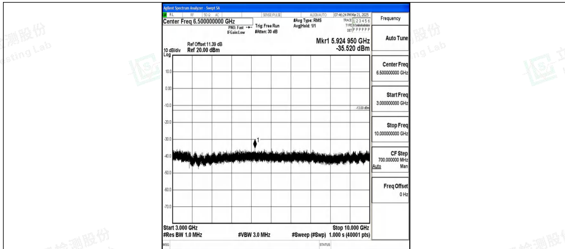
Band12_10MHz_QPSK_23060_1RB#0_3000~10000_3000~10000
