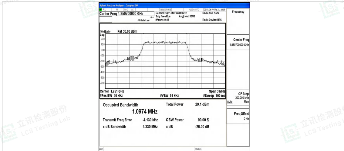
Band25-1.4MHz-QPSK-26047-6RB#0-PASS
