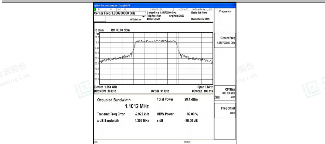
Band25-1.4MHz-16QAM-26047-6RB#0-PASS
