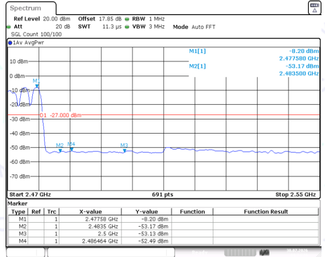
DH5-Ant1-Hop_2480-PASS
