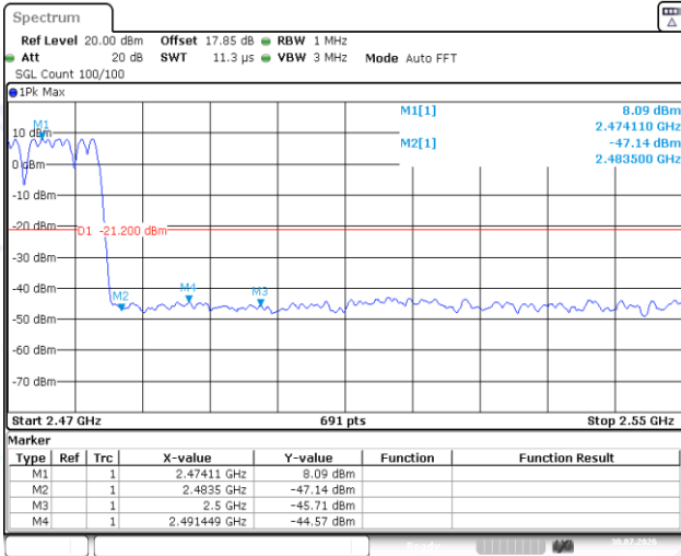
DH5-Ant1-Hop_2480-PASS
